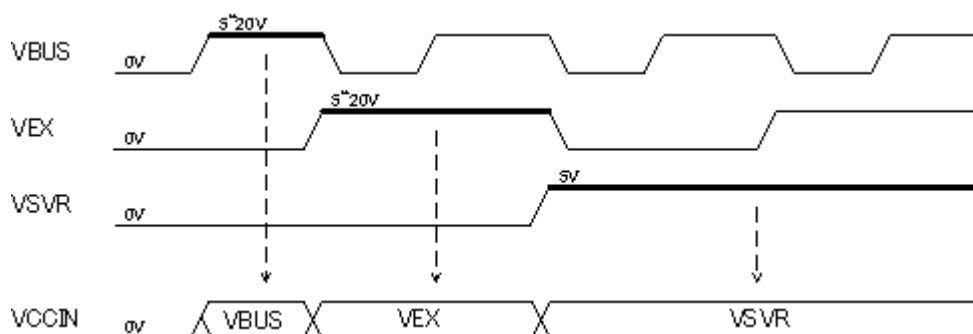
Figure 5-2. Power Supply Management Block Diagram and Timing Chart
