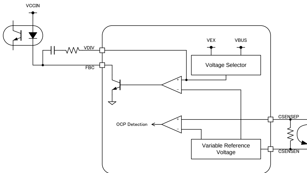
Figure 5-7. ACDC Bridge Block Diagram
