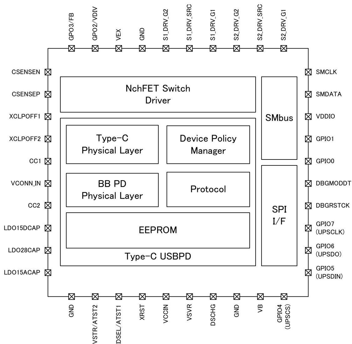
Figure 1-1. Block Diagram
