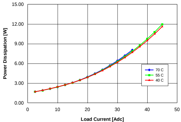
Fig. 1.2V.6: Power dissipation vs. load current and ambient temperature for converter mounted vertically with V_{in} = 48\text{ V} and air flowing from pin 3 to pin 1 at a rate of 200 LFM (1.0 m/s).
