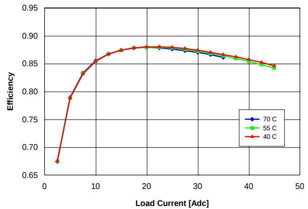
Fig. 1.5V.4: Efficiency vs. load current and ambient temperature for converter mounted vertically with V_{in} = 48\text{ V} and air flowing from pin 3 to pin 1 at a rate of 200 LFM (1.0 m/s).
