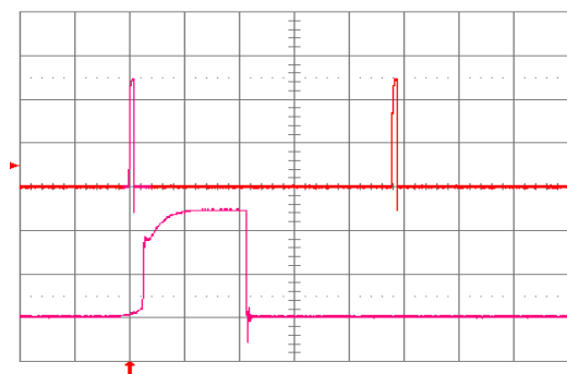
Fig. 2.5V.15: Load current (top trace, 20 A/div, 20 ms/div) into a 10 mΩ short circuit during restart, at V_{in} = 48 V. Bottom trace (20 A/div, 1 ms/div) is an expansion of the on-time portion of the top trace.
