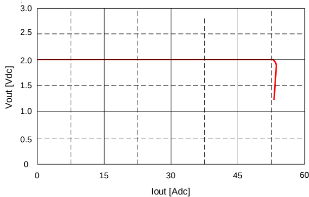
Fig. 2.0V.14: Output voltage vs. load current showing current limit point and converter shutdown point. Input voltage has almost no effect on current limit characteristic.
