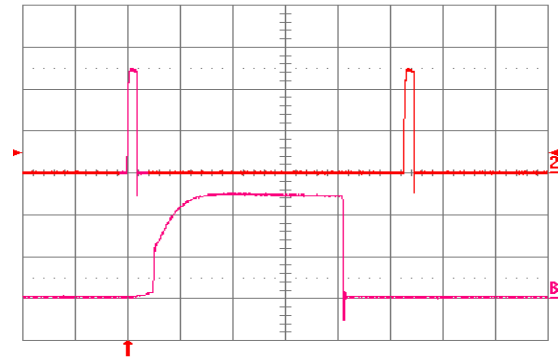
Fig. 1.8V.15: Load current (top trace, 20 A/div, 20 ms/div) into a 10 mΩ short circuit during restart, at V_{in} = 48 V. Bottom trace (20 A/div, 1 ms/div) is an expansion of the on-time portion of the top trace
