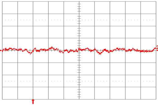
Fig. 2.5V.12: Input reflected ripple current, i_s (10 mA/div), measured through 10 \mu H at the source at full rated load current and V_{in} = 48 V. Refer to Fig. 2.5V.11 for test setup. Time scale: 1 \mu s/div.
