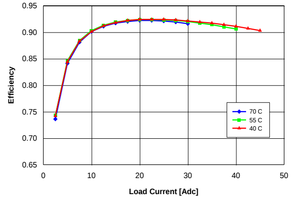
Fig. 3.3V.4: Efficiency vs. load current and ambient temperature for converter mounted vertically with V_{in} = 48\text{ V} and air flowing from pin 3 to pin 1 at a rate of 200 LFM (1.0 m/s).
