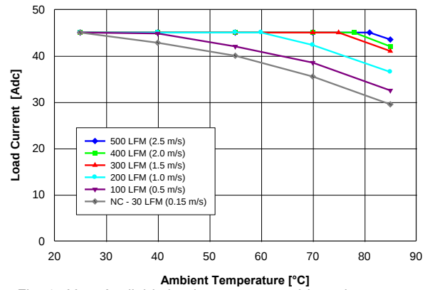
Fig. 1.0V.2: Available load current vs. ambient air temperature and airflow rates for QM48T45010 converter with B height pins mounted horizontally with V_{in} = 48\text{ V} , air flowing from pin 3 to pin 1, and MOSFET temperature \leq 120\text{ }^{\circ}\text{C} .
