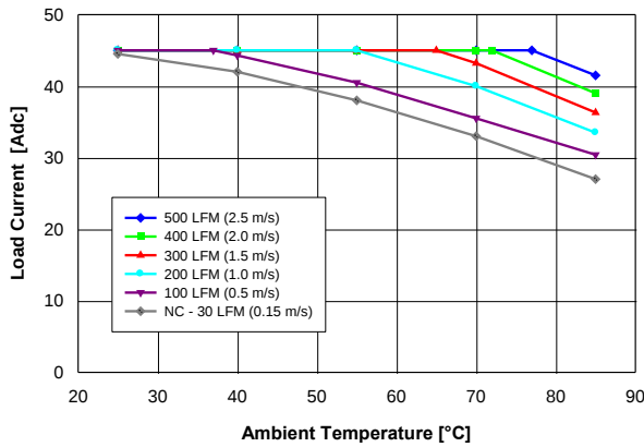
Fig. 1.5V.1: Available load current vs. ambient air temperature and airflow rates for QM48T45015 converter with B height pins mounted vertically with V_{in} = 48\text{ V} , air flowing from pin 3 to pin 1, and MOSFET temperature \leq 120\text{ }^{\circ}\text{C} . Note: NC – Natural convection
