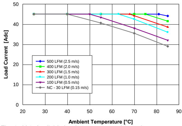
Fig. 1.0V.1: Available load current vs. ambient air temperature and airflow rates for QM48T45010 converter with B height pins mounted vertically with V_{in} = 48\text{ V} , air flowing from pin 3 to pin 1, and MOSFET temperature \leq 120\text{ }^{\circ}\text{C} . Note: NC – Natural convection
