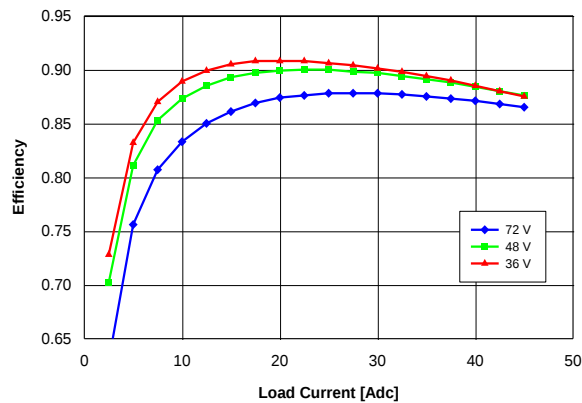
Fig. 2.0V.3: Efficiency vs. load current and input voltage for converter mounted vertically with air flowing from pin 3 to pin 1 at a rate of 300 LFM (1.5 m/s) and T_a = 25\text{ }^{\circ}\text{C} .
