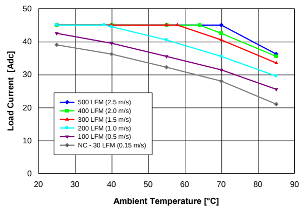
Fig. 2.5V.2: Available load current vs. ambient air temperature and airflow rates for QM48T45025 converter with B height pins mounted horizontally with V_{in} = 48\text{ V} , air flowing from pin 3 to pin 1, and MOSFET temperature \leq 120^\circ\text{C} .
