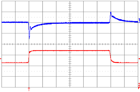
Fig. 3.3V.9: Output voltage response to load current step-change (22.5 A – 33.75 A – 22.5 A) at V_{in} = 48 V. Top trace: output voltage (100 mV/div.). Bottom trace: load current (10 A/div). Current slew rate: 1 A/ \mu s. C_o = 470 \mu F tantalum + 1 \mu F ceramic. Time scale: 0.2 ms/div.
