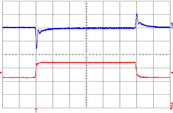
Fig. 1.2V.9: Output voltage response to load current step-change (22.5 A – 33.75 A – 22.5 A) at V_{in} = 48 V. Top trace: output voltage (20 mV/div.). Bottom trace: load current (10 A/div). Current slew rate: 1 A/ \mu s. C_o = 470 \mu F tantalum + 1 \mu F ceramic. Time scale: 0.2 ms/div.
