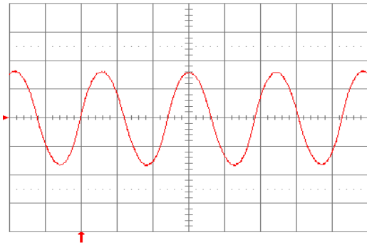
Fig. 2.5V.13: Input reflected ripple current, i_c (100 mA/div), measured at input terminals at full rated load current and V_{in} = 48 V. Refer to Fig. 2.5V.11 for test setup. Time scale: 1 \mu s/div.
