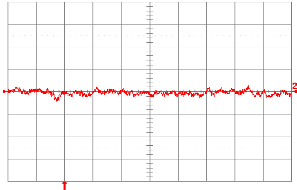
Fig. 1.0V.12: Input reflected ripple current, i_s (10 mA/div), measured through 10 \mu H at the source at full rated load current and V_{in} = 48 V. Refer to Fig. 1.0V.11 for test setup. Time scale: 1 \mu s/div.
