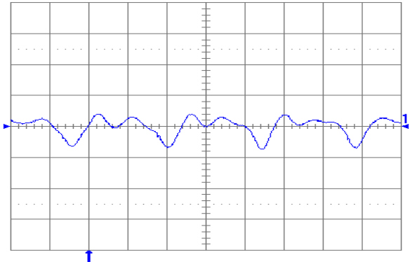
Fig. 1.2V.10: Output voltage ripple (20 mV/div.) at full rated load current into a resistive load with C_o = 10 \mu F tantalum + 1 \mu F ceramic and V_{in} = 48 V. Time scale: 1 \mu s/div.
