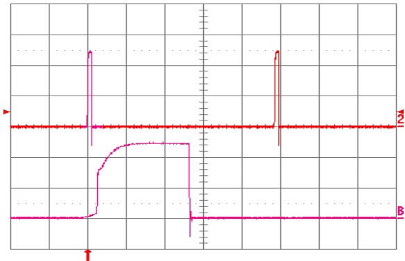
Fig. 2.0V.15: Load current (top trace, 20 A/div, 20 ms/div) into a 10\ \text{m}\Omega short circuit during restart, at V_{in} = 48\ \text{V} . Bottom trace (20 A/div, 1 ms/div) is an expansion of the on-time portion of the top trace.
