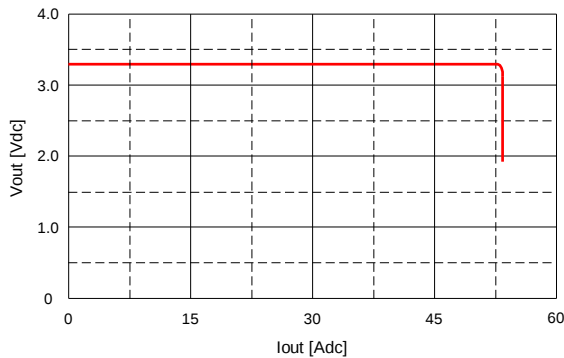
Fig. 3.3V.14: Output voltage vs. load current showing current limit point and converter shutdown point. Input voltage has almost no effect on current limit characteristic.
