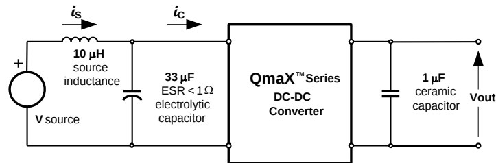
Fig. 1.0V.11: Test Setup for measuring input reflected ripple currents, i_c and i_s .
