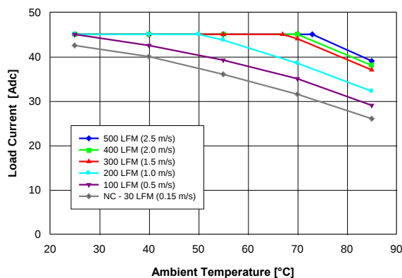
Fig. 1.8V.2: Available load current vs. ambient air temperature and airflow rates for QM48T45018 converter with B height pins mounted horizontally with V_{in} = 48\text{ V} , air flowing from pin 3 to pin 1, and MOSFET temperature \leq 120^\circ\text{C} .
