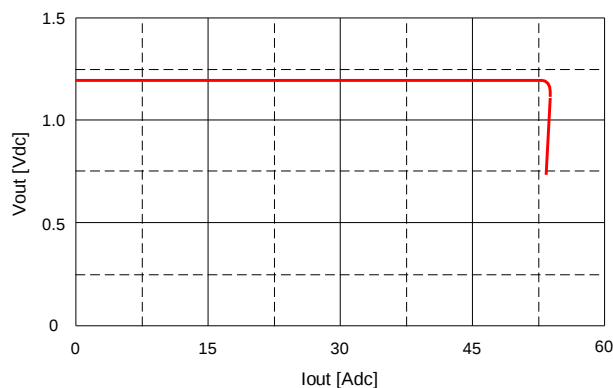
Fig. 1.2V.14: Output voltage vs. load current showing current limit point and converter shutdown point. Input voltage has almost no effect on current limit characteristic.
