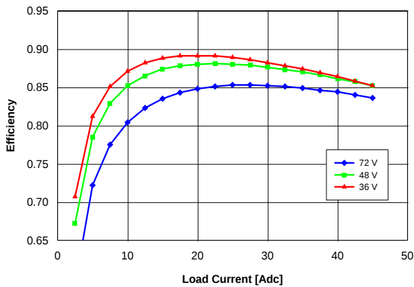
Fig. 1.5V.3: Efficiency vs. load current and input voltage for converter mounted vertically with air flowing from pin 3 to pin 1 at a rate of 300 LFM (1.5 m/s) and T_a = 25\text{ }^{\circ}\text{C} .
