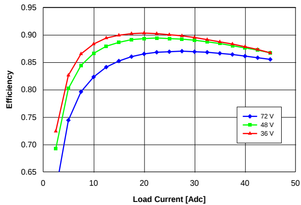
Fig. 1.8V.3: Efficiency vs. load current and input voltage for converter mounted vertically with air flowing from pin 3 to pin 1 at a rate of 300 LFM (1.5 m/s) and T_a = 25^\circ\text{C} .
