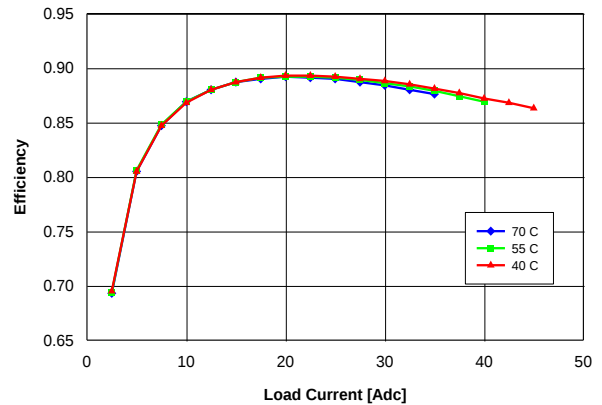
Fig. 1.8V.4: Efficiency vs. load current and ambient temperature for converter mounted vertically with V_{in} = 48\text{ V} and air flowing from pin 3 to pin 1 at a rate of 200 LFM (1.0 m/s).
