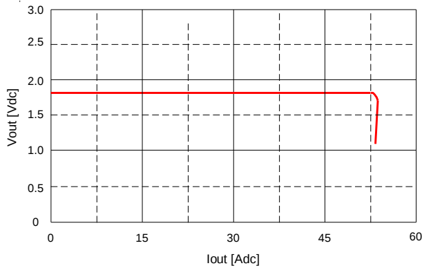
Fig. 1.8V.14: Output voltage vs. load current showing current limit point and converter shutdown point. Input voltage has almost no effect on current limit characteristic.
