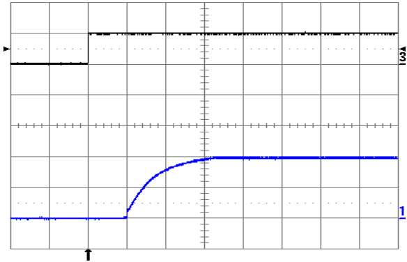
Fig. 2.0V.8: Turn-on transient at full rated load current (resistive) plus 40,000 \mu\text{F} at V_{in} = 48\text{ V} , triggered via ON/OFF pin. Top trace: ON/OFF signal (5 V/div.). Bottom trace: output voltage (1 V/div.). Time scale: 2 ms/div.
