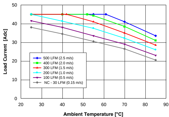
Fig. 3.3V.1: Available load current vs. ambient air temperature and airflow rates for QM48T45033 converter with B height pins mounted vertically with V_{in} = 48\text{ V} , air flowing from pin 3 to pin 1, and MOSFET temperature \leq 120^\circ\text{C} .
