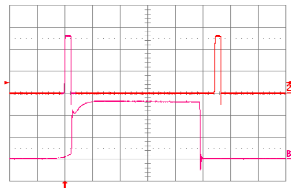
Fig. 1.2V.15: Load current (top trace, 20 A/div, 20 ms/div) into a 10 mΩ short circuit during restart, at V_{in} = 48 V. Bottom trace (20 A/div, 1 ms/div) is an expansion of the on-time portion of the top trace.
