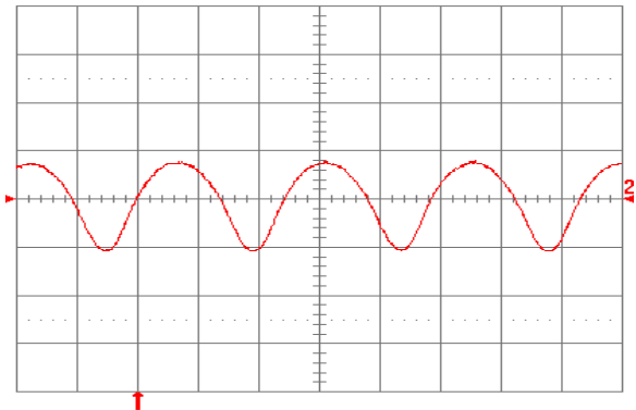
Fig. 1.2V.13: Input reflected ripple current, i_c (100 mA/div), measured at input terminals at full rated load current and V_{in} = 48 V. Refer to Fig. 1.2V.11 for test setup. Time scale: 1 \mu s/div.
