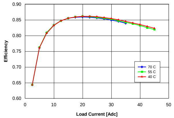
Fig. 1.2V.4: Efficiency vs. load current and ambient temperature for converter mounted vertically with V_{in} = 48\text{ V} and air flowing from pin 3 to pin 1 at a rate of 200 LFM (1.0 m/s).
