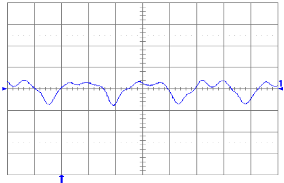
Fig. 2.0V.10: Output voltage ripple (20 mV/div.) at full rated load current into a resistive load with C_o = 10\text{ }\mu\text{F} tantalum + 1 \mu\text{F} ceramic and V_{in} = 48\text{ V} . Time scale: 1 \mu\text{s} /div.
