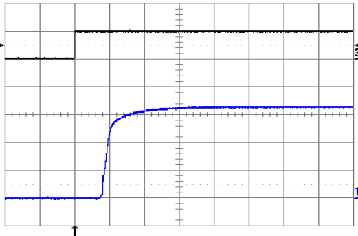
Fig. 3.3V.7: Turn-on transient at full rated load current (resistive) with no output capacitor at V_{in} = 48\text{ V} , triggered via ON/OFF pin. Top trace: ON/OFF signal (5 V/div.). Bottom trace: output voltage (1 V/div.). Time scale: 2 ms/div.
