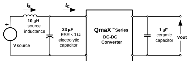
Fig. 2.0V.11: Test Setup for measuring input reflected ripple currents, i_c and i_s .
