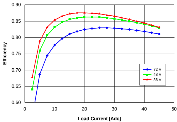
Fig. 1.2V.3: Efficiency vs. load current and input voltage for converter mounted vertically with air flowing from pin 3 to pin 1 at a rate of 300 LFM (1.5 m/s) and T_a = 25^\circ\text{C} .
