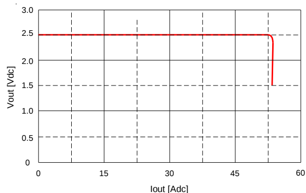
Fig. 2.5V.14: Output voltage vs. load current showing current limit point and converter shutdown point. Input voltage has almost no effect on current limit characteristic.
