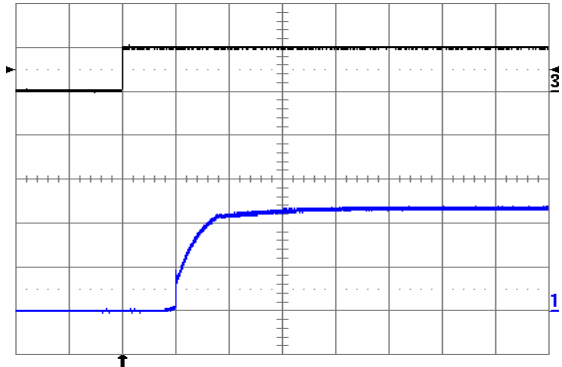
Fig. 1.2V.8: Turn-on transient at full rated load current (resistive) plus 40,000 \mu\text{F} at V_{in} = 48\text{ V} , triggered via ON/OFF pin. Top trace: ON/OFF signal (5 V/div.). Bottom trace: output voltage (1 V/div.). Time scale: 2 ms/div.
