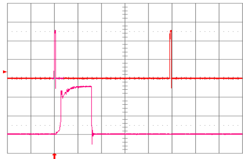
Fig. 3.3V.15: Load current (top trace, 20 A/div, (20 ms/div) into a 10 m \Omega short circuit during restart, at V_{in} = 48 V. Bottom trace (20 A/div, 1 ms/div) is an expansion of the on-time portion of the top trace.
