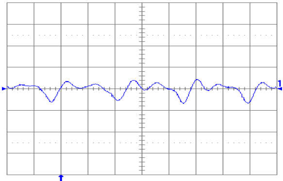
Fig. 1.0V.10: Output voltage ripple (20 mV/div.) at full rated load current into a resistive load with C_o = 10\text{ }\mu\text{F} tantalum + 1 \mu\text{F} ceramic and V_{in} = 48\text{ V} . Time scale: 1 \mu\text{s} /div.
