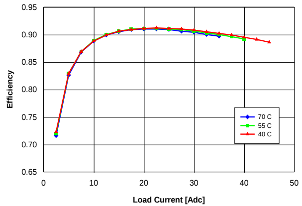
Fig. 2.5V.4: Efficiency vs. load current and ambient temperature for converter mounted vertically with V_{in} = 48\text{ V} and air flowing from pin 3 to pin 1 at a rate of 200 LFM (1.0 m/s).
