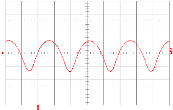
Fig. 1.0V.13: Input reflected ripple current, i_c (100 mA/div), measured at input terminals at full rated load current and V_{in} = 48 V. Refer to Fig. 1.0V.11 for test setup. Time scale: 1 \mu s/div.
