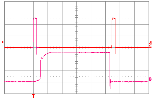
Fig. 1.0V.15: Load current (top trace, 20 A/div, 20 ms/div) into a 10 m \Omega short circuit during restart, at V_{in} = 48 V. Bottom trace (20 A/div, 1 ms/div) is an expansion of the on-time portion of the top trace.
