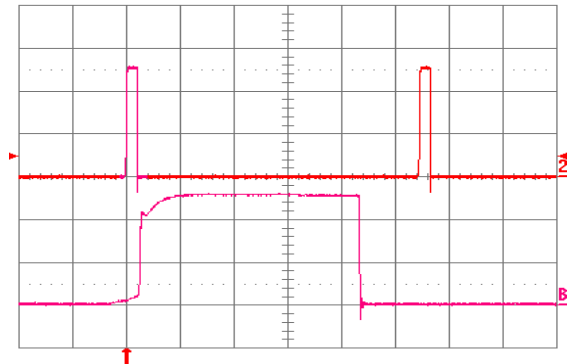
Fig. 1.5V.15: Load current (top trace, 20 A/div, 20 ms/div) into a 10\ \text{m}\Omega short circuit during restart, at V_{in} = 48\ \text{V} . Bottom trace (20 A/div, 1 ms/div) is an expansion of the on-time portion of the top trace.
