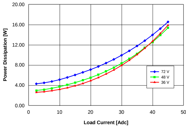
Fig. 2.5V.5: Power dissipation vs. load current and input voltage for converter mounted vertically with air flowing from pin 3 to pin 1 at a rate of 300 LFM (1.5 m/s) and T_a = 25^\circ\text{C} .
