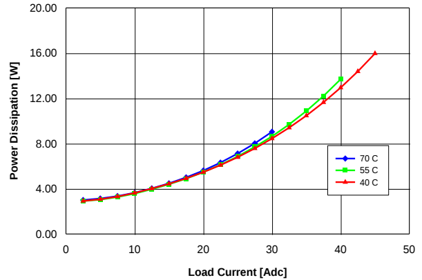
Fig. 3.3V.6: Power dissipation vs. load current and ambient temperature for converter mounted vertically with V_{in} = 48\text{ V} and air flowing from pin 3 to pin 1 at a rate of 200 LFM (1.0 m/s).
