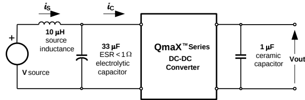
Fig. 2.5V.11: Test Setup for measuring input reflected ripple currents, i_c and i_s .
