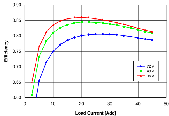
Fig. 1.0V.3: Efficiency vs. load current and input voltage for converter mounted vertically with air flowing from pin 3 to pin 1 at a rate of 300 LFM (1.5 m/s) and T_a = 25\text{ }^{\circ}\text{C} .
