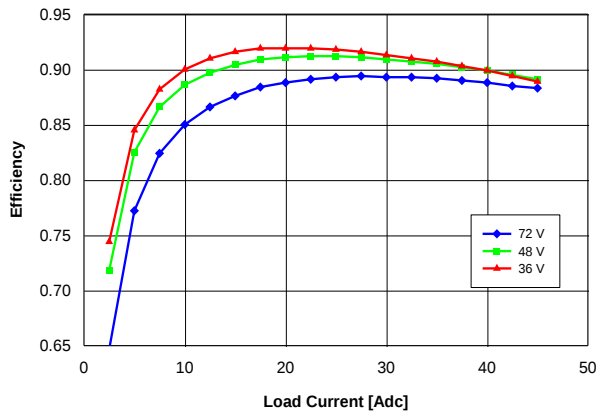
Fig. 2.5V.3: Efficiency vs. load current and input voltage for converter mounted vertically with air flowing from pin 3 to pin 1 at a rate of 300 LFM (1.5 m/s) and T_a = 25^\circ\text{C} .
