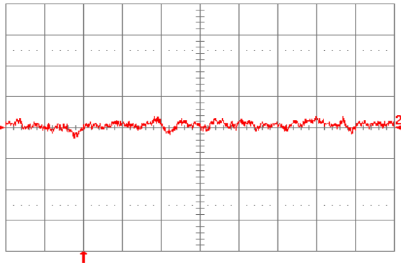
Fig. 1.2V.12: Input reflected ripple current, i_s (10 mA/div), measured through 10 \mu H at the source at full rated load current and V_{in} = 48 V. Refer to Fig. 1.2V.11 for test setup. Time scale: 1 \mu s/div.
