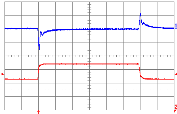
Fig. 1.0V.9: Output voltage response to load current step-change (22.5 A – 33.75 A – 22.5 A) at V_{in} = 48\text{ V} . Top trace: output voltage (100 mV/div.). Bottom trace: load current (10 A/div.). Current slew rate: 1 A/ \mu\text{s} . C_o = 470\text{ }\mu\text{F} tantalum + 1 \mu\text{F} ceramic. Time scale: 0.2 ms/div.
