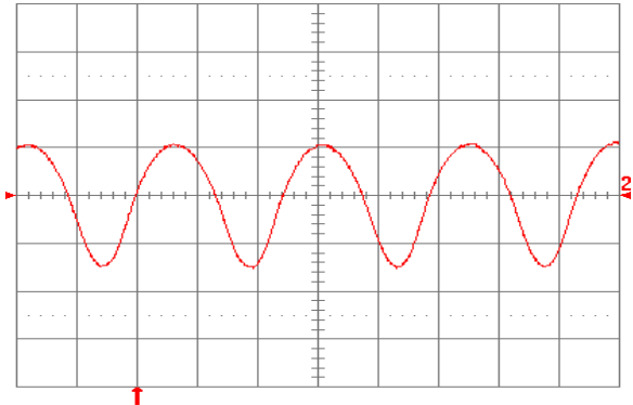
Fig. 1.5V.13: Input reflected ripple current, i_c (100 mA/div), measured at input terminals at full rated load current and V_{in} = 48\ \text{V} . Refer to Fig. 1.5V.11 for test setup. Time scale: 1\ \mu\text{s}/\text{div} .
