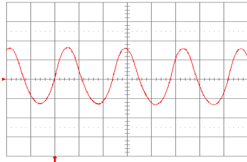
Fig. 3.3V.13: Input reflected ripple current, i_c (100 mA/div), measured at input terminals at full rated load current and V_{in} = 48 V. Refer to Fig. 3.3V.11 for test setup. Time scale: 1 \mu s/div.
