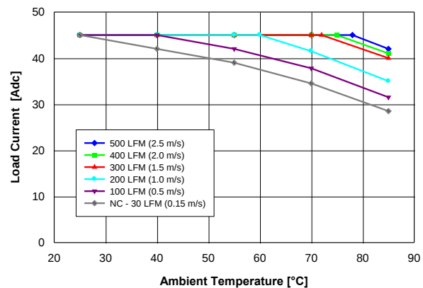
Fig. 1.2V.2: Available load current vs. ambient air temperature and airflow rates for QM48T45012 converter with B height pins mounted horizontally with V_{in} = 48\text{ V} , air flowing from pin 3 to pin 1, and MOSFET temperature \leq 120^\circ\text{C} .
