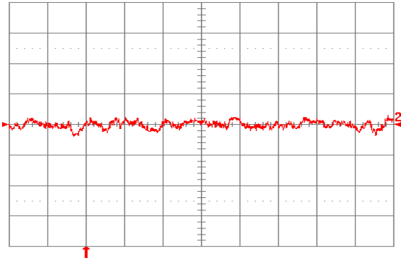
Fig. 1.5V.12: Input reflected ripple current, i_s (10 mA/div), measured through 10\ \mu\text{H} at the source at full rated load current and V_{in} = 48\ \text{V} . Refer to Fig. 1.5V.11 for test setup. Time scale: 1\ \mu\text{s}/\text{div} .
