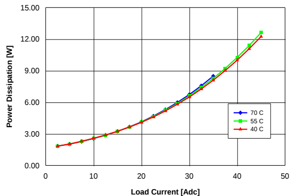
Fig. 1.5V.6: Power dissipation vs. load current and ambient temperature for converter mounted vertically with V_{in} = 48\text{ V} and air flowing from pin 3 to pin 1 at a rate of 200 LFM (1.0 m/s).
