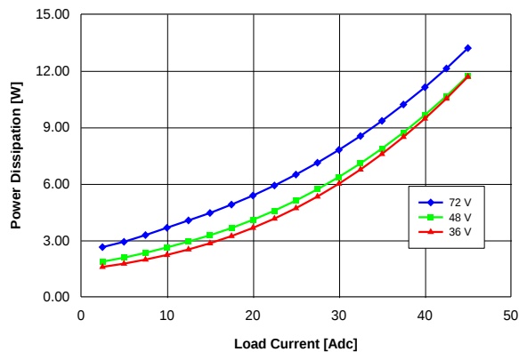
Fig. 1.5V.5: Power dissipation vs. load current and input voltage for converter mounted vertically with air flowing from pin 3 to pin 1 at a rate of 300 LFM (1.5 m/s) and T_a = 25\text{ }^{\circ}\text{C} .
