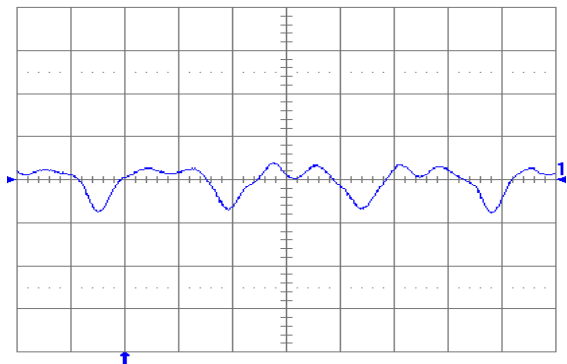
Fig. 1.5V.10: Output voltage ripple (20 mV/div.) at full rated load current into a resistive load with C_o = 10 \mu F tantalum + 1 \mu F ceramic and V_{in} = 48 V. Time scale: 1 \mu s/div.
