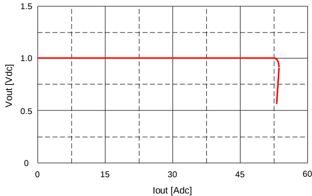
Fig. 1.0V.14: Output voltage vs. load current showing current limit point and converter shutdown point. Input voltage has almost no effect on current limit characteristic.
