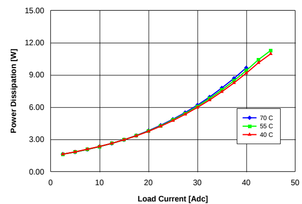
Fig. 1.0V.6: Power dissipation vs. load current and ambient temperature for converter mounted vertically with V_{in} = 48\text{ V} and air flowing from pin 3 to pin 1 at a rate of 200 LFM (1.0 m/s).
