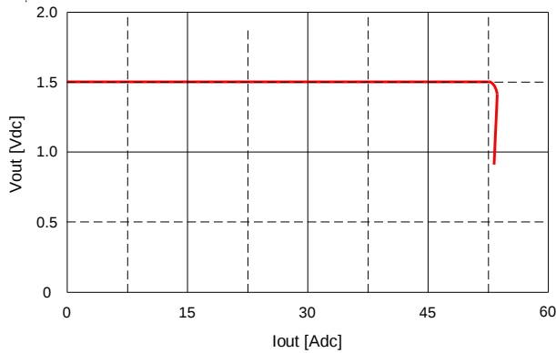
Fig. 1.5V.14: Output voltage vs. load current showing current limit point and converter shutdown point. Input voltage has almost no effect on current limit characteristic.
