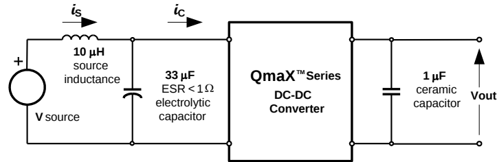
Fig. 1.8V.11: Test Setup for measuring input reflected ripple currents, i_c and i_s .
