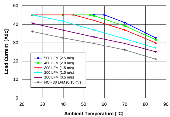
Fig. 3.3V.2: Available load current vs. ambient air temperature and airflow rates for QM48T45033 converter with B height pins mounted horizontally with V_{in} = 48\text{ V} , air flowing from pin 3 to pin 1, and MOSFET temperature \leq 120^\circ\text{C} .
