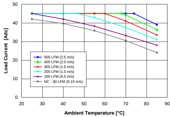
Fig. 2.0V.1: Available load current vs. ambient air temperature and airflow rates for QM48T45020 converter with B height pins mounted vertically with V_{in} = 48\text{ V} , air flowing from pin 3 to pin 1, and MOSFET temperature \leq 120\text{ }^{\circ}\text{C} . Note: NC – Natural convection
