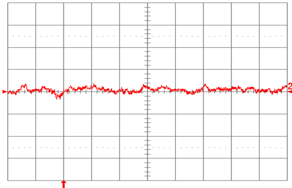
Fig. 1.8V.12: Input reflected ripple current, i_s (10 mA/div), measured through 10 \mu H at the source at full rated load current and V_{in} = 48 V. Refer to Fig. 1.8V.11 for test setup. Time scale: 1 \mu s/div.
