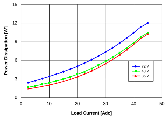
Fig. 1.0V.5: Power dissipation vs. load current and input voltage for converter mounted vertically with air flowing from pin 3 to pin 1 at a rate of 300 LFM (1.5 m/s) and T_a = 25\text{ }^{\circ}\text{C} .
