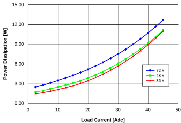
Fig. 1.2V.5: Power dissipation vs. load current and input voltage for converter mounted vertically with air flowing from pin 3 to pin 1 at a rate of 300 LFM (1.5 m/s) and T_a = 25^\circ\text{C} .
