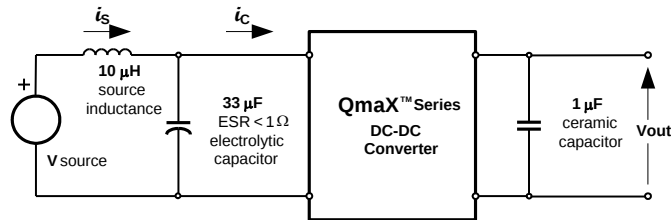
Fig. 1.2V.11: Test Setup for measuring input reflected ripple currents, i_c and i_s .
