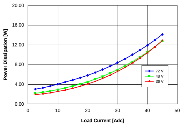
Fig. 2.0V.5: Power dissipation vs. load current and input voltage for converter mounted vertically with air flowing from pin 3 to pin 1 at a rate of 300 LFM (1.5 m/s) and T_a = 25\text{ }^{\circ}\text{C} .
