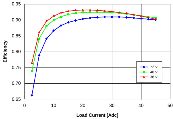
Fig. 3.3V.3: Efficiency vs. load current and input voltage for converter mounted vertically with air flowing from pin 3 to pin 1 at a rate of 300 LFM (1.5 m/s) and T_a = 25^\circ\text{C} .
