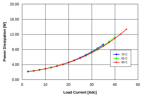
Fig. 2.0V.6: Power dissipation vs. load current and ambient temperature for converter mounted vertically with V_{in} = 48\text{ V} and air flowing from pin 3 to pin 1 at a rate of 200 LFM (1.0 m/s).
