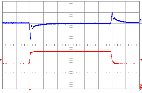
Fig. 2.0V.9: Output voltage response to load current step-change (22.5 A – 33.75 A – 22.5 A) at V_{in} = 48\text{ V} . Top trace: output voltage (100 mV/div.). Bottom trace: load current (10 A/div.). Current slew rate: 1 A/ \mu\text{s} . C_o = 470\text{ }\mu\text{F} tantalum + 1 \mu\text{F} ceramic. Time scale: 0.2 ms/div.
