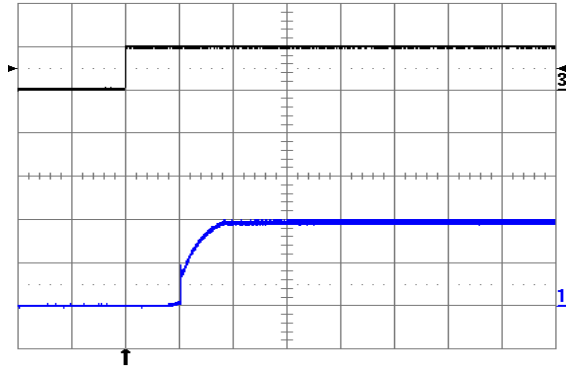
Fig. 1.0V.8: Turn-on transient at full rated load current (resistive) plus 40,000 \mu\text{F} at V_{in} = 48\text{ V} , triggered via ON/OFF pin. Top trace: ON/OFF signal (5 V/div.). Bottom trace: output voltage (1 V/div.). Time scale: 2 ms/div.
