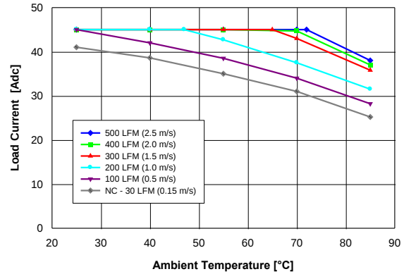
Fig. 2.0V.2: Available load current vs. ambient air temperature and airflow rates for QM48T45020 converter with B height pins mounted horizontally with V_{in} = 48\text{ V} , air flowing from pin 3 to pin 1, and MOSFET temperature \leq 120\text{ }^{\circ}\text{C} .
