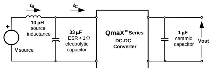
Fig. 1.5V.11: Test Setup for measuring input reflected ripple currents, i_c and i_s .
