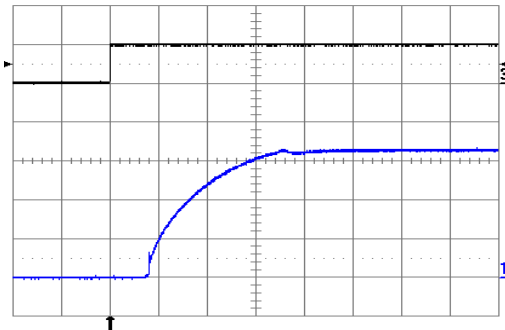
Fig. 3.3V.8: Turn-on transient at full rated load current (resistive) plus 40,000 \mu\text{F} at V_{in} = 48\text{ V} , triggered via ON/OFF pin. Top trace: ON/OFF signal (5 V/div.). Bottom trace: output voltage (1 V/div.). Time scale: 2 ms/div.
