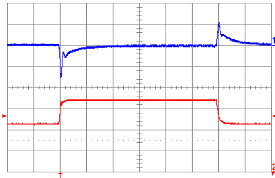
Fig. 1.5V.9: Output voltage response to load current step-change (22.5 A – 33.75 A – 22.5 A) at V_{in} = 48 V. Top trace: output voltage (100 mV/div.). Bottom trace: load current (10 A/div.). Current slew rate: 1 A/ \mu s. C_o = 470 \mu F tantalum + 1 \mu F ceramic. Time scale: 0.2 ms/div.
