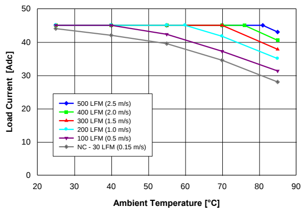
Fig. 1.2V.1: Available load current vs. ambient air temperature and airflow rates for QM48T45012 converter with B height pins mounted vertically with V_{in} = 48\text{ V} , air flowing from pin 3 to pin 1, and MOSFET temperature \leq 120^\circ\text{C} . Note: NC – Natural convection
