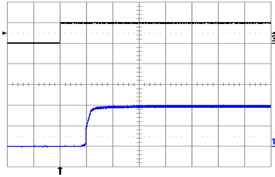
Fig. 1.0V.7: Turn-on transient at full rated load current (resistive) with no output capacitor at V_{in} = 48\text{ V} , triggered via ON/OFF pin. Top trace: ON/OFF signal (5 V/div.). Bottom trace: output voltage (1 V/div.). Time scale: 2 ms/div.
