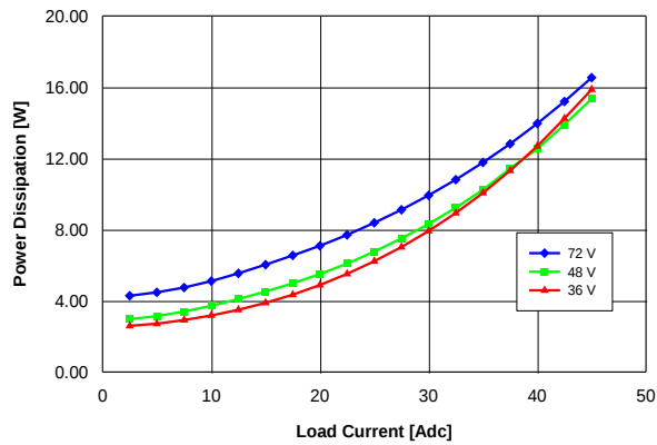
Fig. 3.3V.5: Power dissipation vs. load current and input voltage for converter mounted vertically with air flowing from pin 3 to pin 1 at a rate of 300 LFM (1.5 m/s) and T_a = 25^\circ\text{C} .
