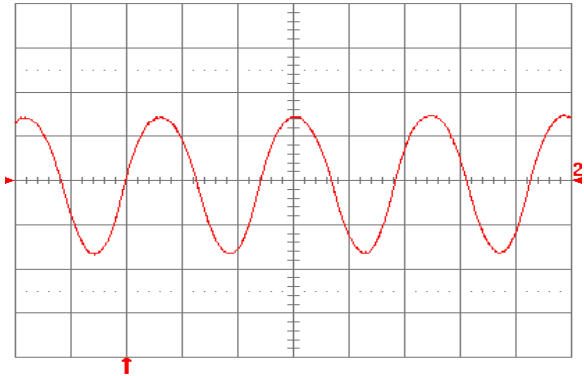
Fig. 2.0V.13: Input reflected ripple current, i_c (100 mA/div), measured at input terminals at full rated load current and V_{in} = 48\ \text{V} . Refer to Fig. 2.0V.11 for test setup. Time scale: 1\ \mu\text{s}/\text{div} .
