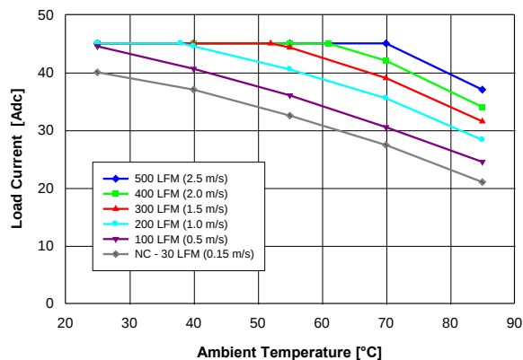
Fig. 2.5V.1: Available load current vs. ambient air temperature and airflow rates for QM48T45025 converter with B height pins mounted vertically with V_{in} = 48\text{ V} , air flowing from pin 3 to pin 1, and MOSFET temp. \leq 120^\circ\text{C} . Note: NC – Natural convection
