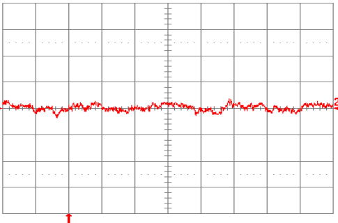
Fig. 3.3V.12: Input reflected ripple current, i_s (10 mA/div), measured through 10 \mu H at the source at full rated load current and V_{in} = 48 V. Refer to Fig. 3.3V.11 for test setup. Time scale: 1 \mu s/div.
