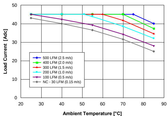
Fig. 1.8V.1: Available load current vs. ambient air temperature and airflow rates for QM48T45018 converter with B height pins mounted vertically with V_{in} = 48\text{ V} , air flowing from pin 3 to pin 1, and MOSFET temperature \leq 120^\circ\text{C} .
