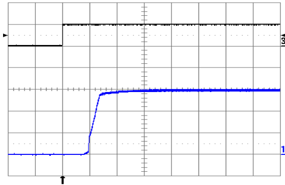
Fig. 1.5V.7: Turn-on transient at full rated load current (resistive) with no output capacitor at V_{in} = 48 V, triggered via ON/OFF pin. Top trace: ON/OFF signal (5 V/div.). Bottom trace: output voltage (1 V/div.) Time scale: 2 ms/div.
