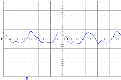
Fig. 3.3V.10: Output voltage ripple (20 mV/div.) at full rated load current into a resistive load with C_o = 10 \mu F tantalum + 1 \mu F ceramic and V_{in} = 48 V. Time scale: 1 \mu s/div.
