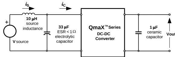
Fig. 3.3V.11: Test Setup for measuring input reflected ripple currents, i_c and i_s .
