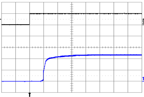
Fig. 1.2V.7: Turn-on transient at full rated load current (resistive) with no output capacitor at V_{in} = 48\text{ V} , triggered via ON/OFF pin. Top trace: ON/OFF signal (5 V/div.). Bottom trace: output voltage (1 V/div.). Time scale: 2 ms/div.
