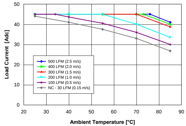
Fig. 1.5V.2: Available load current vs. ambient air temperature and airflow rates for QM48T45015 converter with B height pins mounted horizontally with V_{in} = 48\text{ V} , air flowing from pin 3 to pin 1, and MOSFET temperature \leq 120\text{ }^{\circ}\text{C} .
