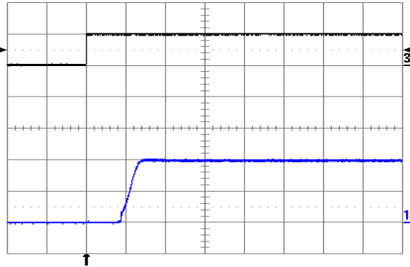
Fig. 2.0V.7: Turn-on transient at full rated load current (resistive) with no output capacitor at V_{in} = 48\text{ V} , triggered via ON/OFF pin. Top trace: ON/OFF signal (5 V/div.). Bottom trace: output voltage (1 V/div.) Time scale: 2 ms/div.
