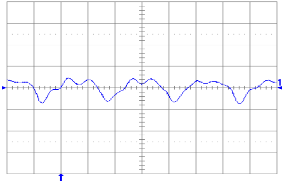
Fig. 1.8V.10: Output voltage ripple (20 mV/div.) at full rated load current into a resistive load with C_o = 10 \mu F tantalum + 1 \mu F ceramic and V_{in} = 48 V. Time scale: 1 \mu s/div.
