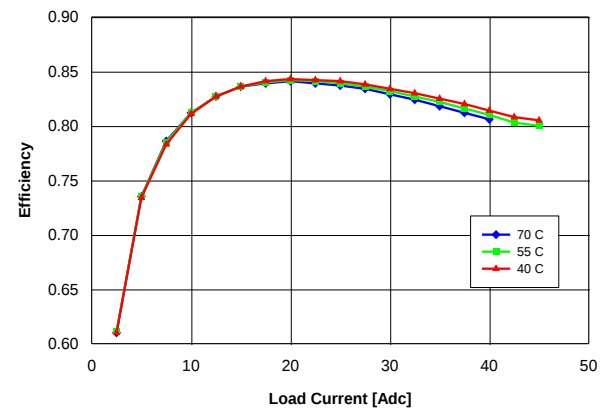
Fig. 1.0V.4: Efficiency vs. load current and ambient temperature for converter mounted vertically with V_{in} = 48\text{ V} and air flowing from pin 3 to pin 1 at a rate of 200 LFM (1.0 m/s).
