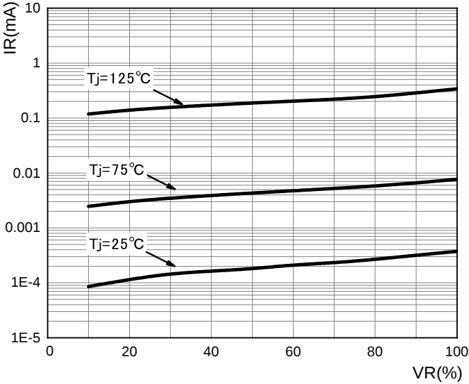
FIG.10: TYPICAL REVERSE CHARACTERISTICS
