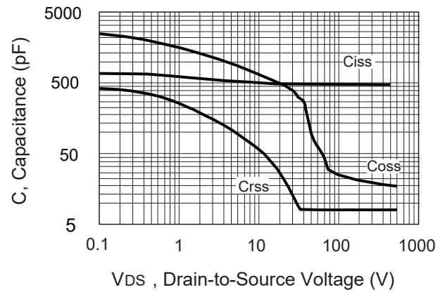
Capacitance Characteristics
