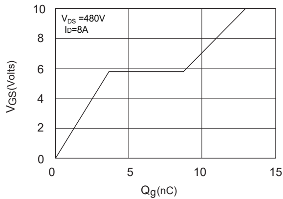
Gate-Charge Characteristics
