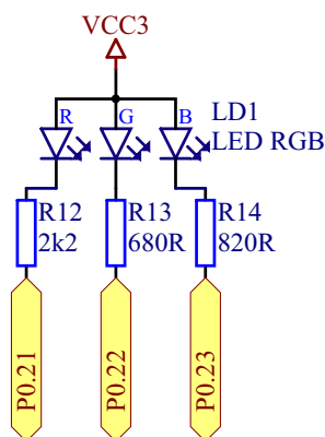
Figure 11 LED configuration
