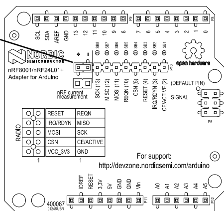
Figure 7 nRF current measurement jumper
