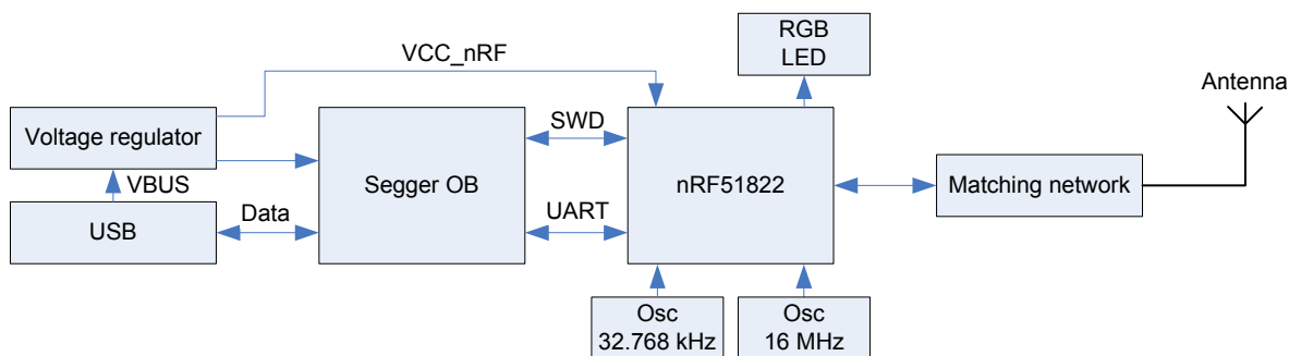
Figure 10 PCA10000 block diagram
