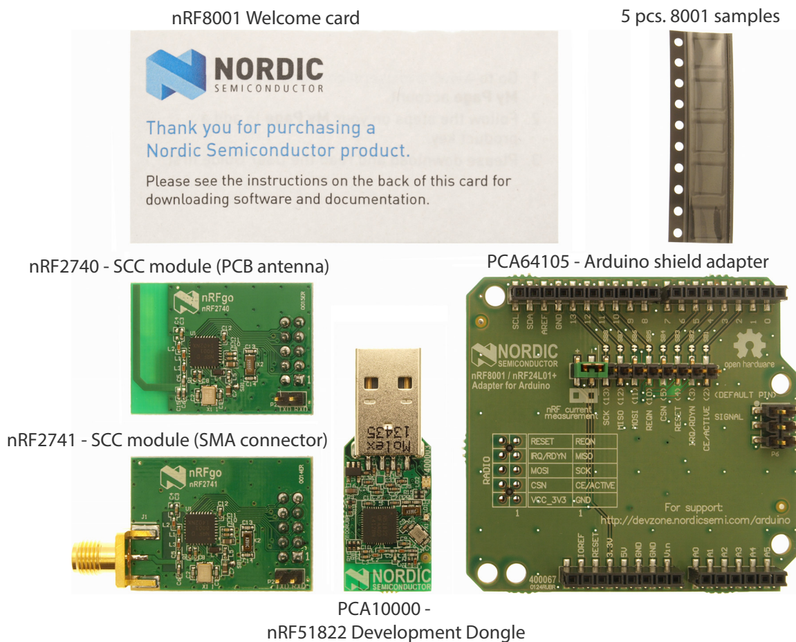
Figure 1 Hardware components
