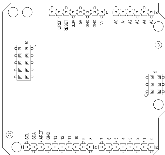
Figure 6 Arduino shield adapter, bottom side
