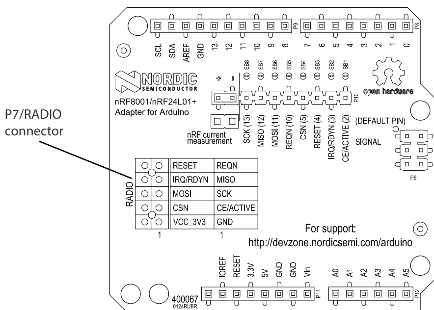
Figure 5 Arduino shield adapter, top side
