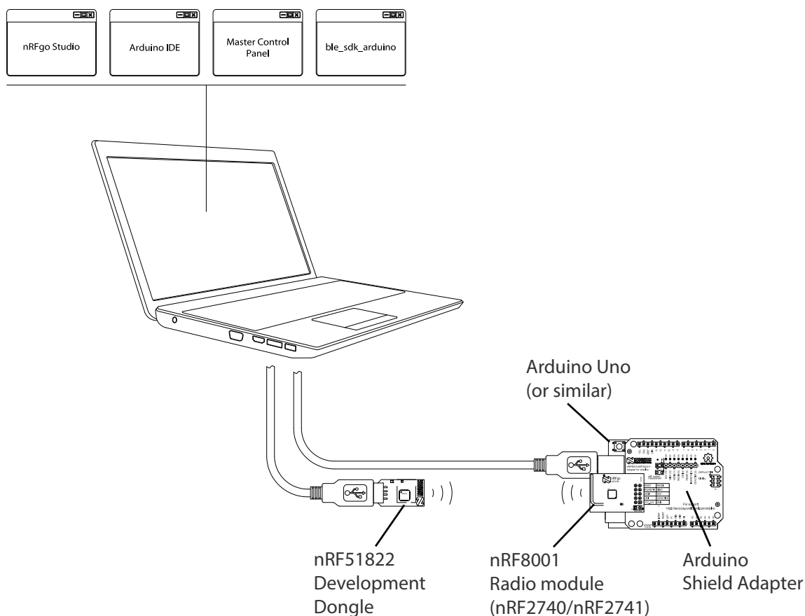
Figure 2 Typical setup
