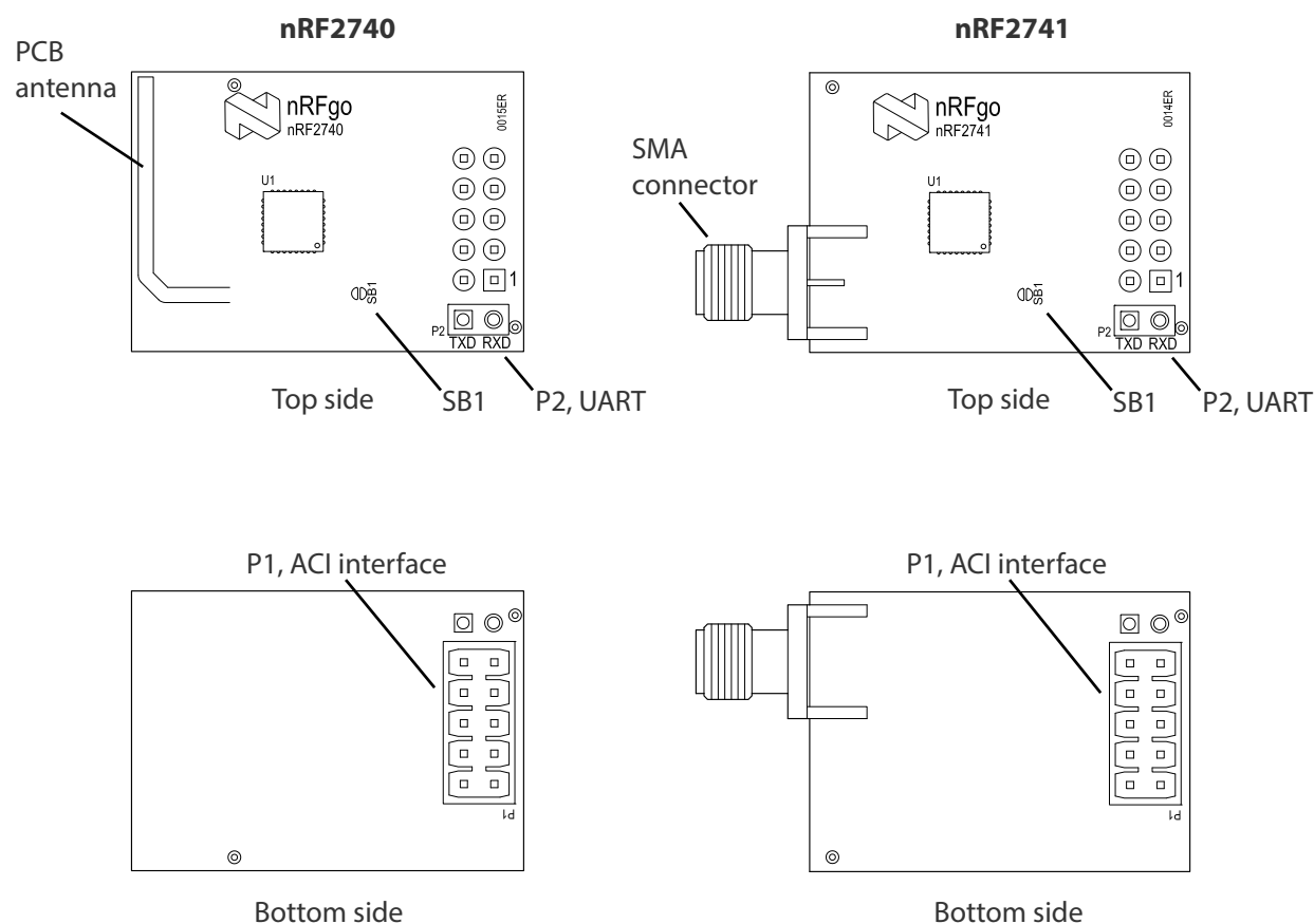
Figure 4 nRF2740 and nRF2741 radio modules
