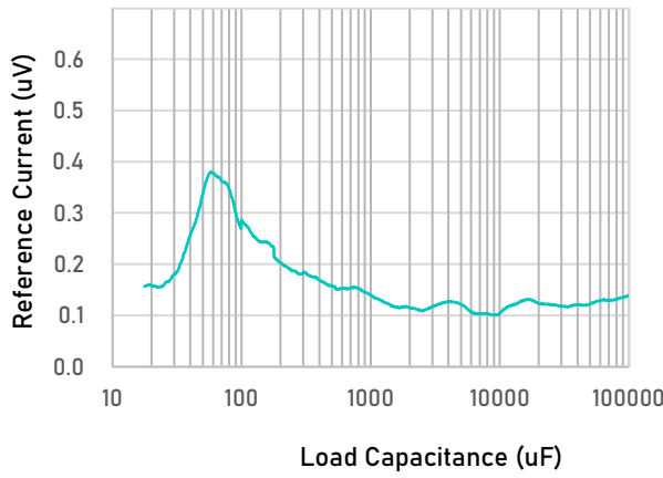
Stability Boundary Conditions for All Devices
