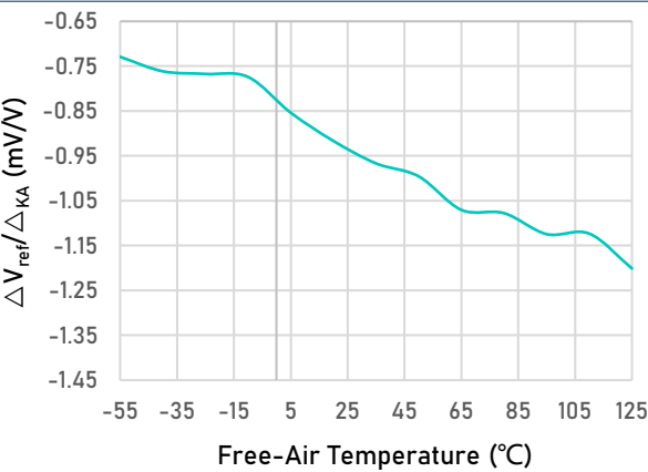
Ratio of Delta Reference Voltage to Delta Cathode vs Free-Air Temperature
