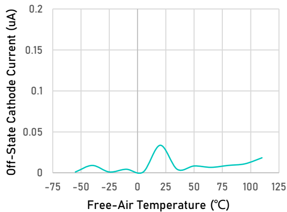
Off-State Cathode Current vs Free-Air Temperature
