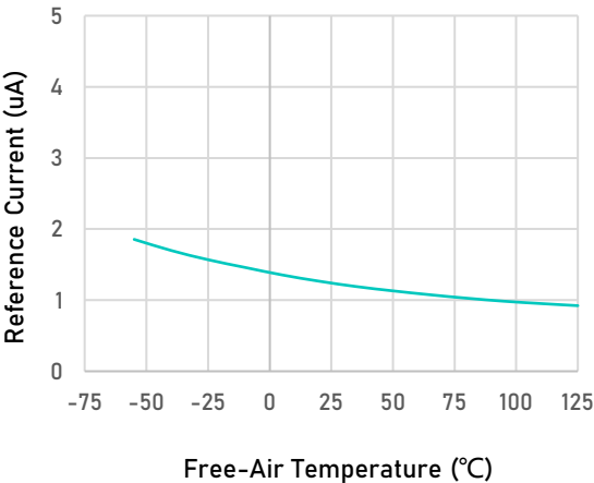
Reference Current vs Free-Air Temperature
