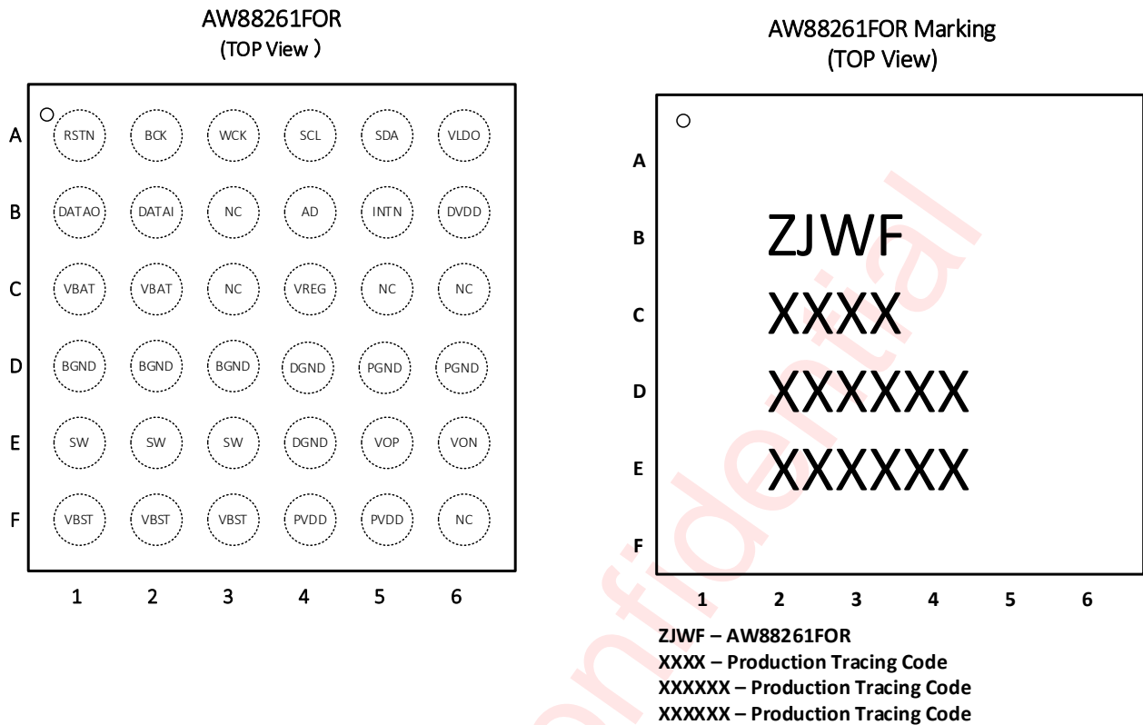
Figure 1 AW88261FOR pin diagram top view and device marking
