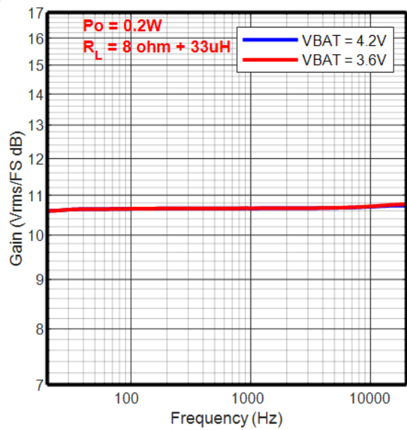
RECEIVER GAIN VS. FREQUENCY
