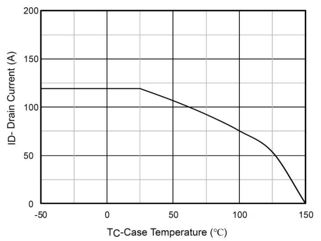
Current De-rating
