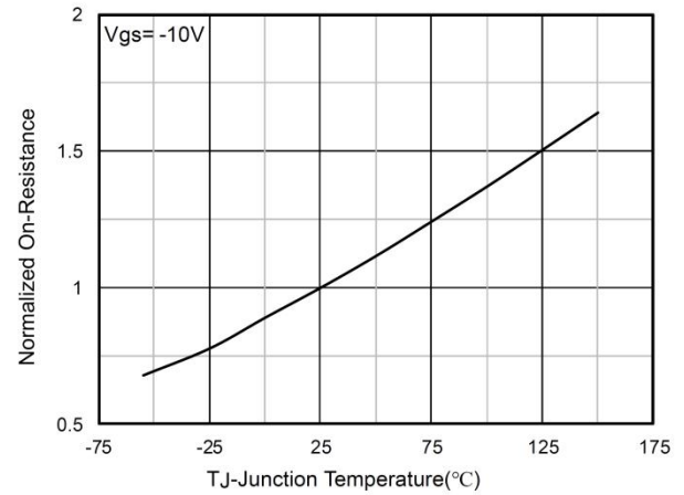
Rdson-Junction Temperature
