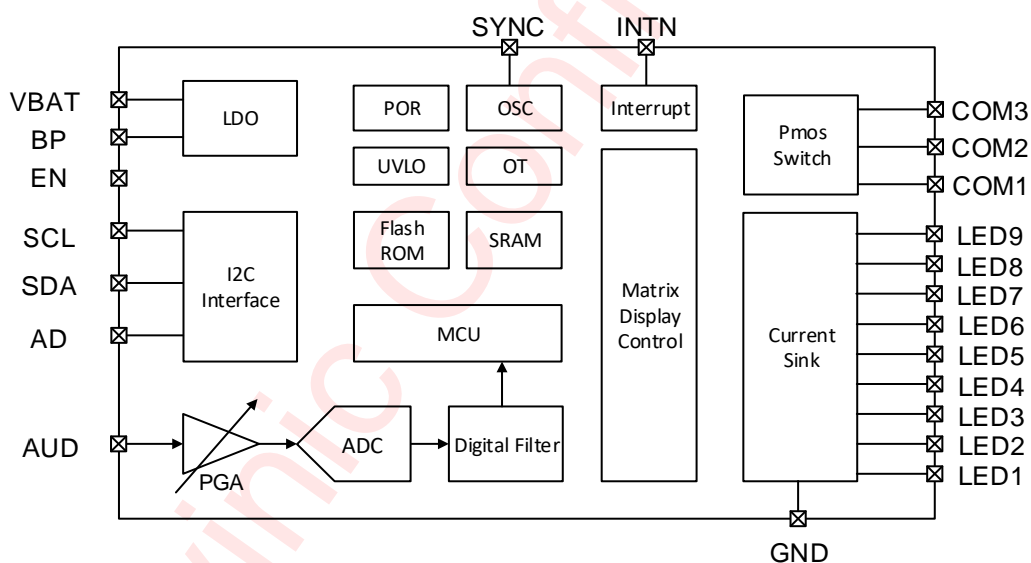
Figure 2 Function Block
