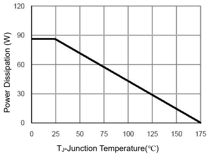
Figure 9 Power De-rating
