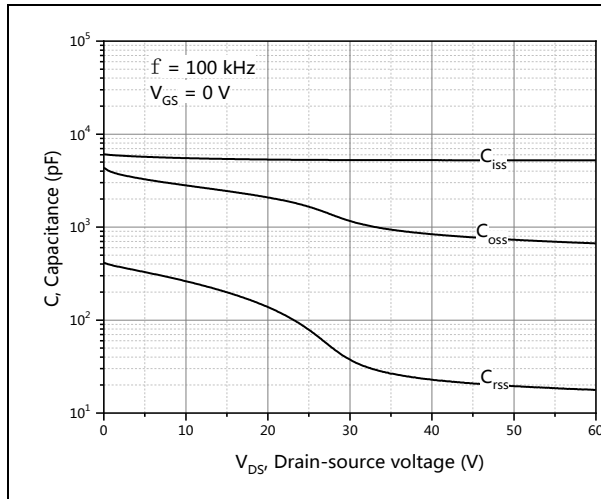
Figure 3, Typ. capacitances
