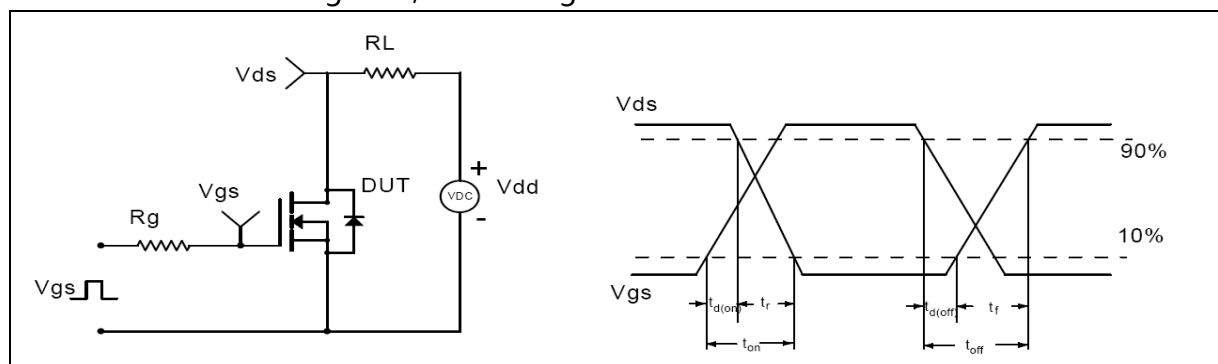
Figure 2, Switching time test circuit &amp; waveforms
