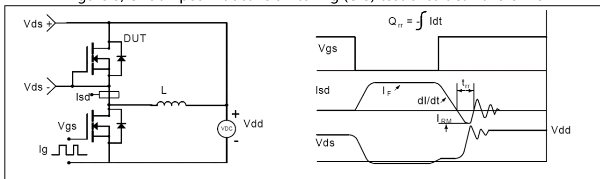
Figure 4, Diode reverse recovery test circuit &amp; waveforms
