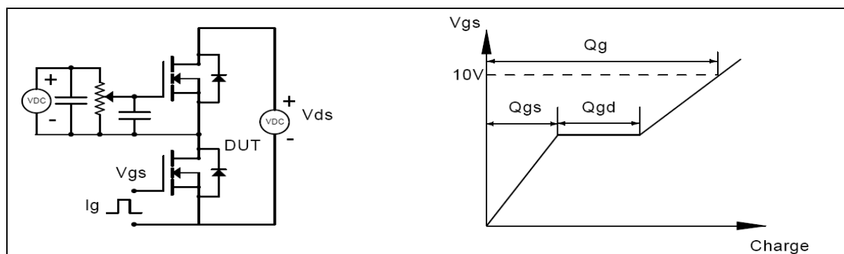
Figure 1, Gate charge test circuit &amp; waveform
