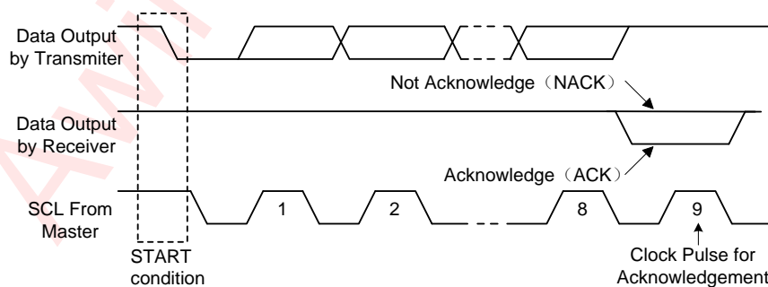
Figure 9 I 2 C ACK Timing
