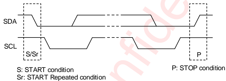
Figure 8 I 2 C Start/Stop Condition Timing
