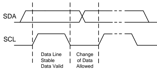
Figure 7 Data Validation Diagram
