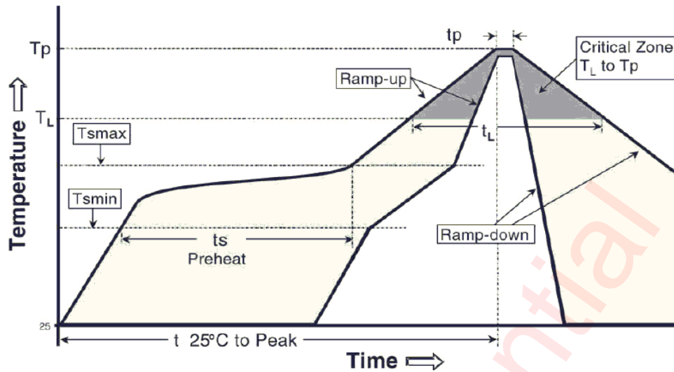
Reflow profile
