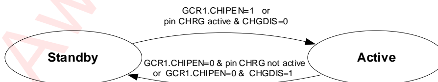
Figure 6 AW2033 Operating Modes Transition
