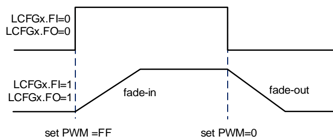
Figure 13 Manual Control Mode
