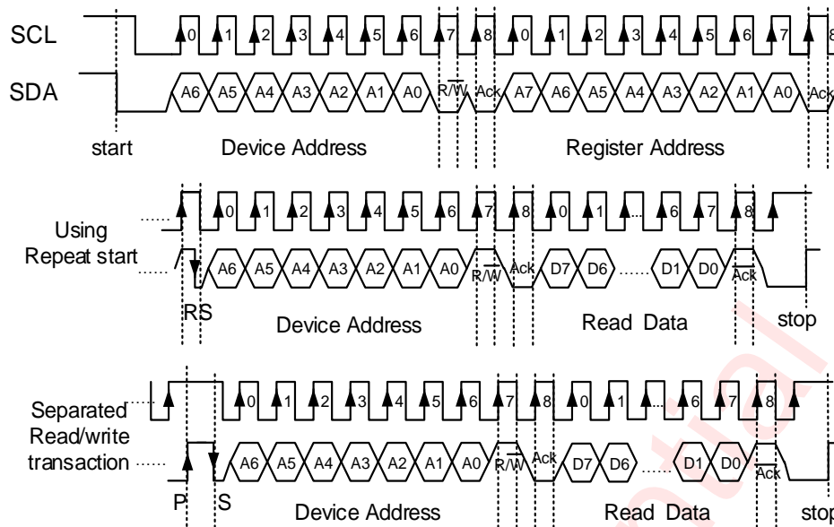
Figure 11 I 2 C Read Byte Cycle
