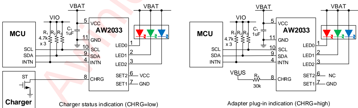
Figure 3 Typical Application Circuits
