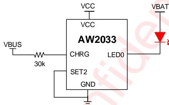
Figure 16 USB Power Insertion Status Indication in PMU-controlled Charging Application
