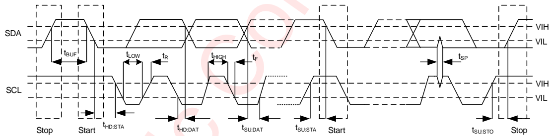
Figure 4 Timing of I 2 C Interface Signals
