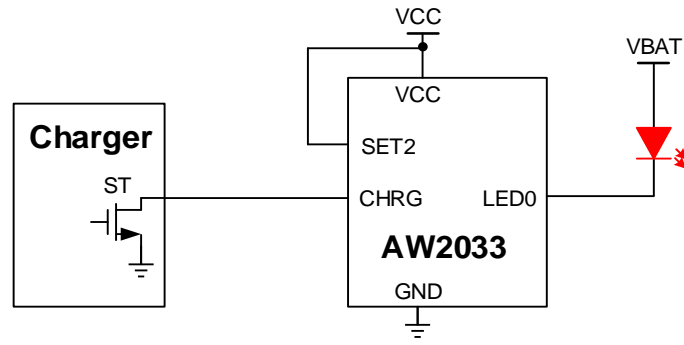
Figure 15 Real Charging Status Indication in Special Charger IC Application
