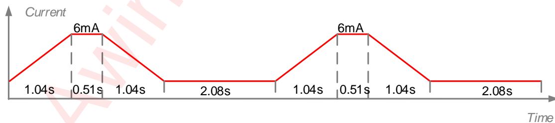
Figure 14 Auto Charging Indication Pattern Parameter
