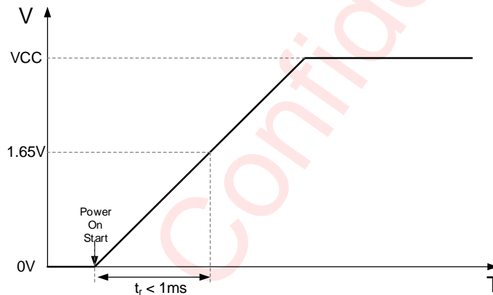
Figure 5 AW2033 Power on Timing
