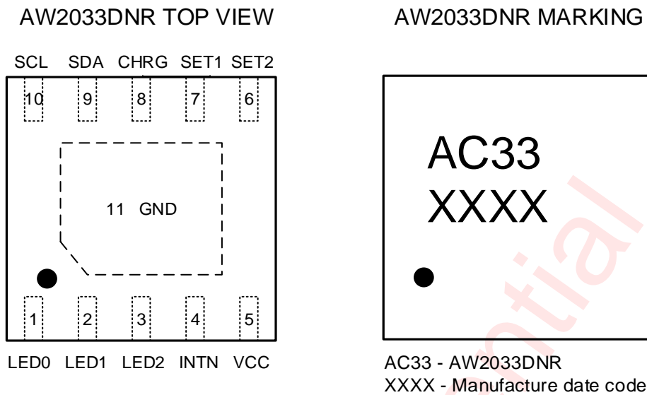
Figure 1 Pin Configuration and Top Marking
