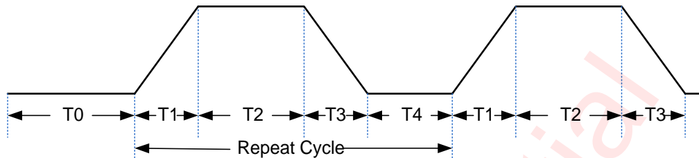
Figure 12 LED Breath Timing in Pattern Mode
