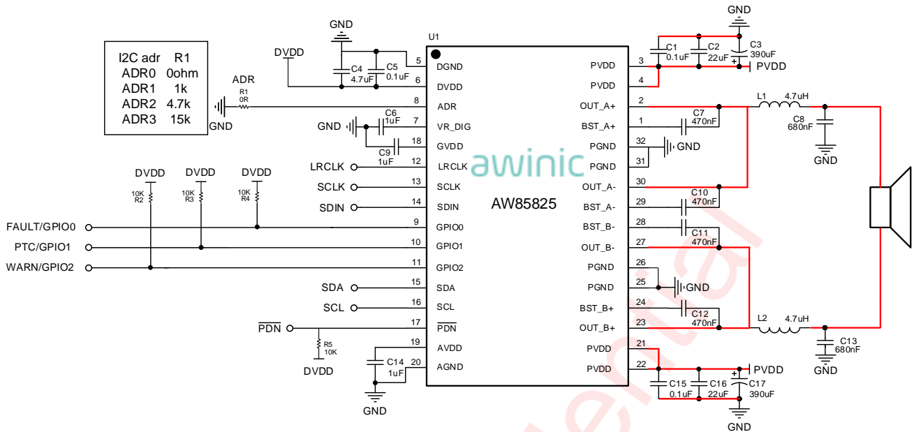
Figure 3 AW85825 PBTl Application Circuit
