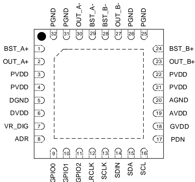
AW85825QNR (Top View)
