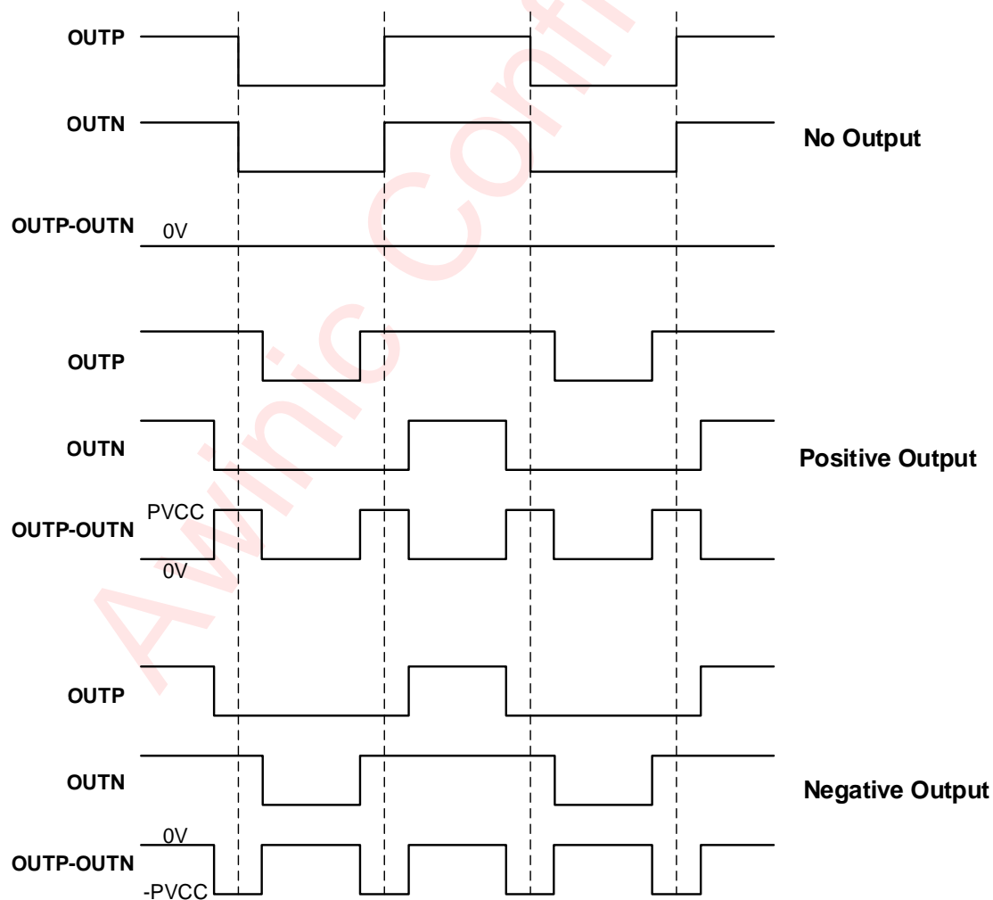
Figure 13 BD Mode Modulation
