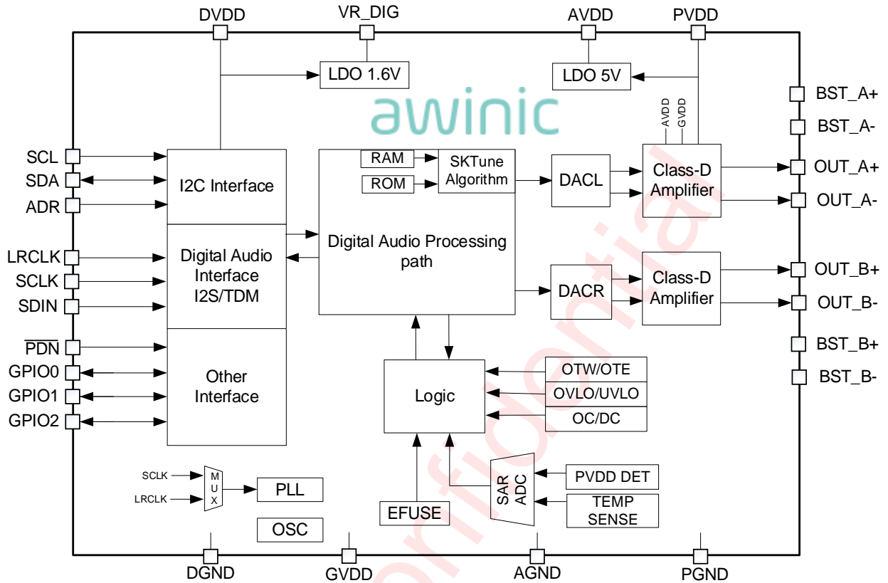
Figure 1 AW85825 Functional Diagram
