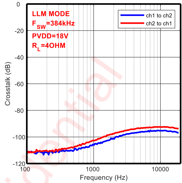
CROSSTALK -BTL
