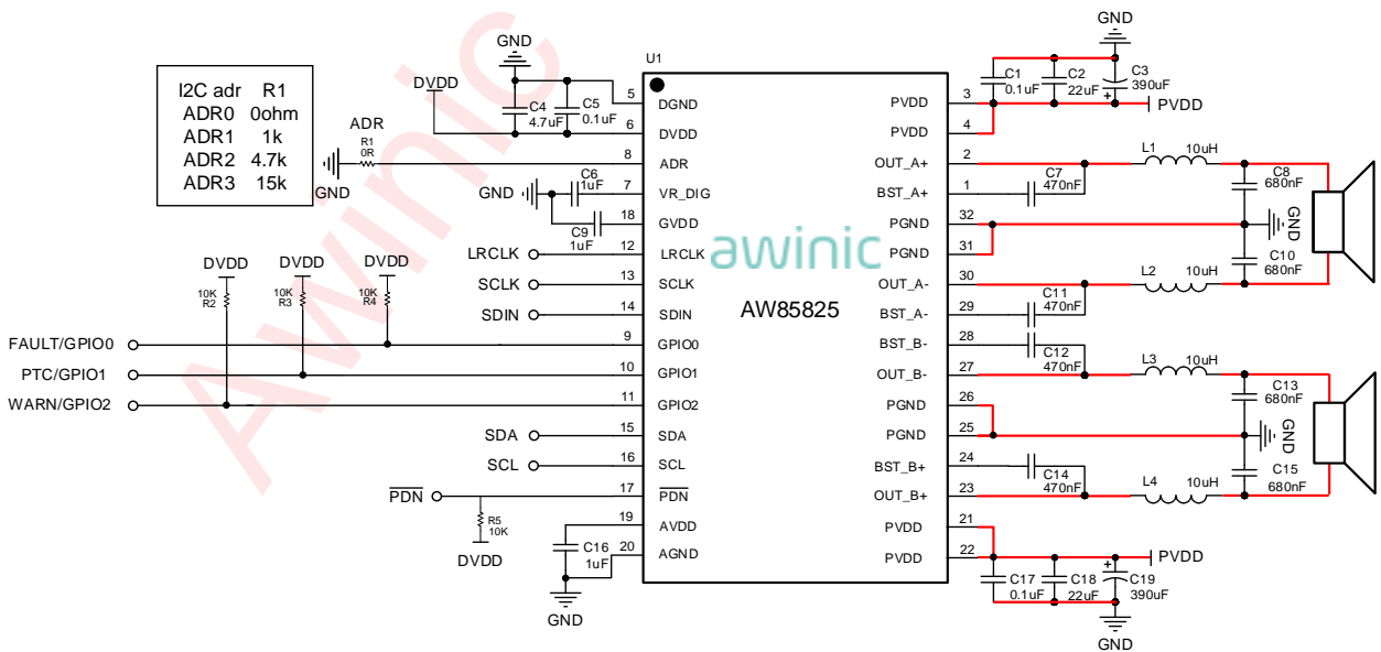
Figure 2 AW85825 BTL Application Circuit
