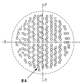
100 contacts size 22D
