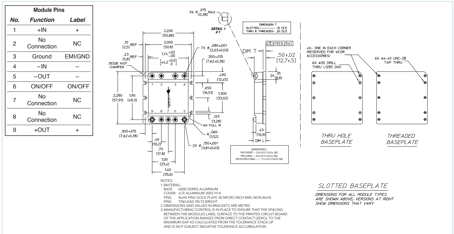
Figure 7 — Mechanical diagram
