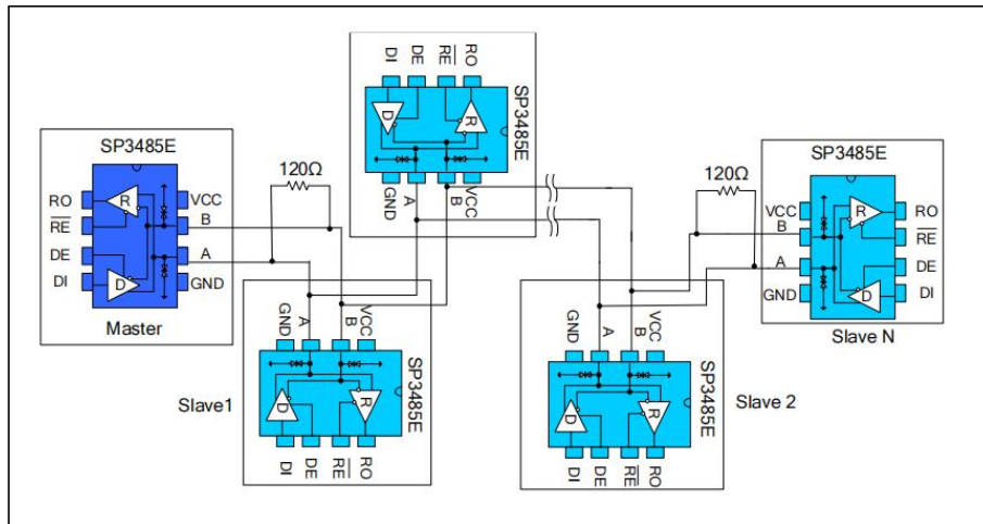
Figure10 Hand in hand SP3485EN-L/TR half duplex communication network
