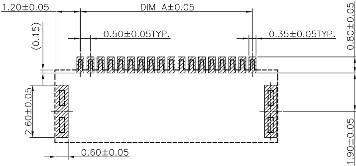
RECOMMENDED P.C.B PATTERN LAYOUT (TOP VIEW) TOLERANCE: ±0.05
