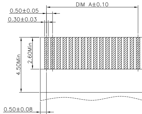
RECOMMENDED FPC/FFC DIMENSION (TOP VIEW)
