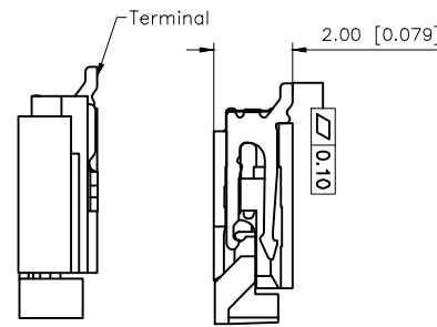
SECTION:A-A SCALE:1:1
