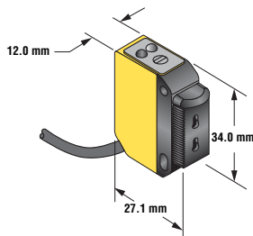
Opposed, Retroreflective and Diffuse Models Suffix E, R, LP and D
