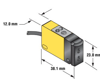
Opposed, Retroreflective and Diffuse Models Suffix E, R, LP and D
