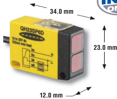
Opposed, Retroreflective and Diffuse Models Suffix E, R, LP and D
