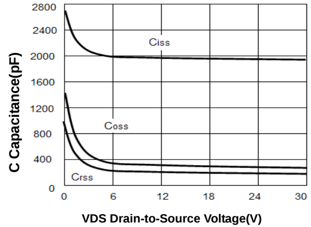
Figure 8. Capacitance
