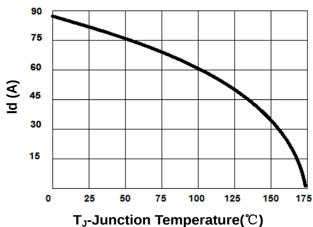
Figure 4. Drain Current
