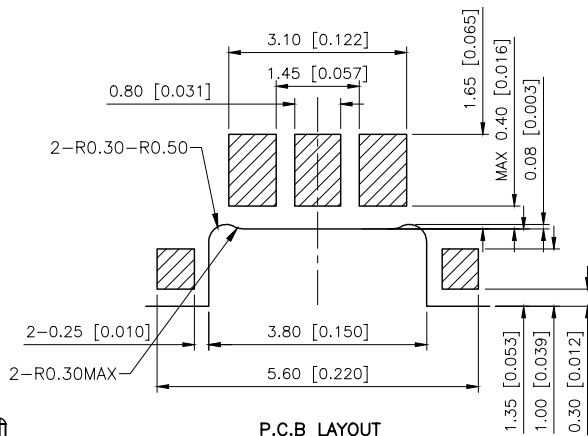
P.C.B LAYOUT VIEW FORM THE DIRECTION A
