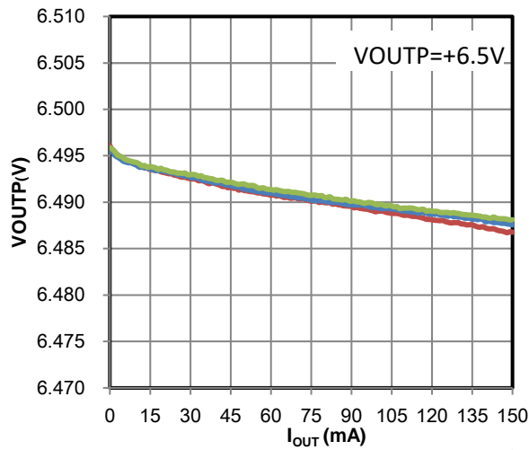
Figure 29 Load Regulation (150mA Mode)
