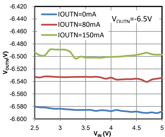
Figure 22 Line Regulation (150mA Mode)
