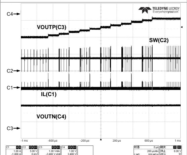
Figure 58 Ramp Up (VOUTP)
