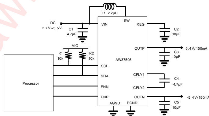
Figure 1 Typical Application Circuit of AW37505
