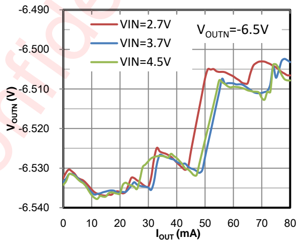
Figure 26 Load Regulation (80mA Mode)
