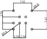
Pcb plate opening size (PCB板开孔尺寸)
