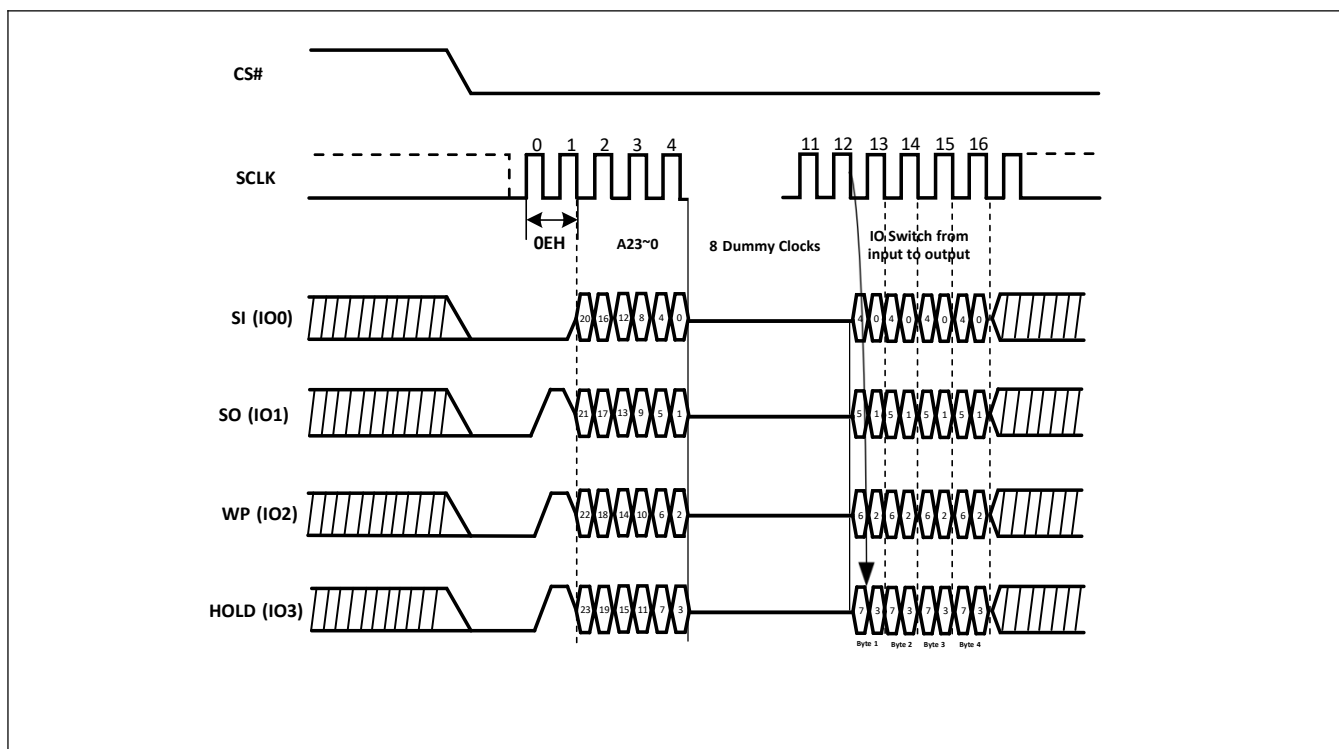
Figure-36. DTR Burst Read with Wrap Sequence ( QPI )
