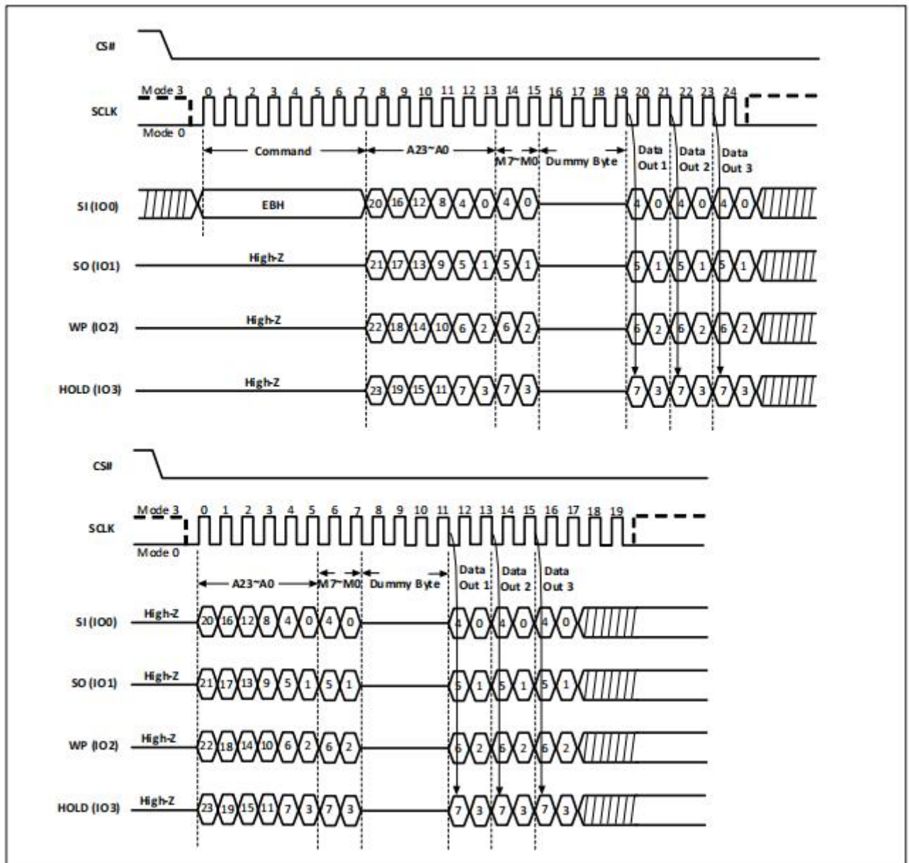
Figure-29. Quad I/O Fast Read with “Continuous Read Mode” Sequence Diagram (M5-4 = (1,0))
