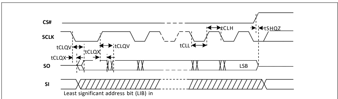
Figure-87. Output Timing (DTR mode)
