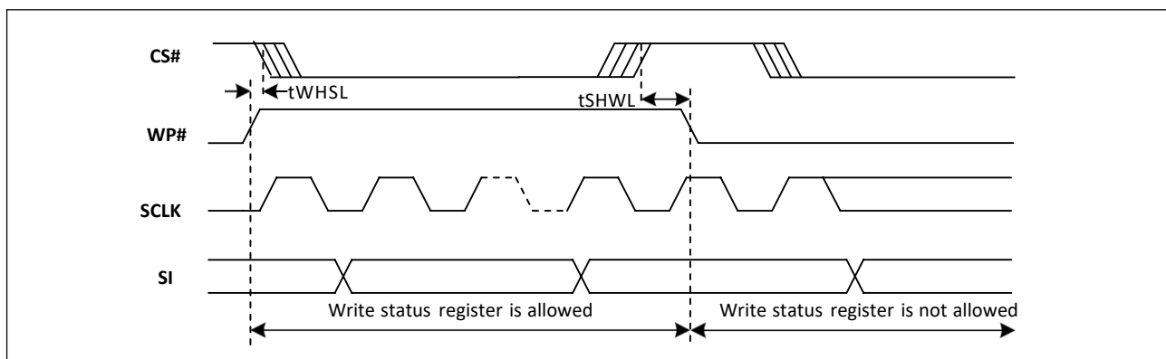
Figure-89. WP Timing
