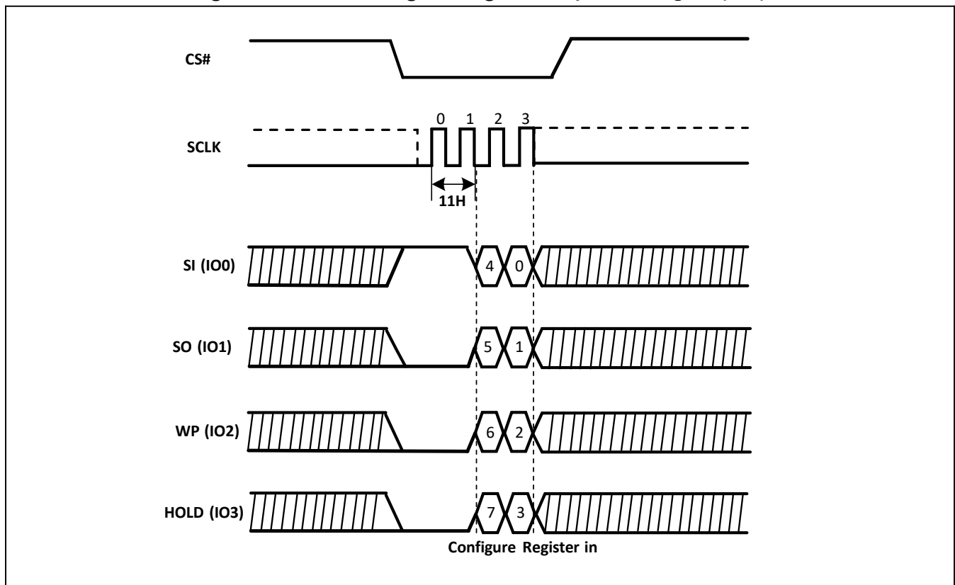
Figure-16. Write Configure Register Sequence Diagram(QPI)
