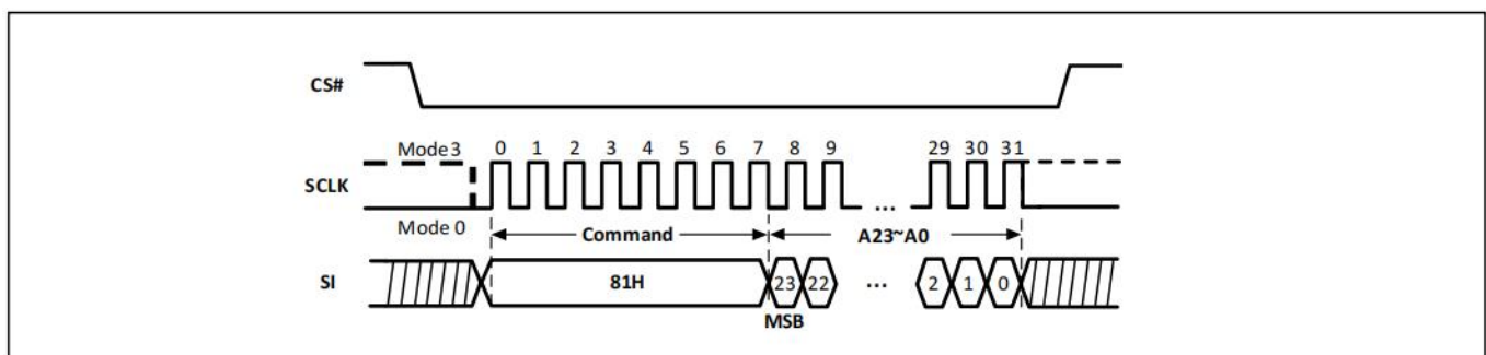
Figure-38. Page Erase Sequence Diagram
