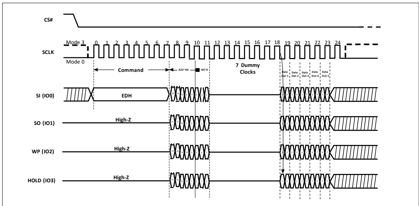
Figure-31. DTR Fast Read Quad I/O Sequence Diagram (M5-4 ≠ (1,0))
