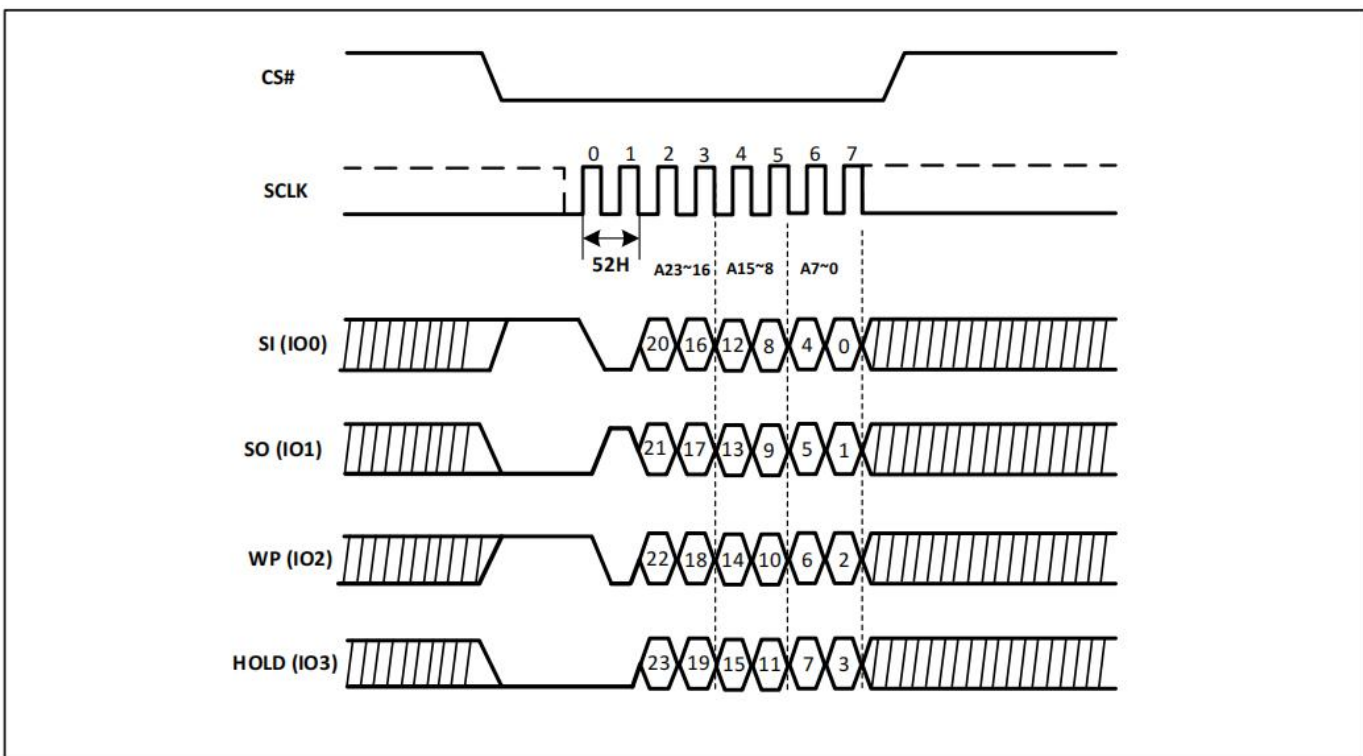
Figure-43. Half Block Erase Sequence Diagram (QPI)
