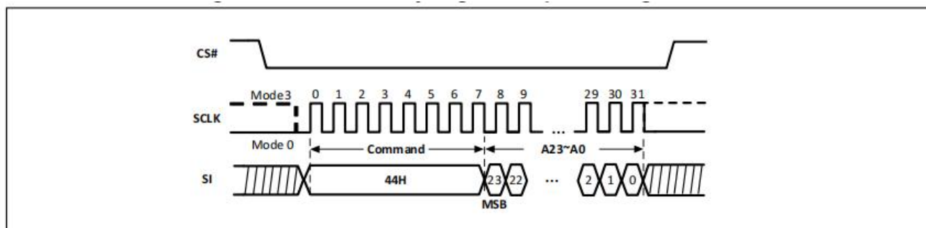
Figure-51. Erase Security Register Sequence Diagram
