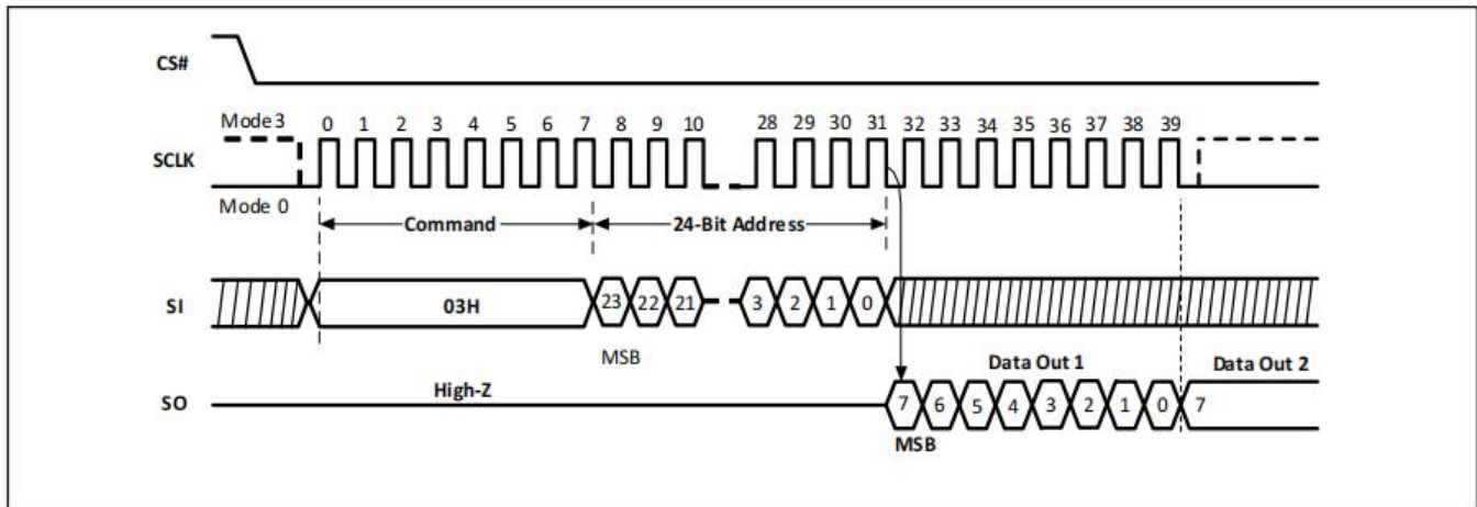
Figure-17. Read Data Bytes Sequence Diagram
