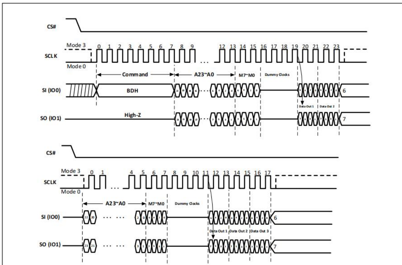
Figure-26. DTR Fast Read Dual I/O with “Continuous Read Mode” Sequence Diagram (M5-4 = (1,0))
