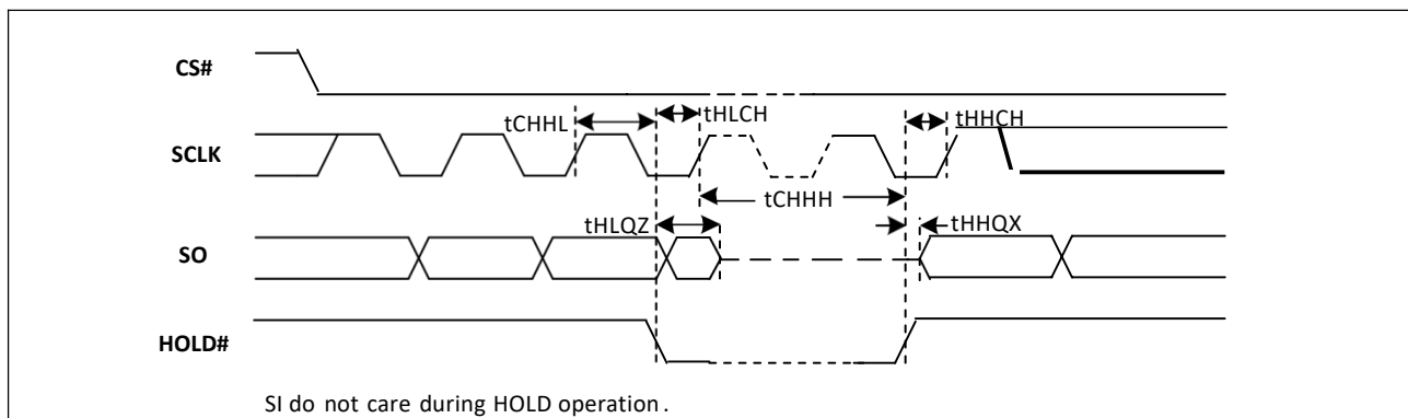
Figure-88. Hold Timing
