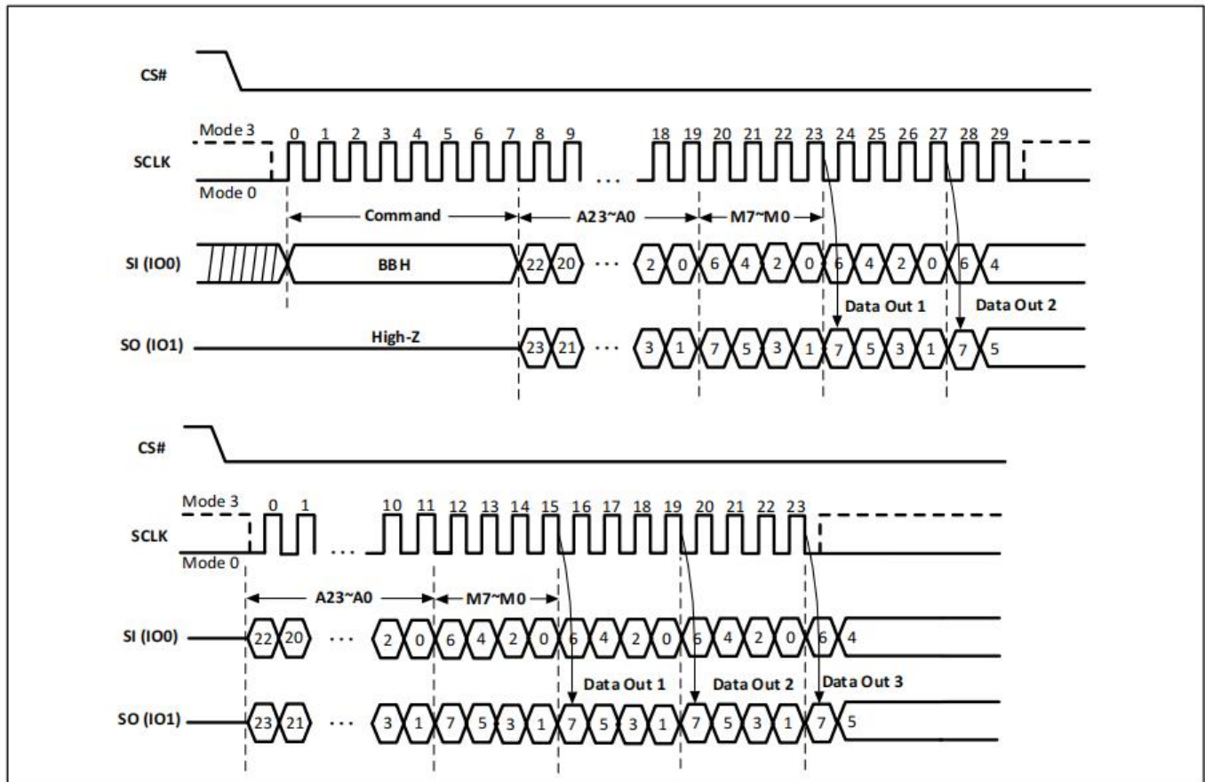
Figure-24. Dual I/O Fast Read with “Continuous Read Mode” Sequence Diagram (M5-4 = (1,0))
