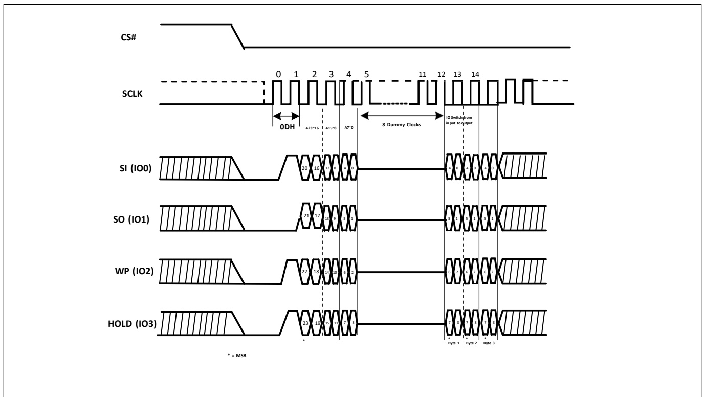
Figure-21. DTR Fast Read Sequence Diagram (QPI)
