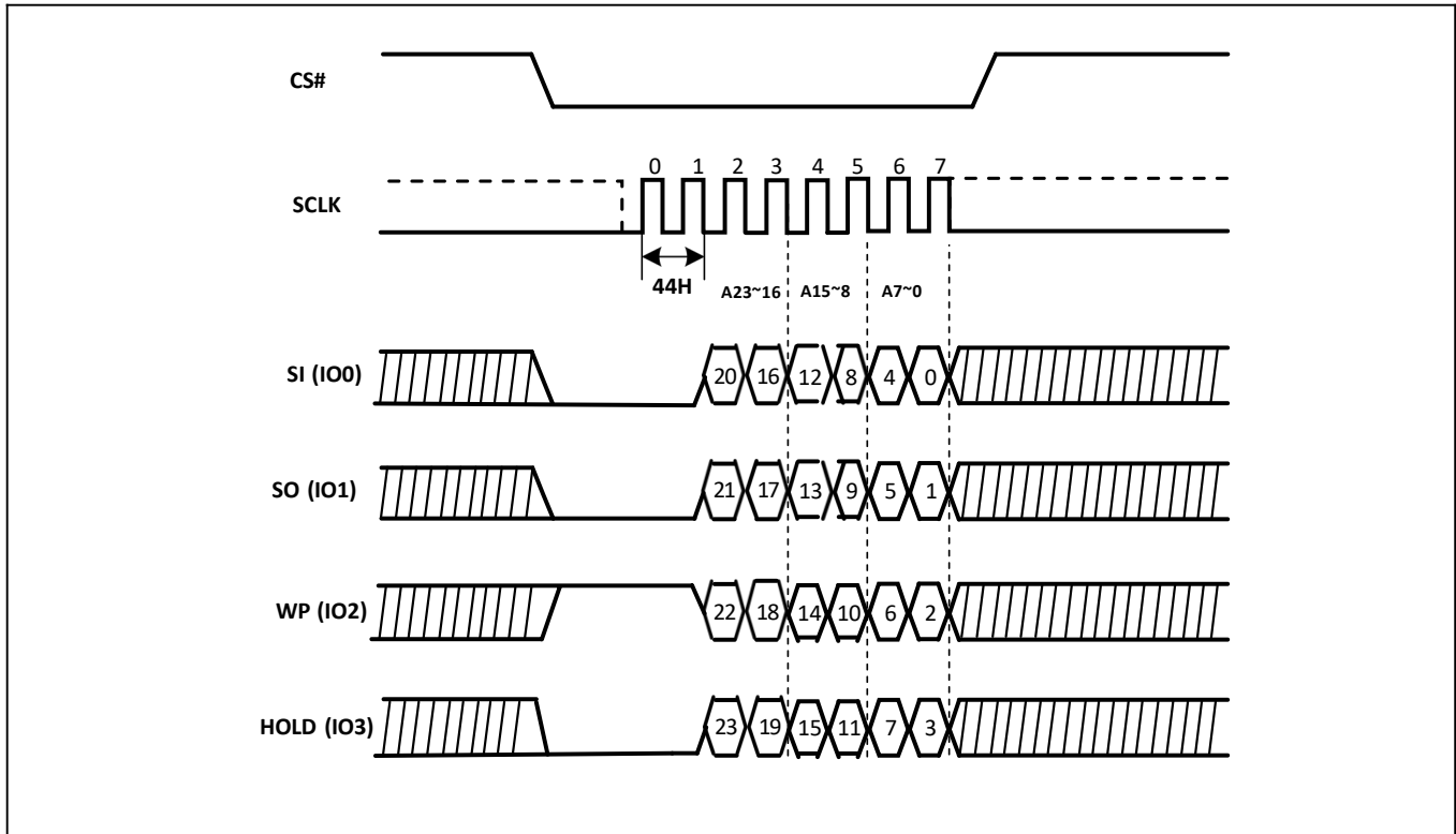
Figure-52. Erase Security Register Sequence Diagram (QPI)
