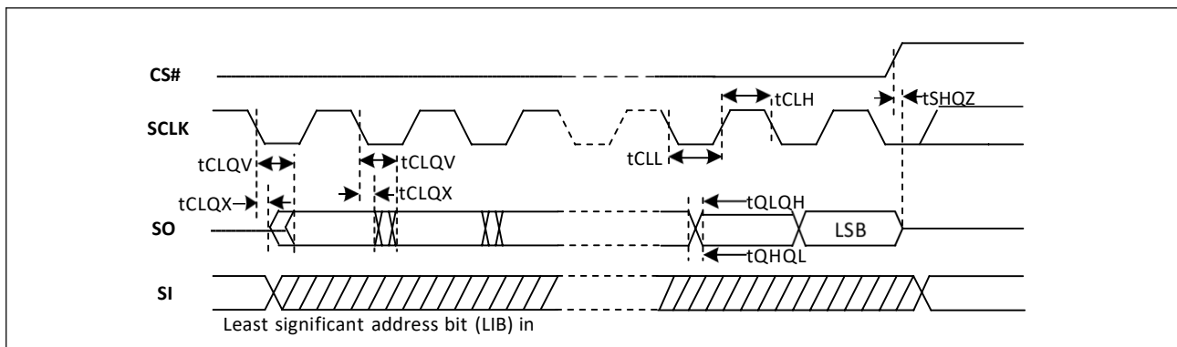
Figure-87. Output Timing (DTR mode)
