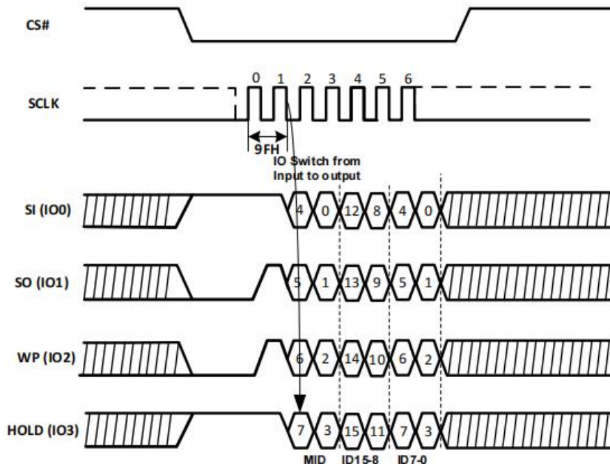
Figure-68. Read Identification Sequence Diagram (QPI)
