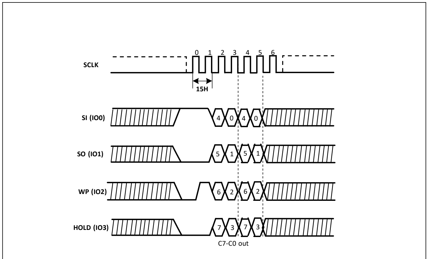
Figure-12. Read Configure Register Sequence Diagram (QPI)
