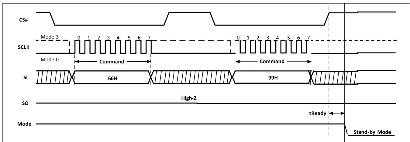
Figure-80. Reset Enable and Reset Sequence Diagram
