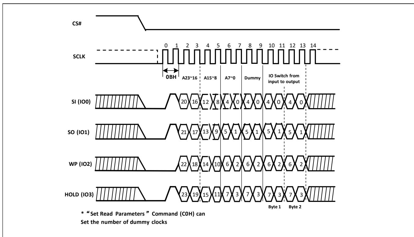
Figure-19. Read Data Bytes at Higher Speed Sequence Diagram (QPI)
