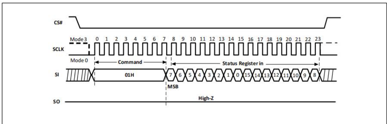
Figure-13a. Write Status Register Sequence Diagram(Command 01H)
