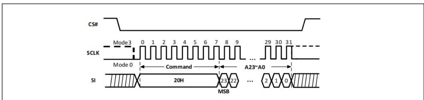
Figure-40. Sector Erase Sequence Diagram
