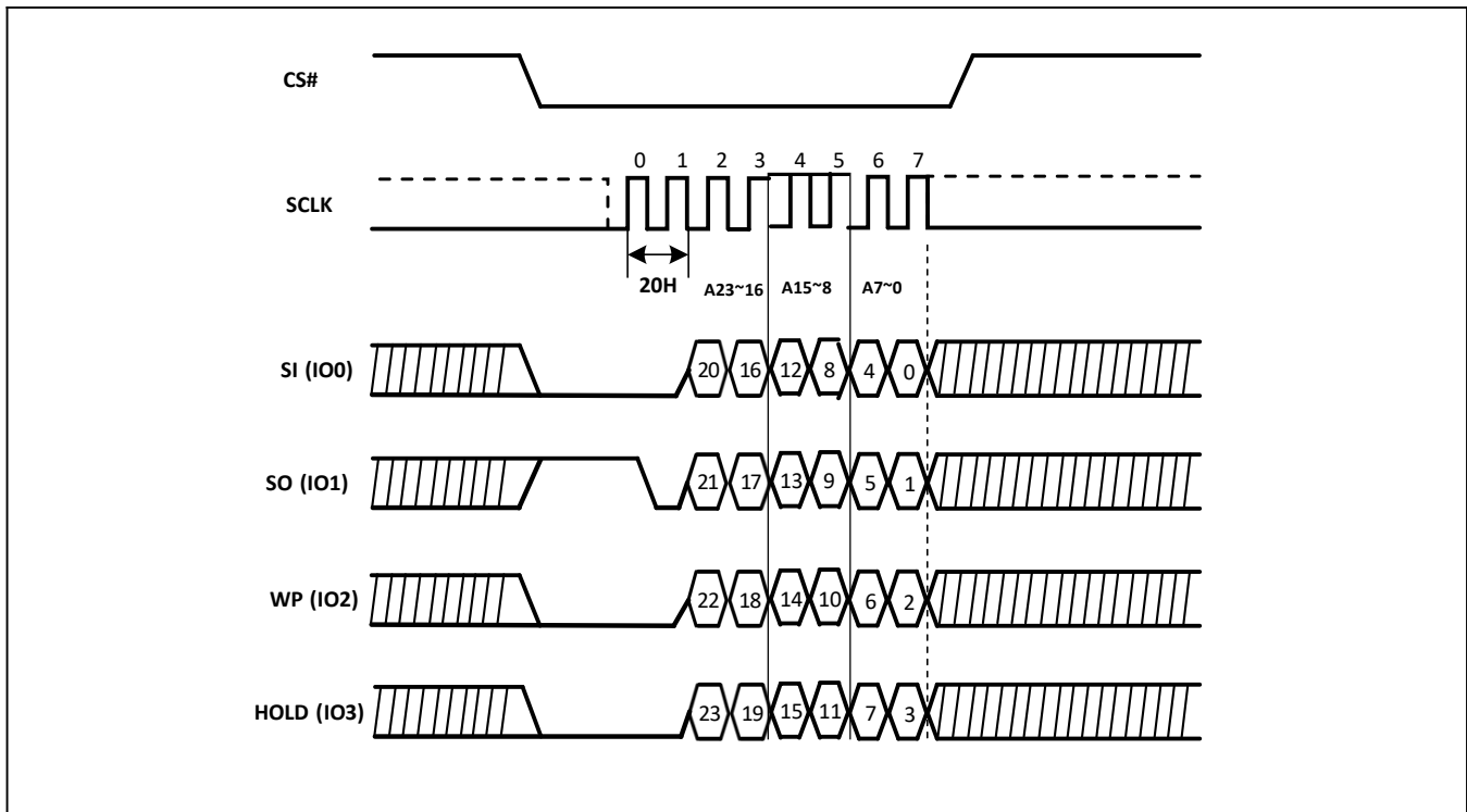
Figure-41. Sector Erase Sequence Diagram (QPI)
