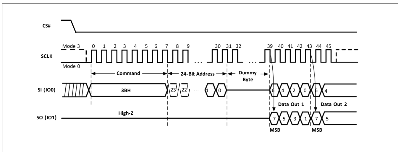
Figure-22. Dual Output Fast Read Sequence Diagram
