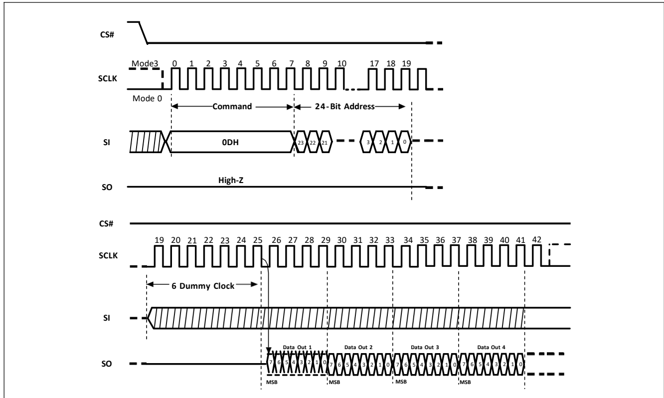
Figure-20. DTR Fast Read Sequence Diagram (SPI)
