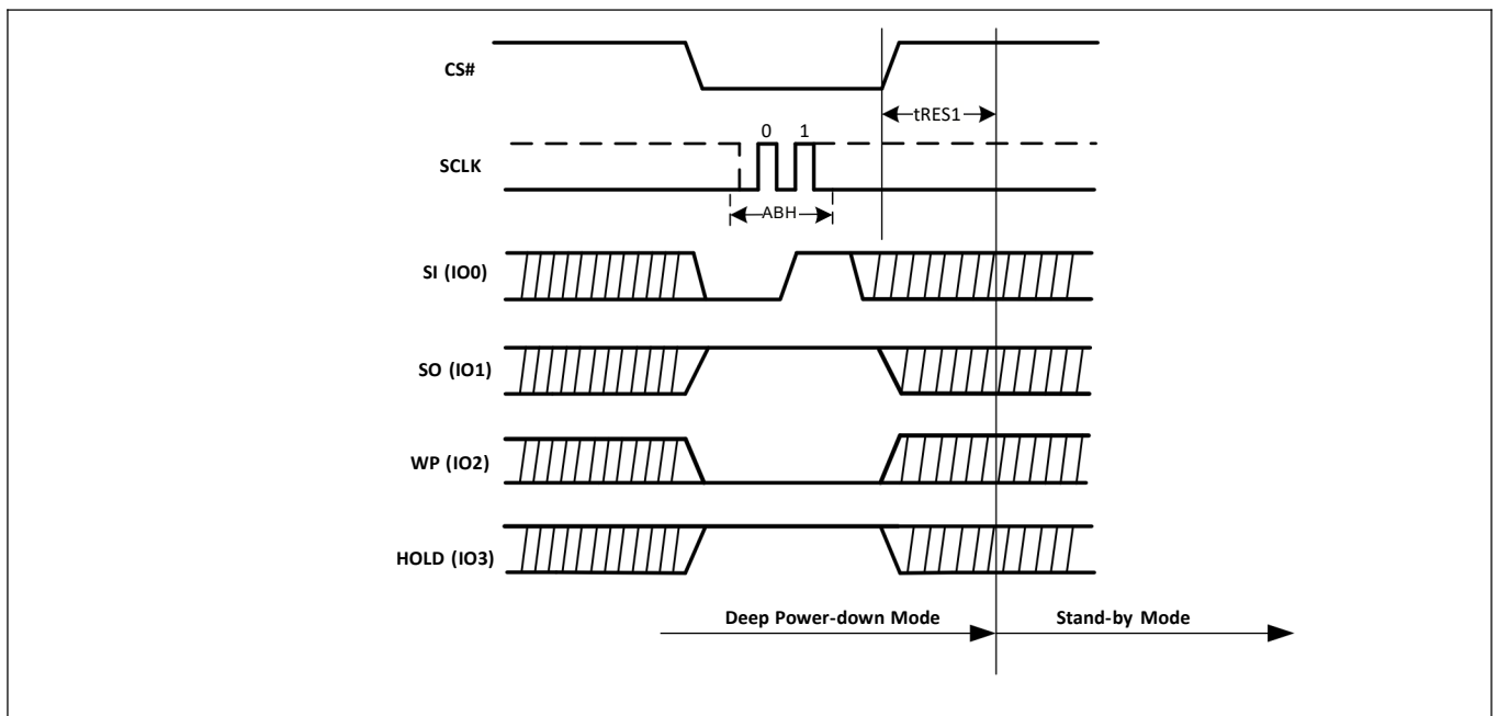
Figure-60. Release from Deep Power-Down (RDP) Sequence Diagram (QPI)
