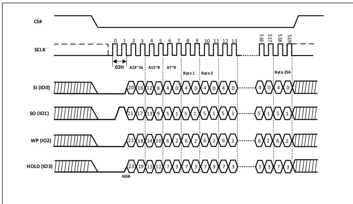
Figure-49. Page Program Sequence Diagram (QPI)
