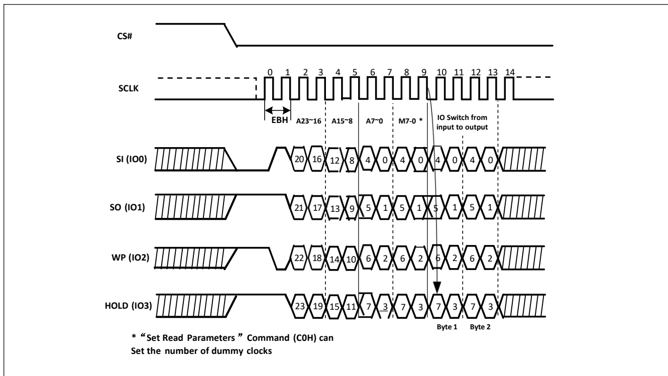
Figure-30. Quad I/O Read in QPI Mode Sequence (M5-4 ≠ (1,0))
