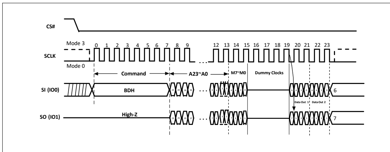
Figure-26. DTR Fast Read Dual I/O with “Continuous Read Mode” Sequence Diagram (M5-4 = (1,0))
