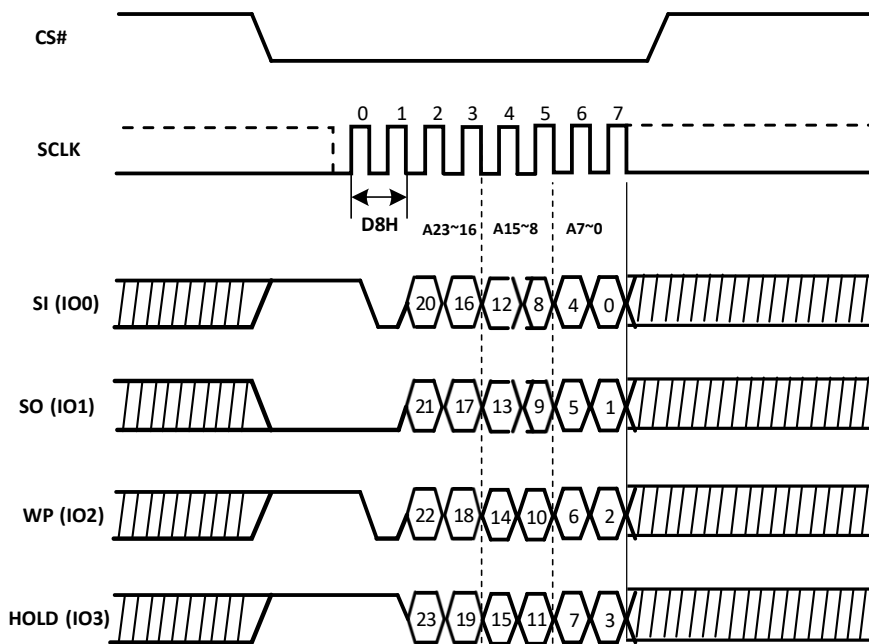
Figure-45. Block Erase Sequence Diagram (QPI)
