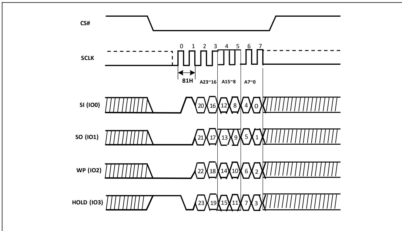
Figure-39. Page Erase Sequence Diagram (QPI)
