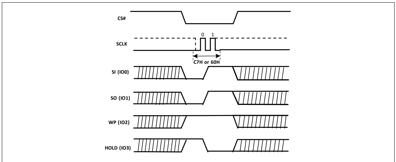
Figure-47. Chip Erase Sequence Diagram (QPI)
