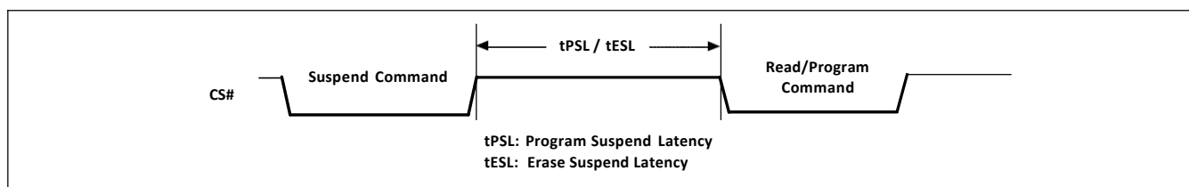
Figure-70. Suspend to Read/Program Latency
