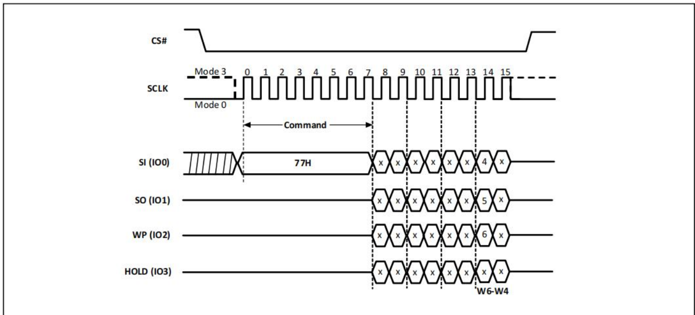
Figure-37. Set Burst with Wrap Sequence Diagram
