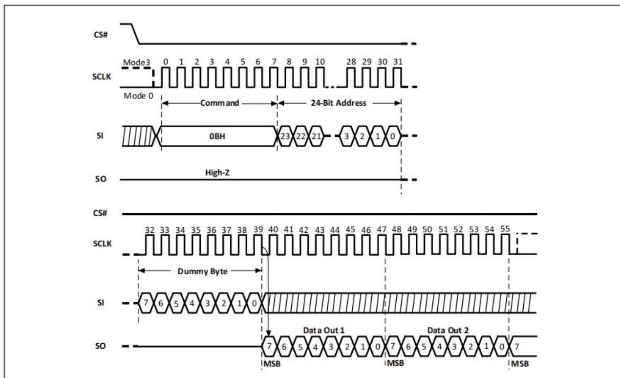
Figure-18. Read Data Bytes at Higher Speed Sequence Diagram
