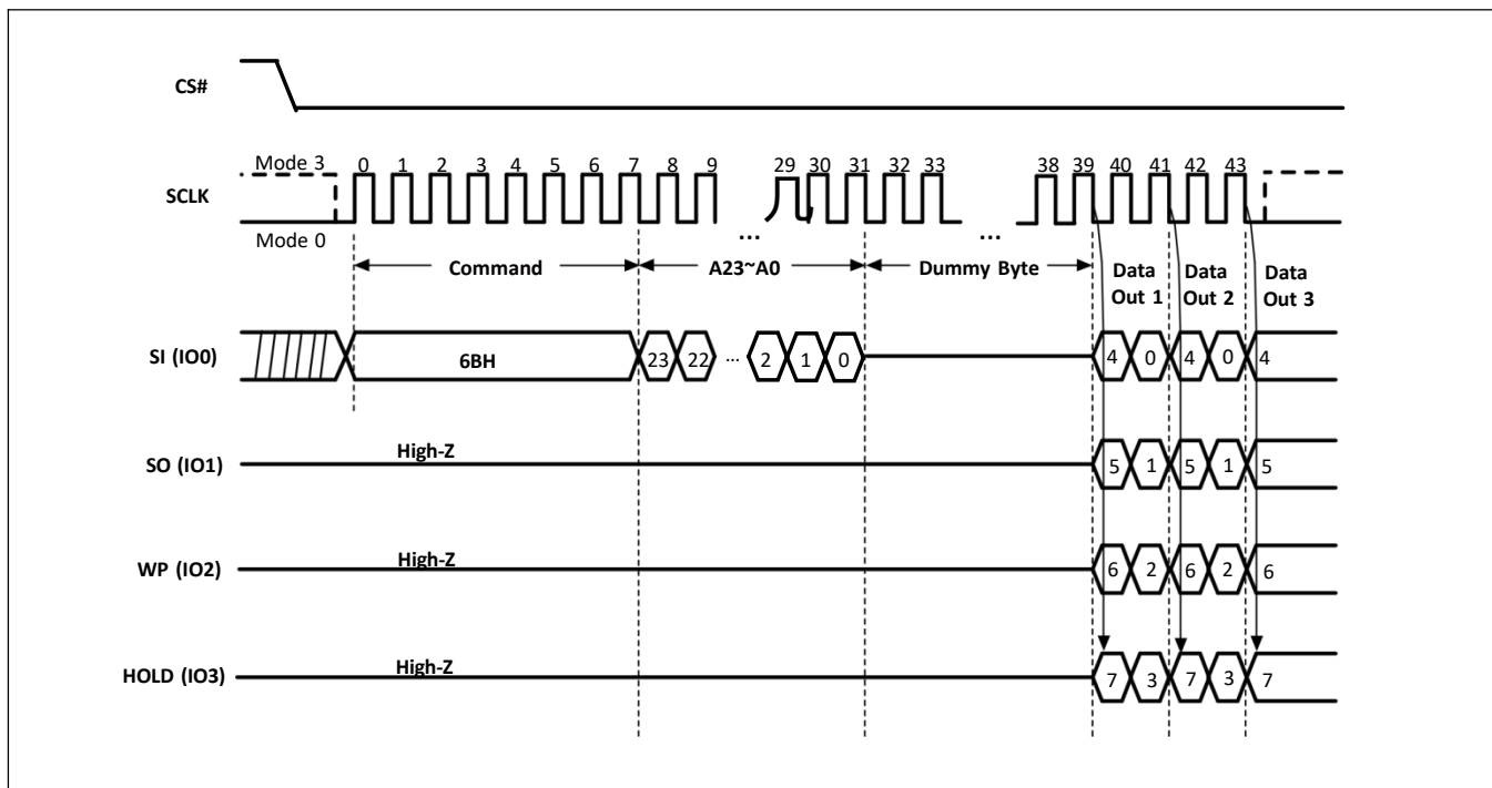
Figure-27. Quad Output Fast Read Sequence Diagram
