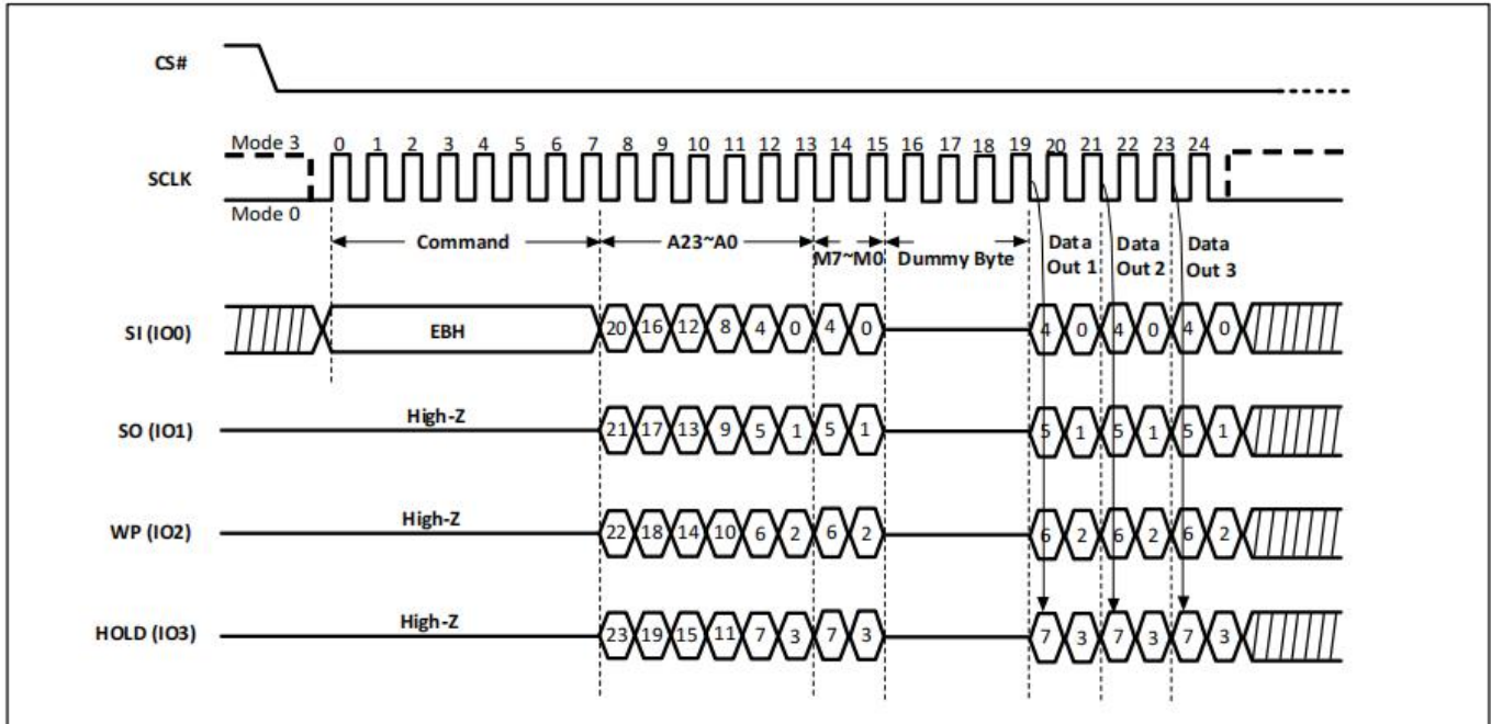
Figure-28. Quad I/O Fast Read Sequence Diagram (M5-4 ≠ (1,0))
