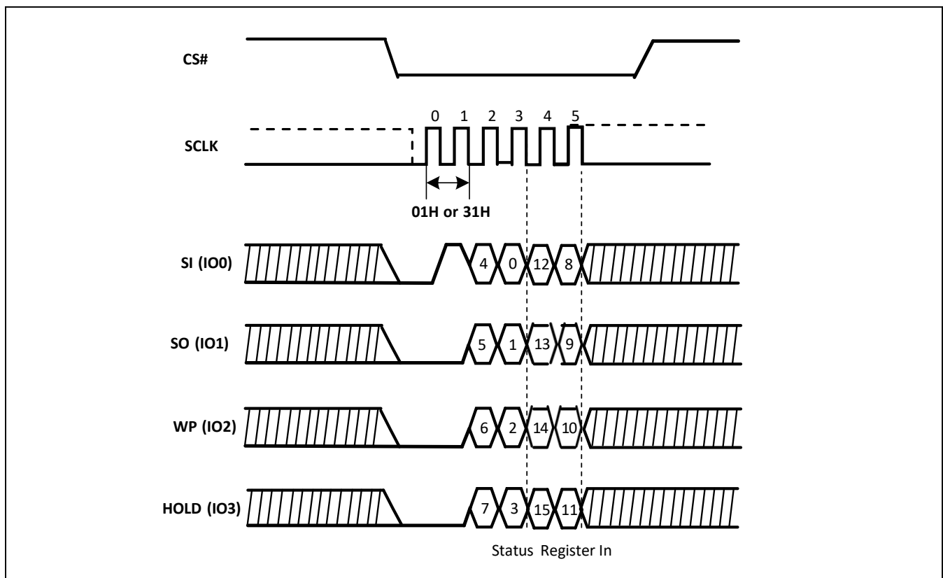
Figure-14. Write Status Register Sequence Diagram (QPI)
