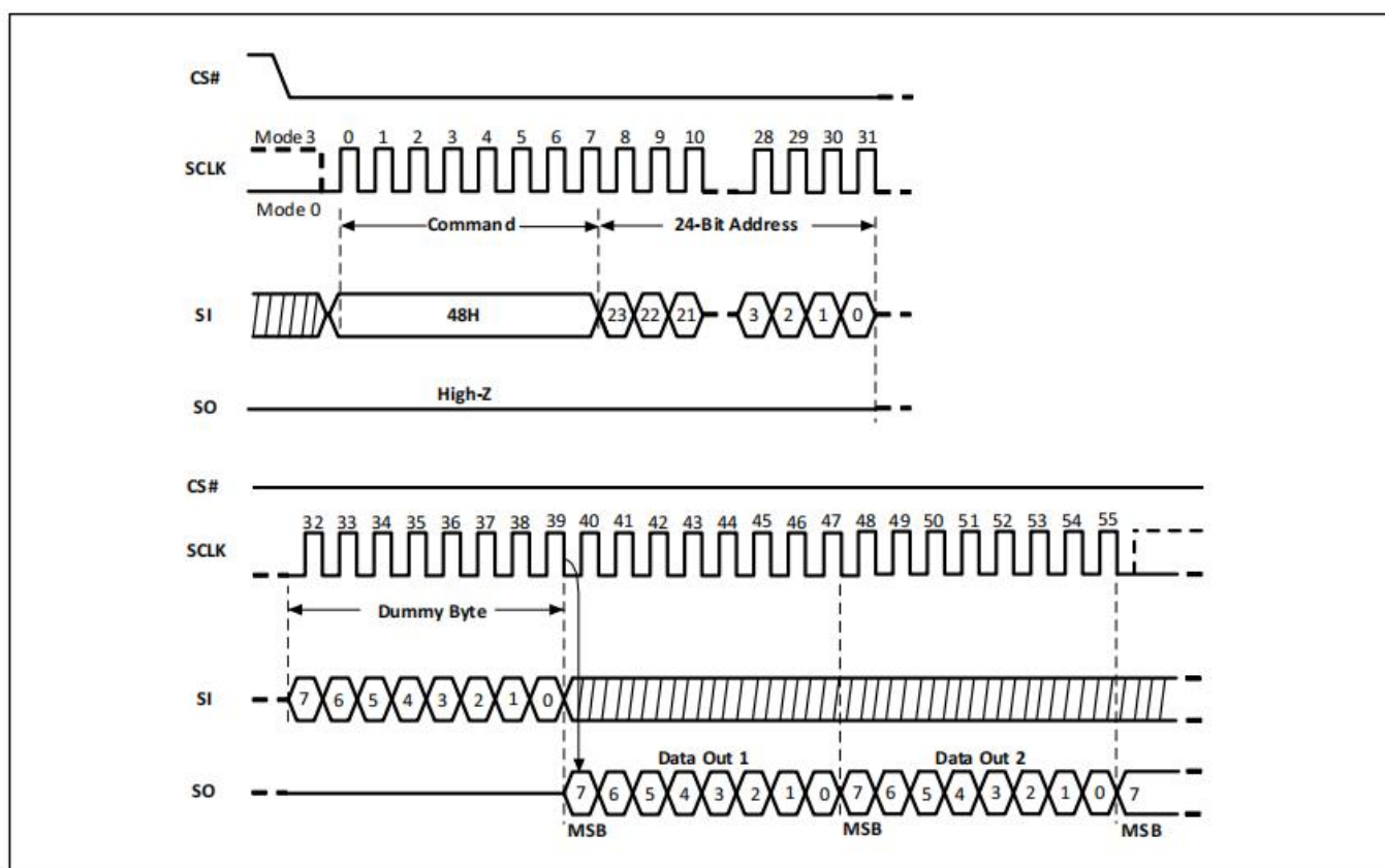
Figure-55. Read Security Register Sequence Diagram
