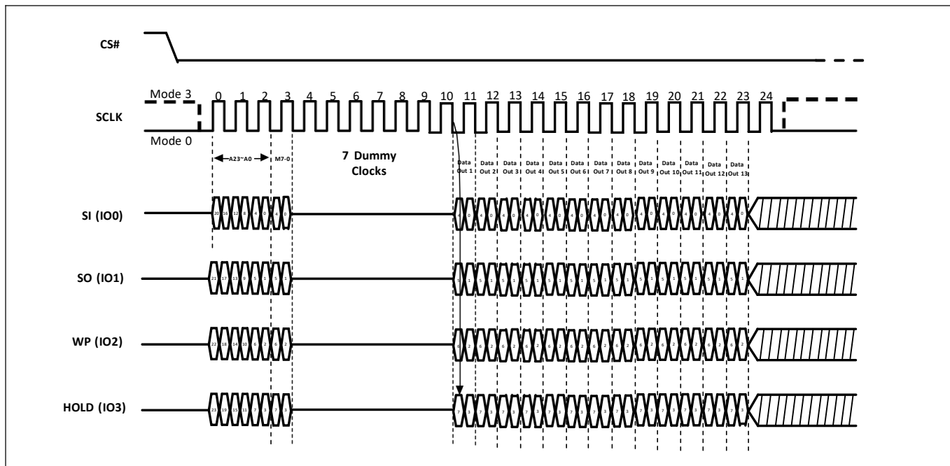
Figure-32. Quad I/O Fast Read with “Continuous Read Mode” Sequence Diagram (M5-4 = (1,0))
