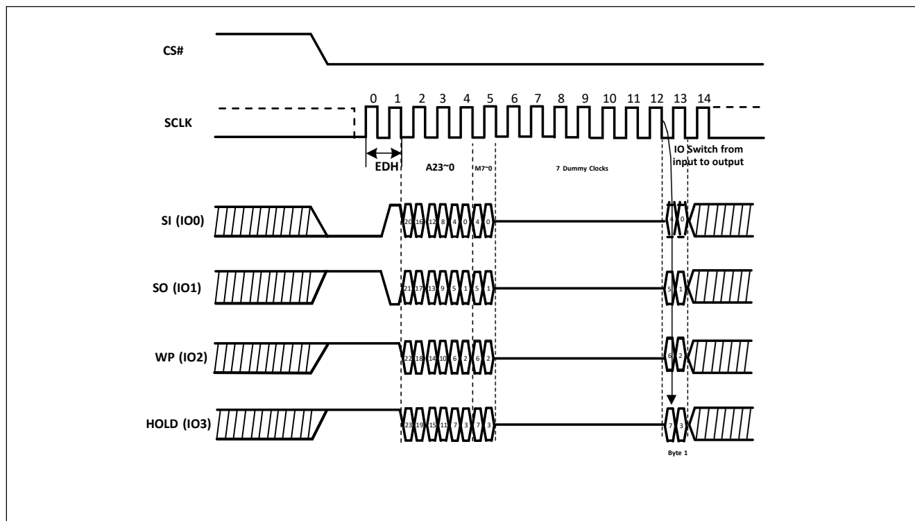
Figure-33. DTR Fast Read Quad I/O in QPI Mode Sequence (M5-4 ≠ (1,0))
