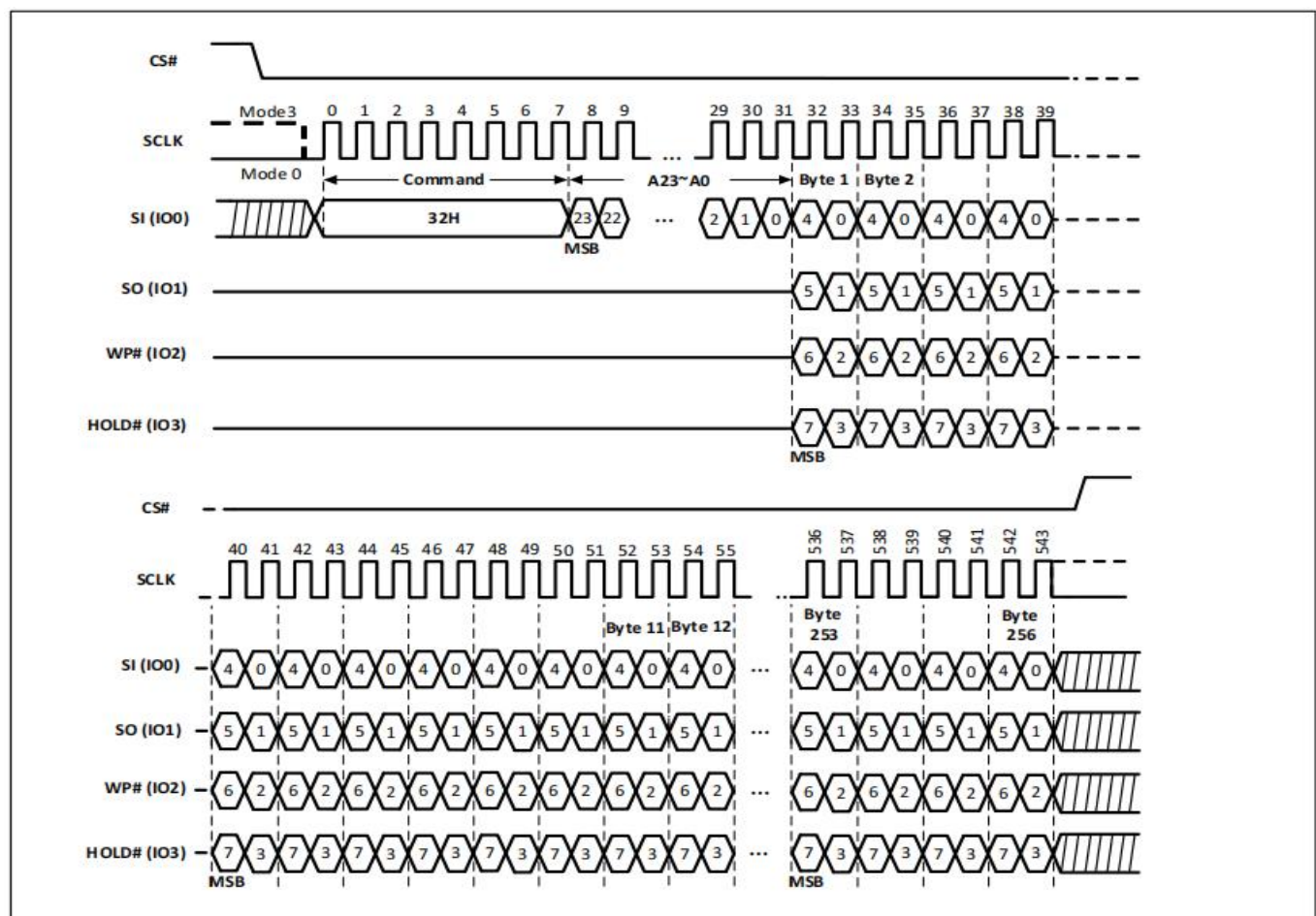
Figure-50. Quad Input Page Program Sequence Diagram
