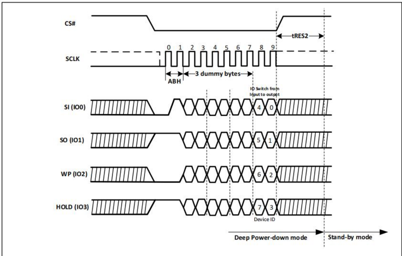
Figure-62. Read Electronic Signature (RES) Sequence Diagram (QPI)
