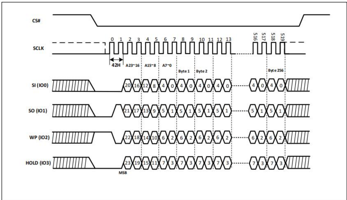
Figure-54. Program Security Register Sequence Diagram(QPI)
