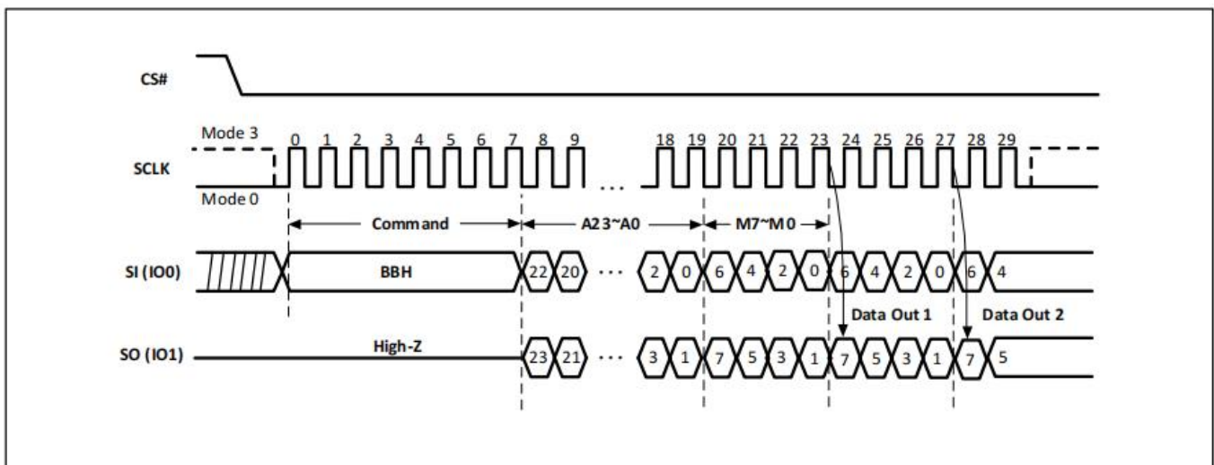
Figure-23. Dual I/O Fast Read Sequence Diagram (M5-4 ≠ (1,0))
