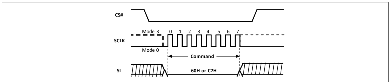
Figure-46. Chip Erase Sequence Diagram
