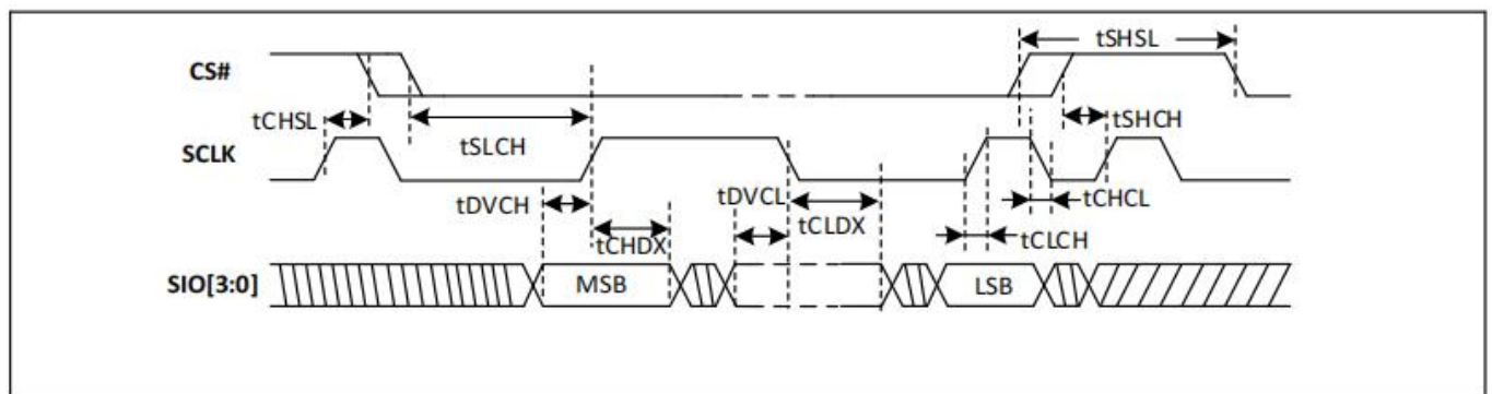
Figure-85. Serial Input Timing (DTR mode)
