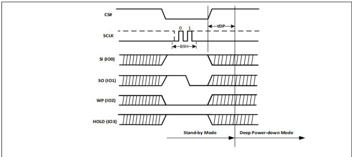
Figure-58. Deep Power-Down Sequence Diagram (QPI)
