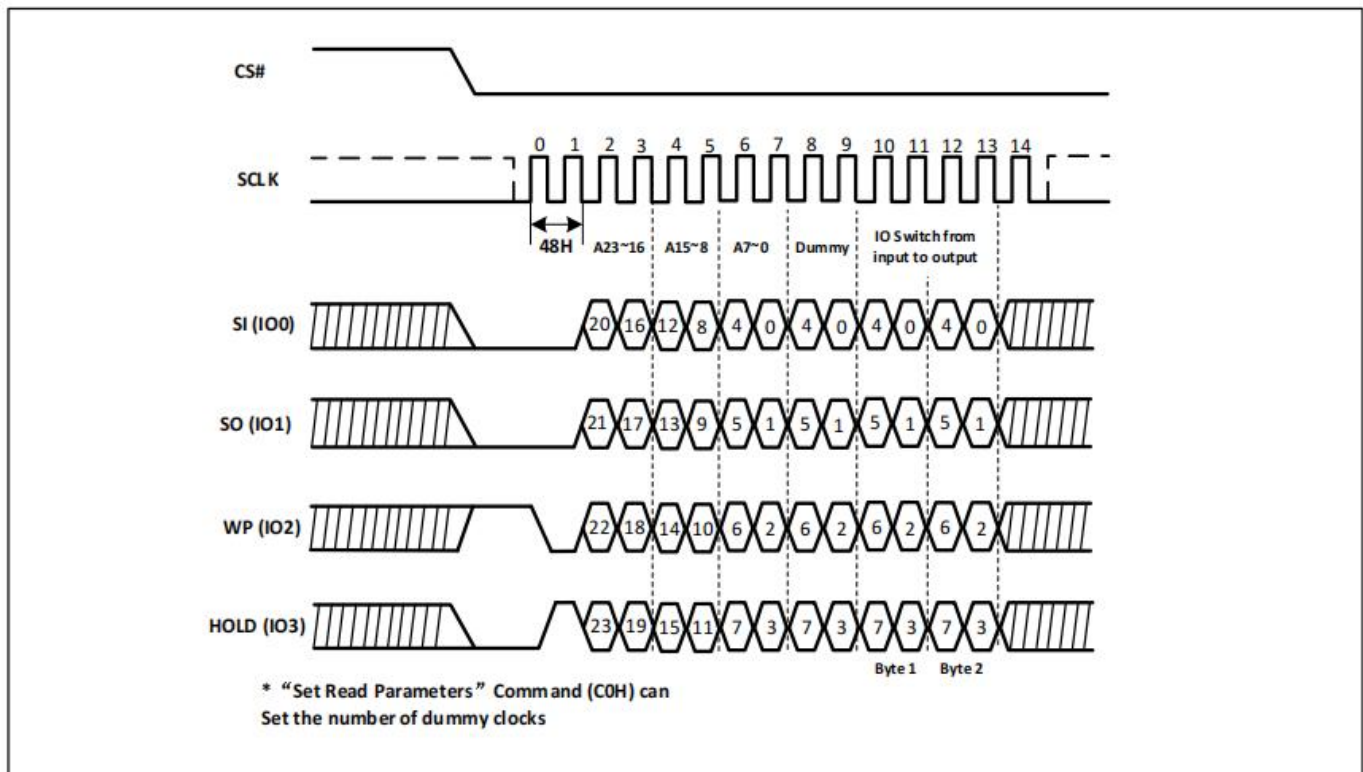
Figure-56. Read Security Register Sequence Diagram (QPI)
