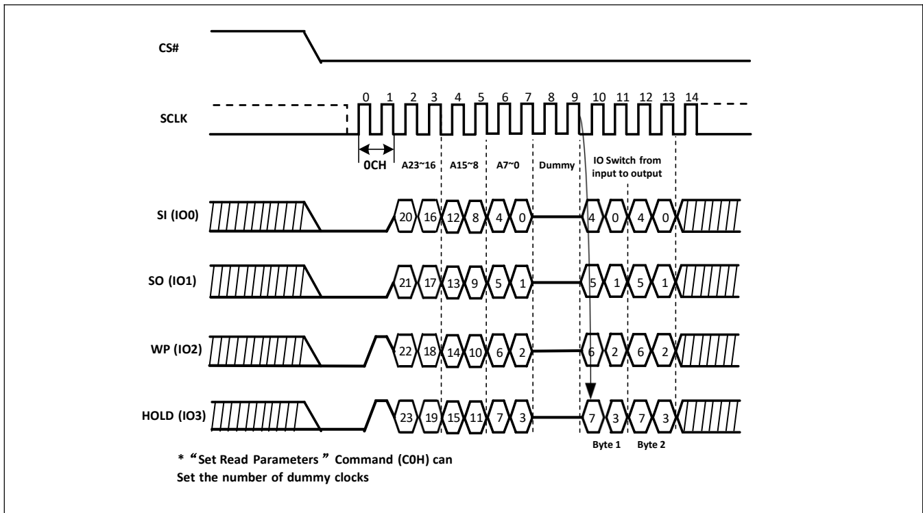
Figure-35. Burst Read with Wrap Sequence ( QPI )
