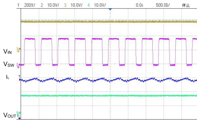
(23) Steady State ( V_{IN}=20.0V, V_{OUT}=12V, I_{OUT}=0.6A )
