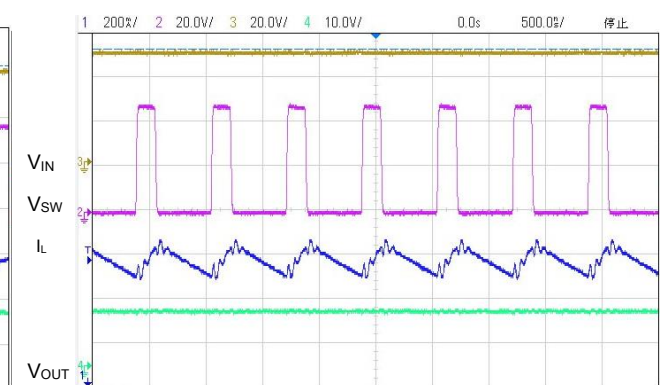
(24) Steady State ( V_{IN}=50.0V, V_{OUT}=12V, I_{OUT}=0.6A )
