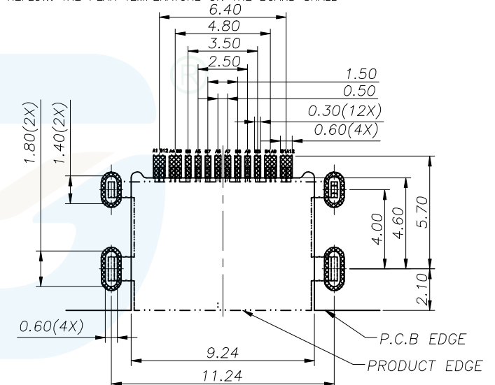
RECOMMENDED PCB LAYOUT(TOP VIEW) THICKNESS 0.80MM;DEFAULT TOLERANCE:±0.05
