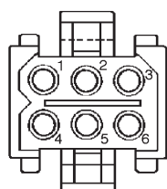
Plug
