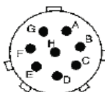
Shell Size 12
