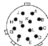
Shell Size 14
