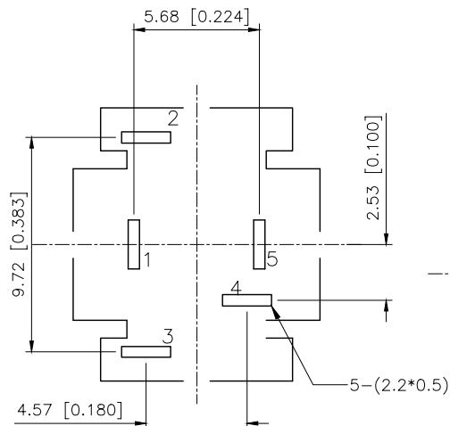
PCB Layout
