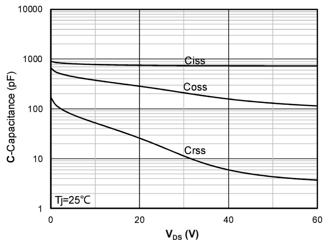
Capacitance Characteristics
