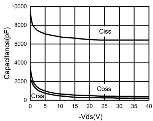
Figure 8. Capacitance
