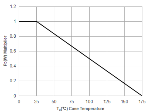
Figure 3. Power Dissipation
