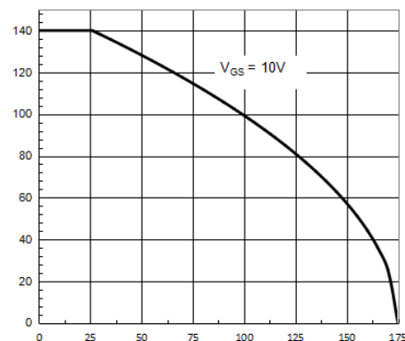
Figure 4. Drain Current
