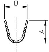
SECTION:A-A SCALE:1:1
