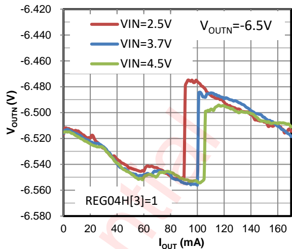
Figure 46 Load Regulation (170mA Mode)
