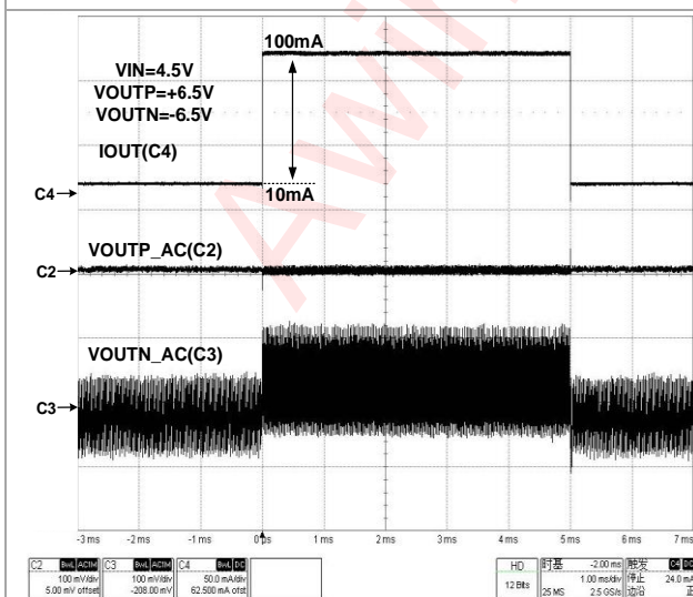
Figure 46 Load Transient (100mA Mode)
