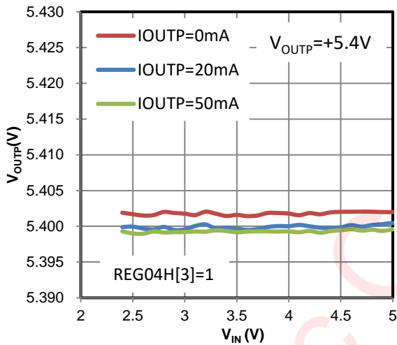
Figure 14 Line Regulation (50mA Mode)
