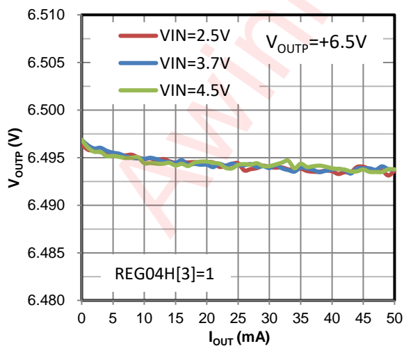
Figure 28 Load Regulation (50mA Mode)
