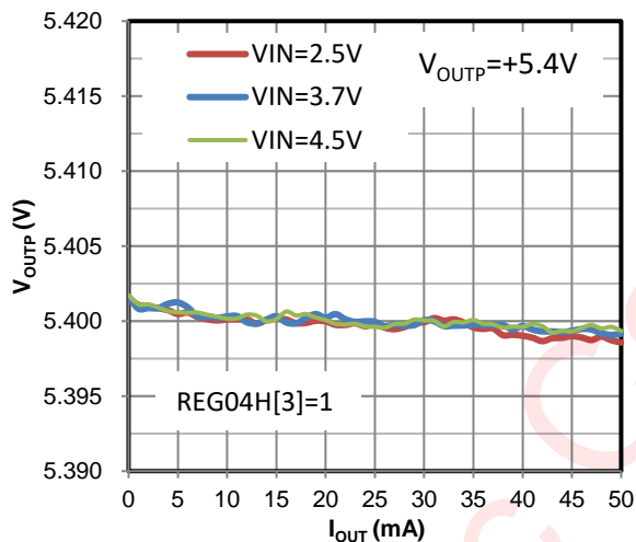
Figure 26 Load Regulation (50mA Mode)
