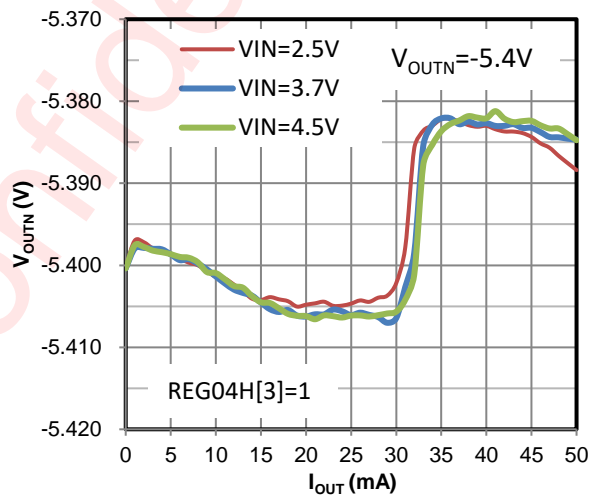
Figure 27 Load Regulation (50mA Mode)
