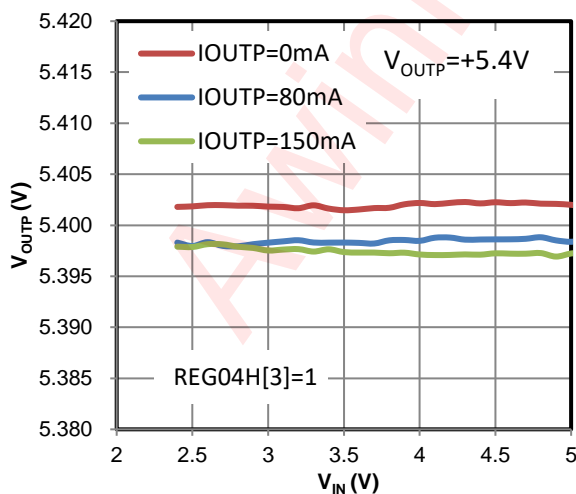
Figure 22 Line Regulation (170mA Mode)
