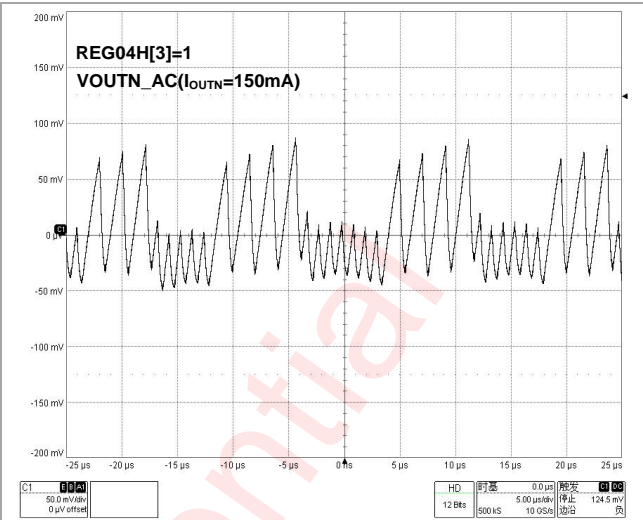
Figure 43 V OUTN Output Voltage Ripple (170mA Mode)
