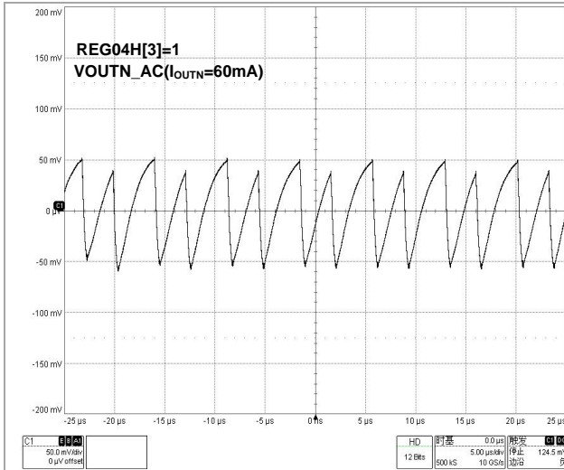
Figure 42 V OUTN Output Voltage Ripple (170mA Mode)
