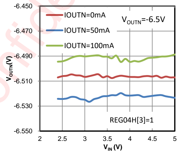
Figure 21 Line Regulation (100mA Mode)
