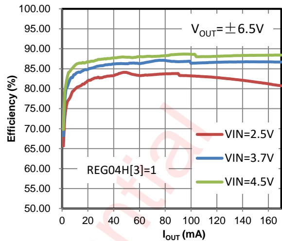
Figure 16 Efficiency (170mA Mode)
