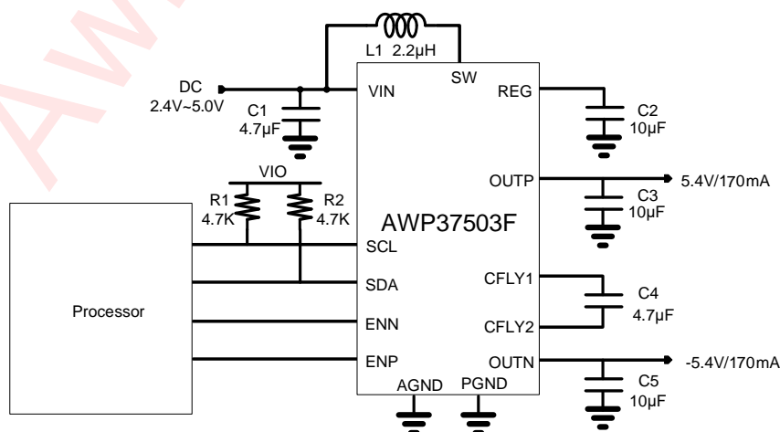
Figure 1 Typical Application Circuit of AWP37503F
