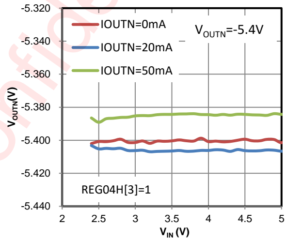
Figure 15 Line Regulation (50mA Mode)
