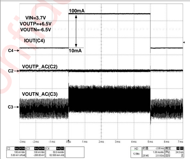
Figure 45 Load Transient (100mA Mode)
