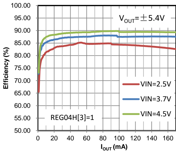
Figure 15 Efficiency (170mA Mode)
