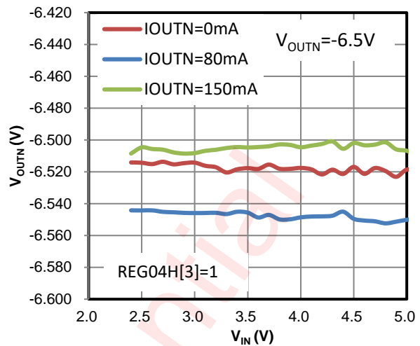
Figure 25 Line Regulation (170mA Mode)
