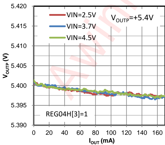
Figure 43 Load Regulation (170mA Mode)
