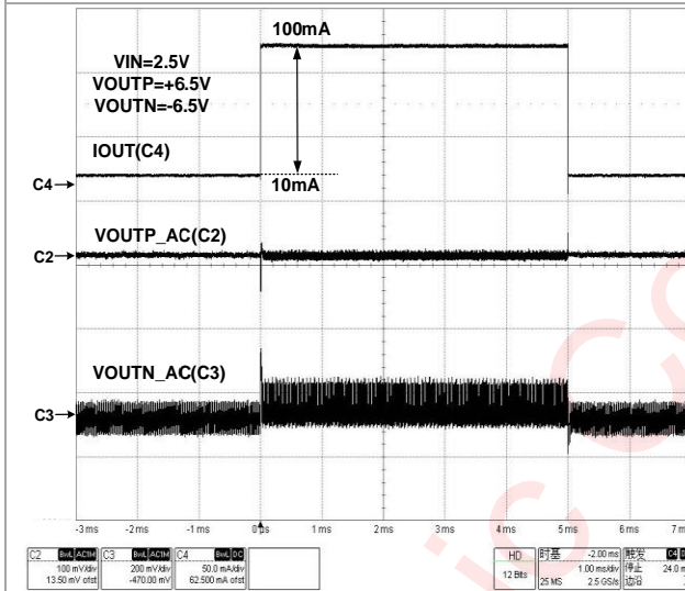
Figure 44 Load Transient (100mA Mode)
