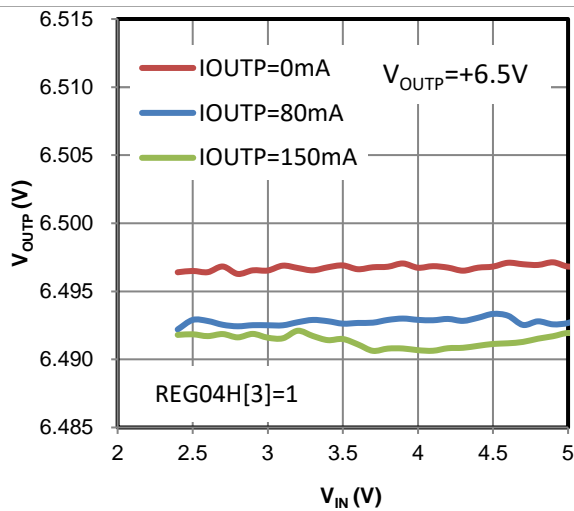
Figure 24 Line Regulation (170mA Mode)
