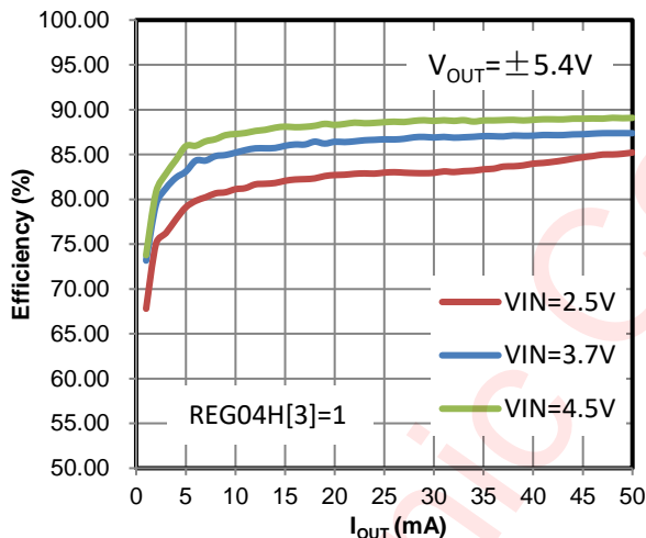
Figure 8 Efficiency (50mA Mode)
