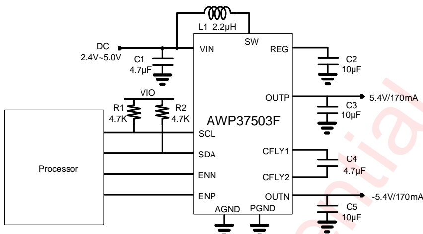
Figure 4 AWP37503F Application Circuit
