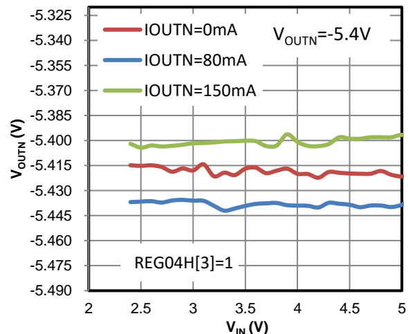
Figure 23 Line Regulation (170mA Mode)
