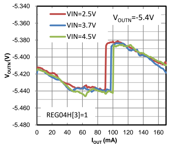
Figure 44 Load Regulation (170mA Mode)
