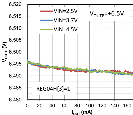
Figure 45 Load Regulation (170mA Mode)
