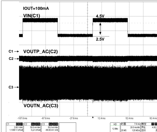
Figure 48 Line Transient (100mA Mode)
