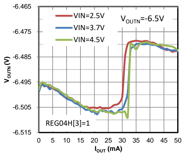
Figure 29 Load Regulation (50mA Mode)
