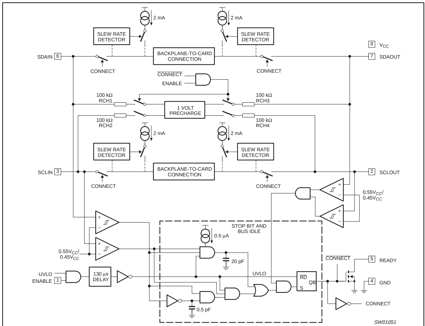
Figure 3. Block diagram
