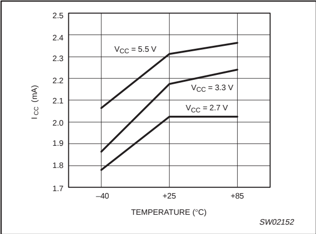
Figure 10. I CC versus Temperature
