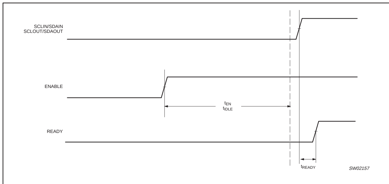
Figure 16. t_{READY} delay that can occur after t_{EN} and t_{IDLE}
