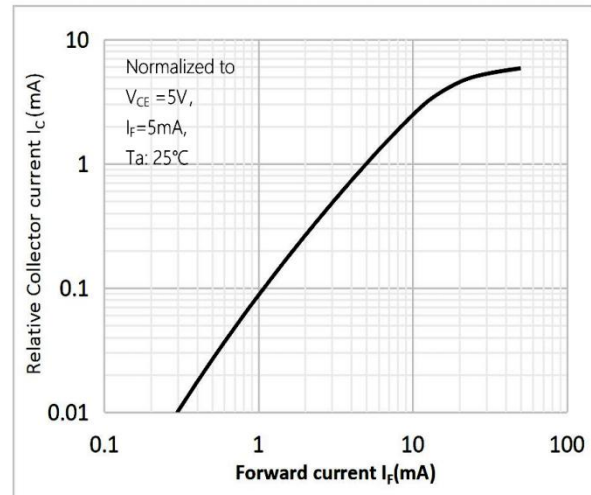
Fig.4 Relative Collector Current vs Forward Current
