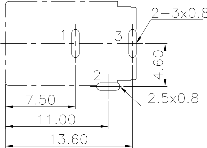
PCB HOLES(TOP VIEW) GENERAL TOLERANCE:±0.05mm
