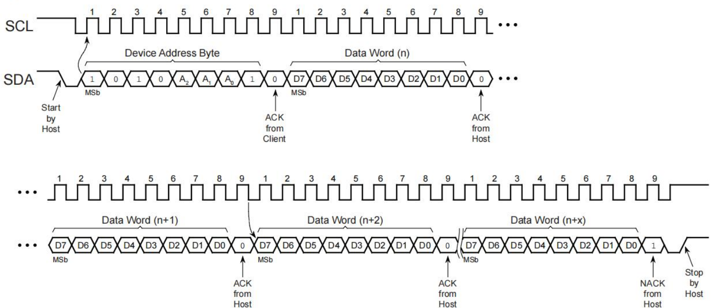
Figure 8-3. Sequential Read
