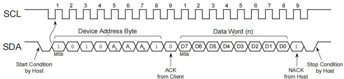
Figure 8-1. Current Address Read
