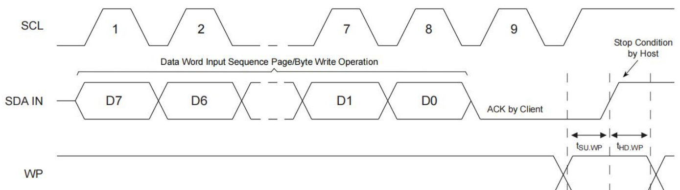
Figure 7-5. Write-Protect Setup and Hold Timing
