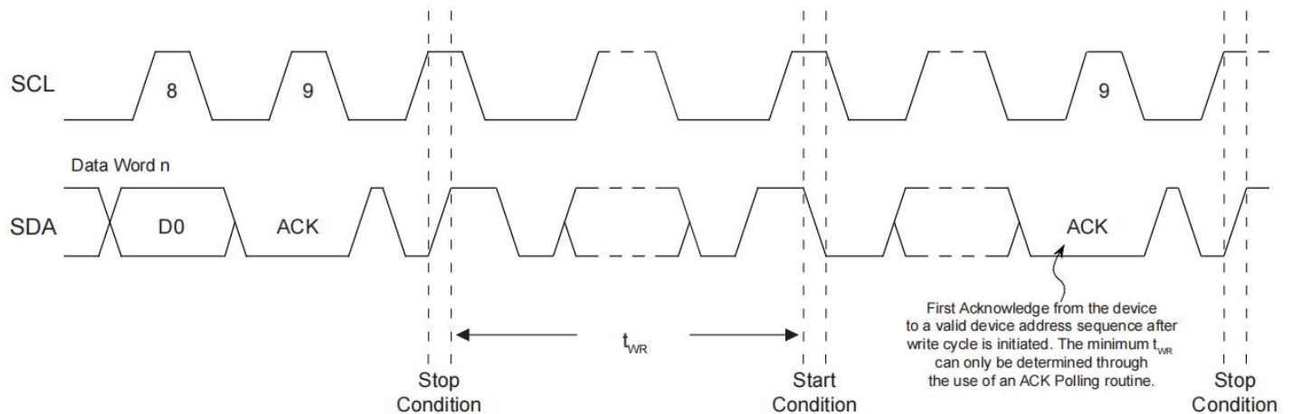
Figure 7-4. Write Cycle Timing
