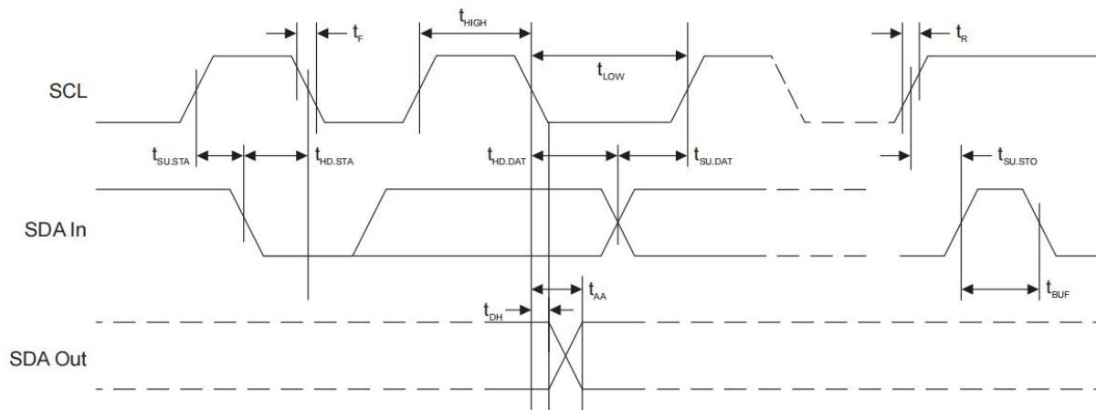
Figure 4-1. Bus Timing
