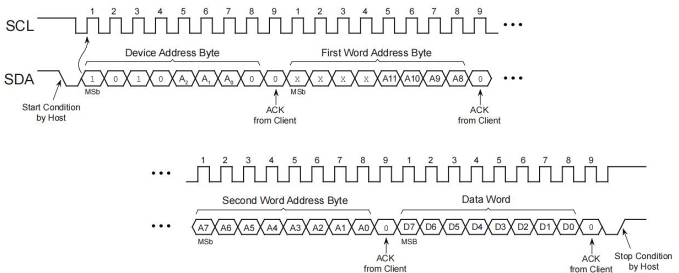
Figure 7-1. Byte Write
