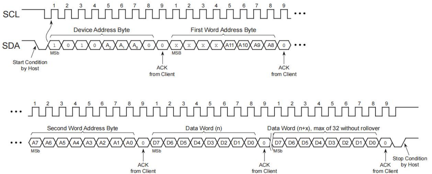
Figure 7-2. Page Write
