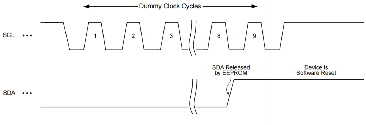
Figure 5-2. Software Reset
