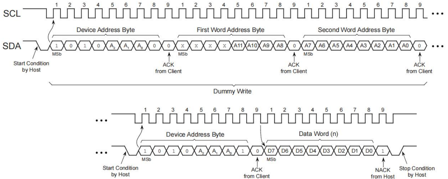
Figure 8-2. Random Read
