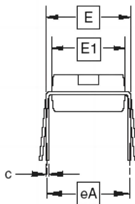
End View
