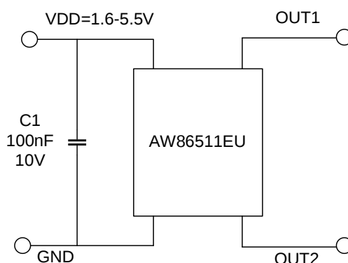
Figure 1 Typical Application Circuit of AW86511EU
