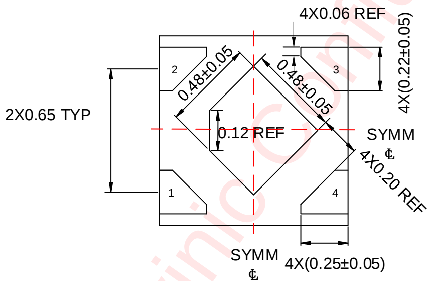
Bottom View
