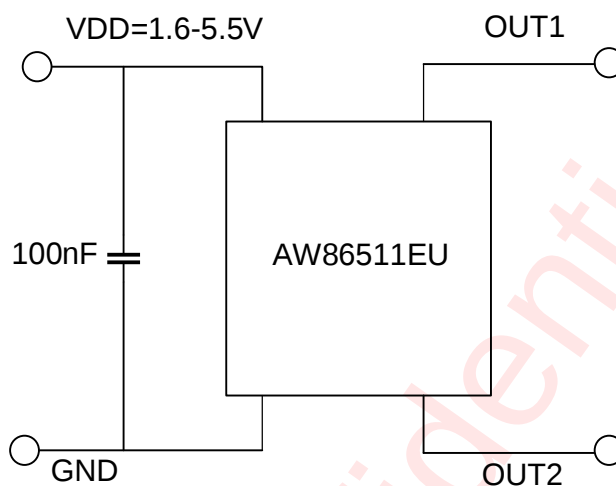
Figure 6 The Application Circuit of AW86511EU
