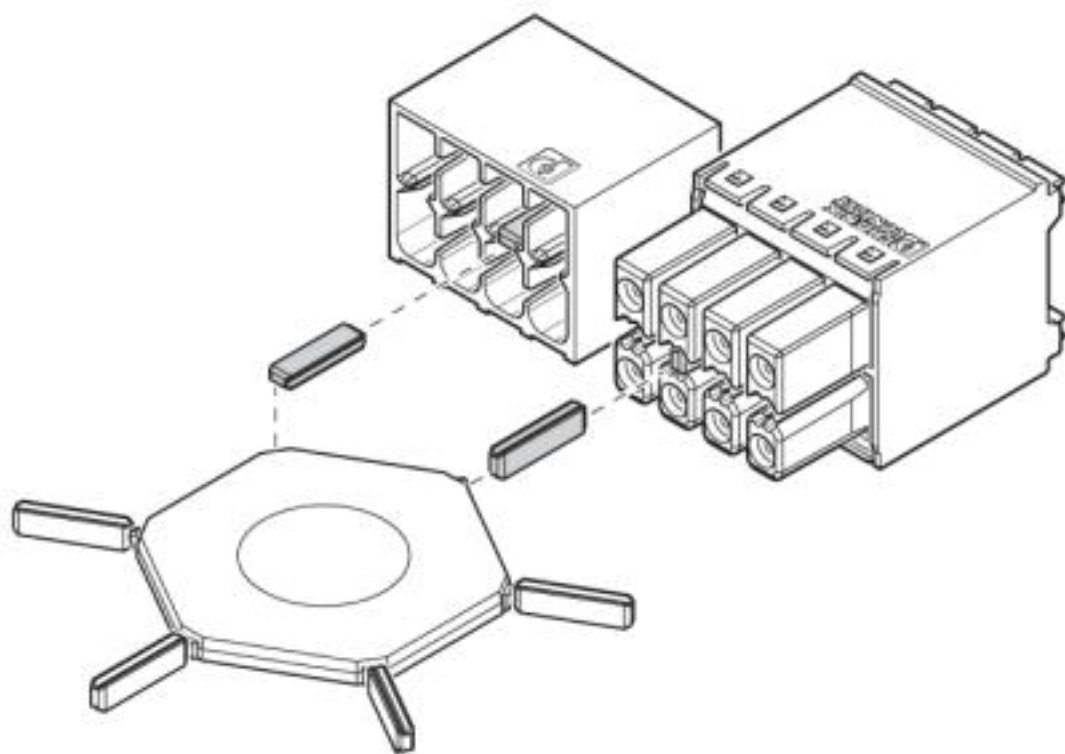
Schematic diagram
