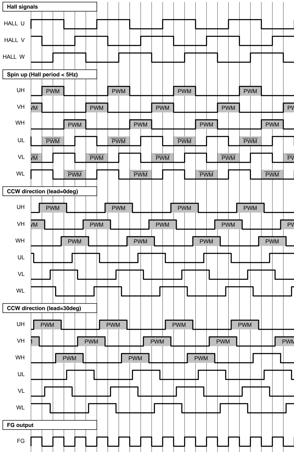
Figure 8. BD62013AFS (Counter clockwise) timing charts
