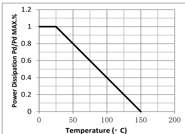
Fig.7 Power Dissipation
