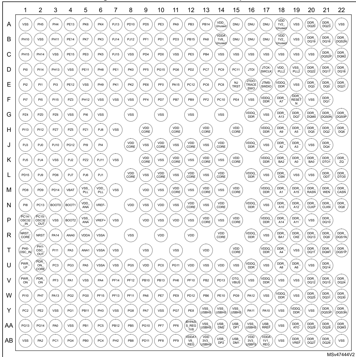
Figure 8. STM32MP153CAA LFBGA448 pinout
