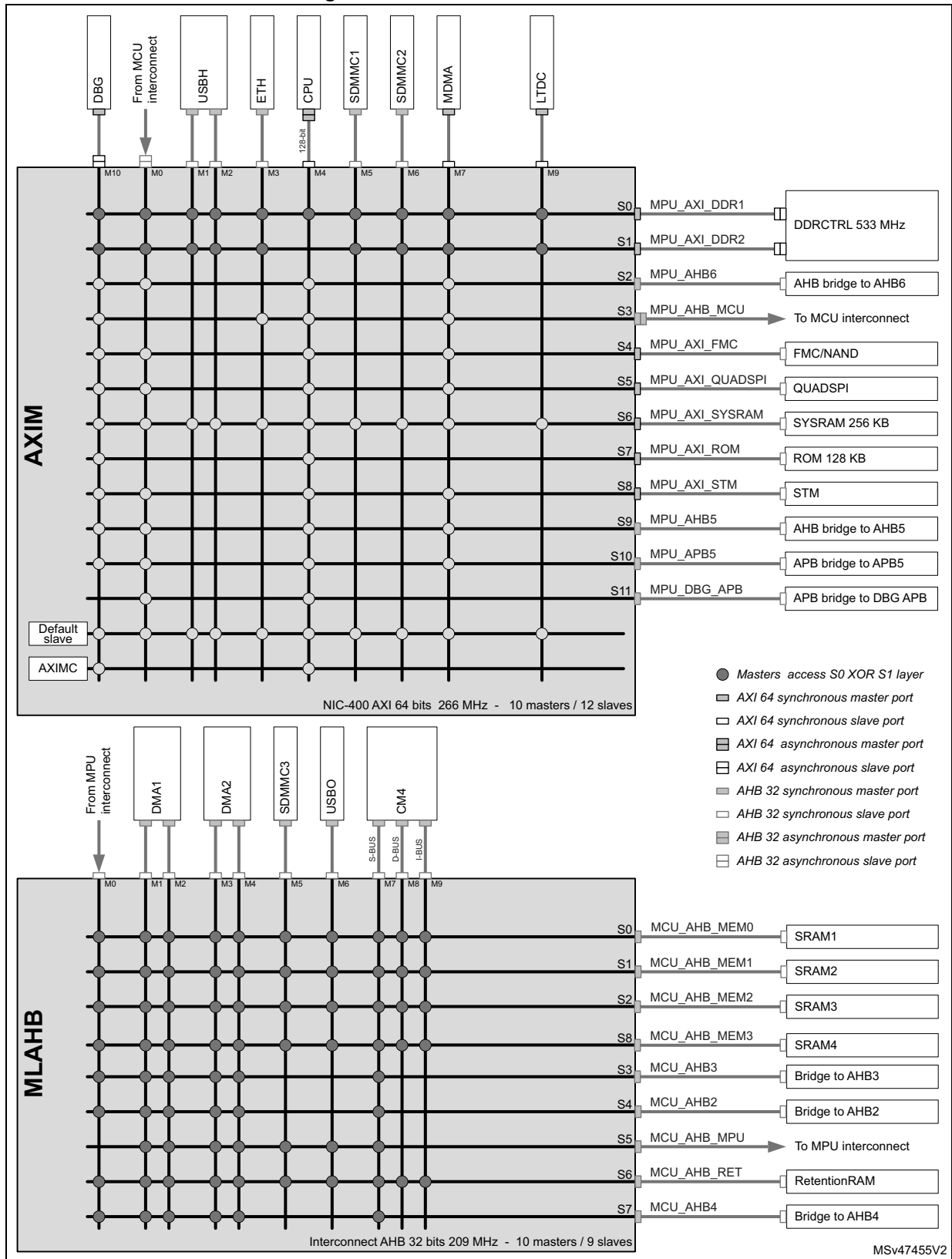
Figure 3. STM32MP153C bus matrix
