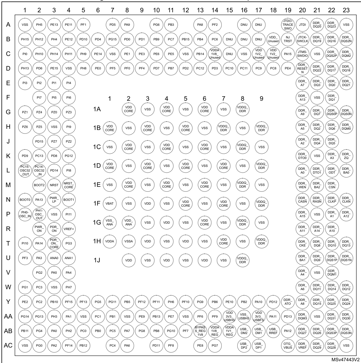
Figure 7. STM32MP153CACxx TFBGA361 pinout
