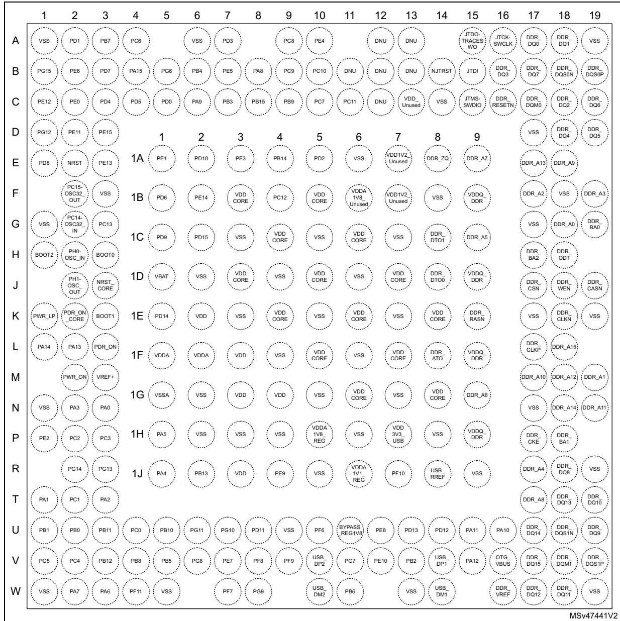
Figure 5. STM32MP153CADxx TFBGA257 pinout
