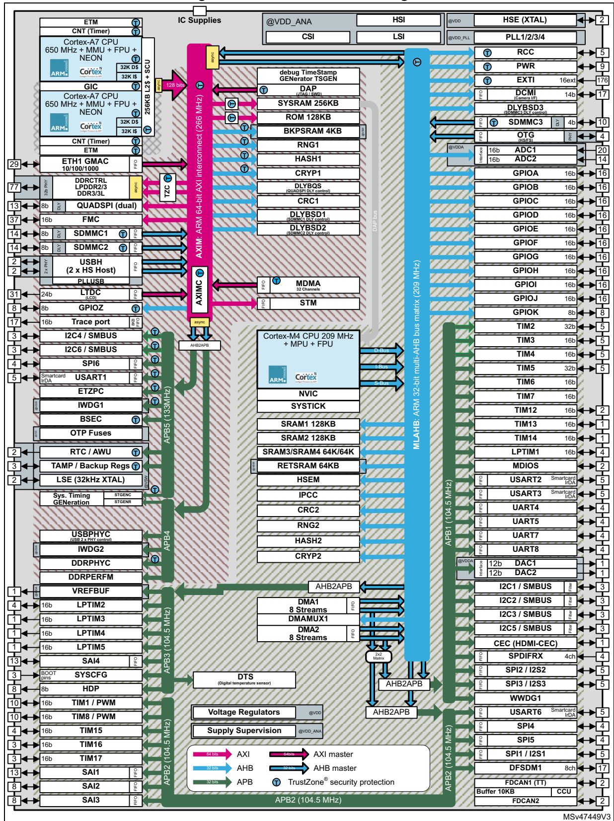
Figure 1. STM32MP153C block diagram
