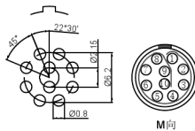
Pcb plate opening size (PCB板开孔尺寸)
