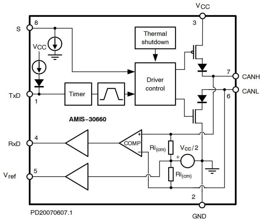
Figure 1. Block Diagram
