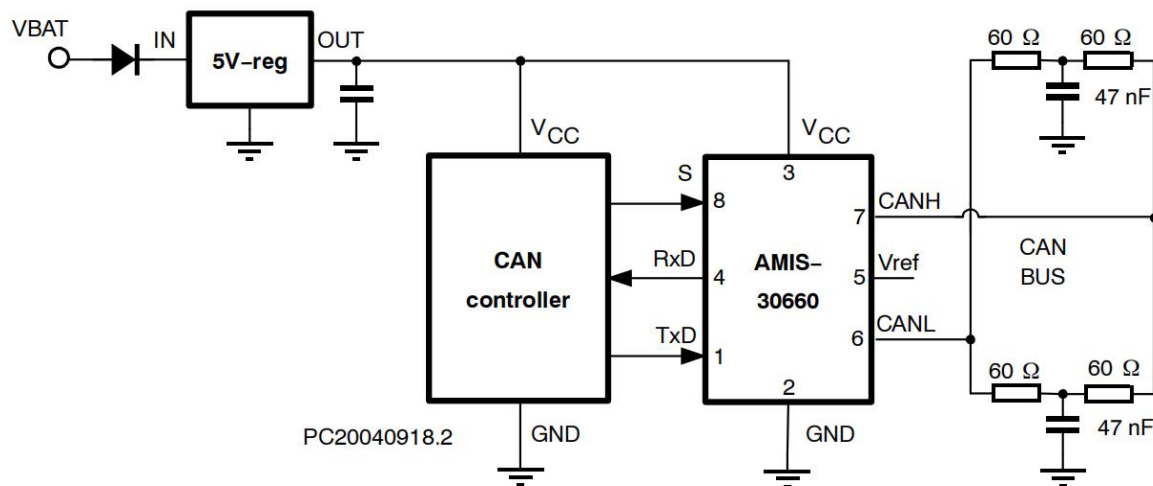
Figure 2. Application Diagram
