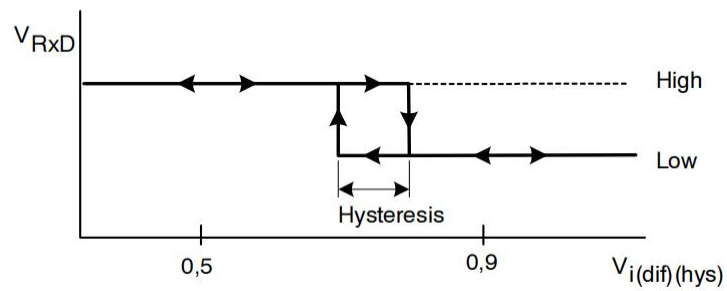
Figure 4. Hysteresis of the Receiver
