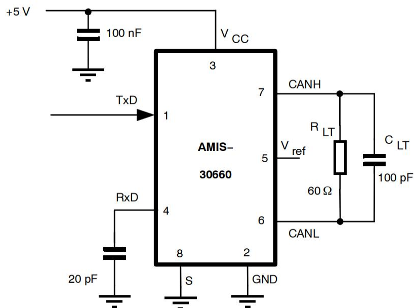
Figure 5. Test Circuit for Timing Characteristics
