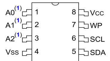
SOIC, TSSOP (Top view)
