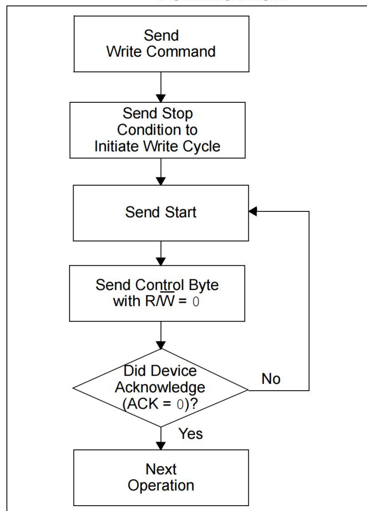
FIGURE 7-1: ACKNOWLEDGE POLLING FLOW
