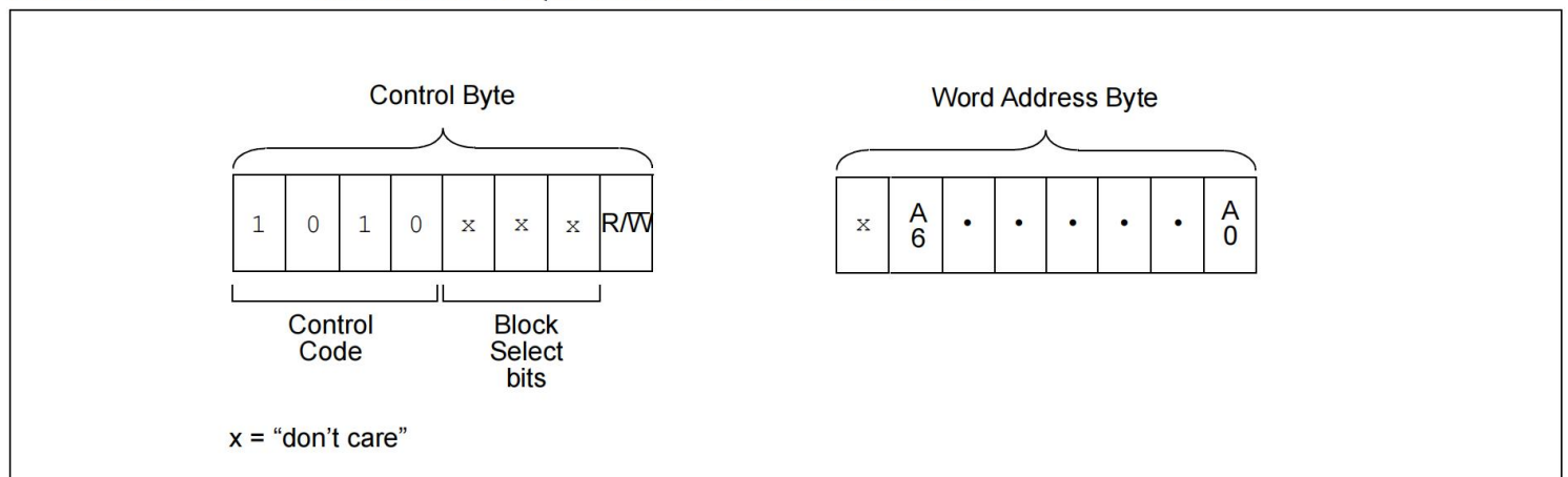
FIGURE 5-2: ADDRESS SEQUENCE BIT ASSIGNMENTS
