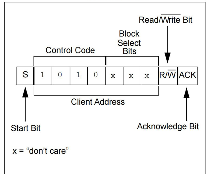
FIGURE 5-1: CONTROL BYTE ALLOCATION
