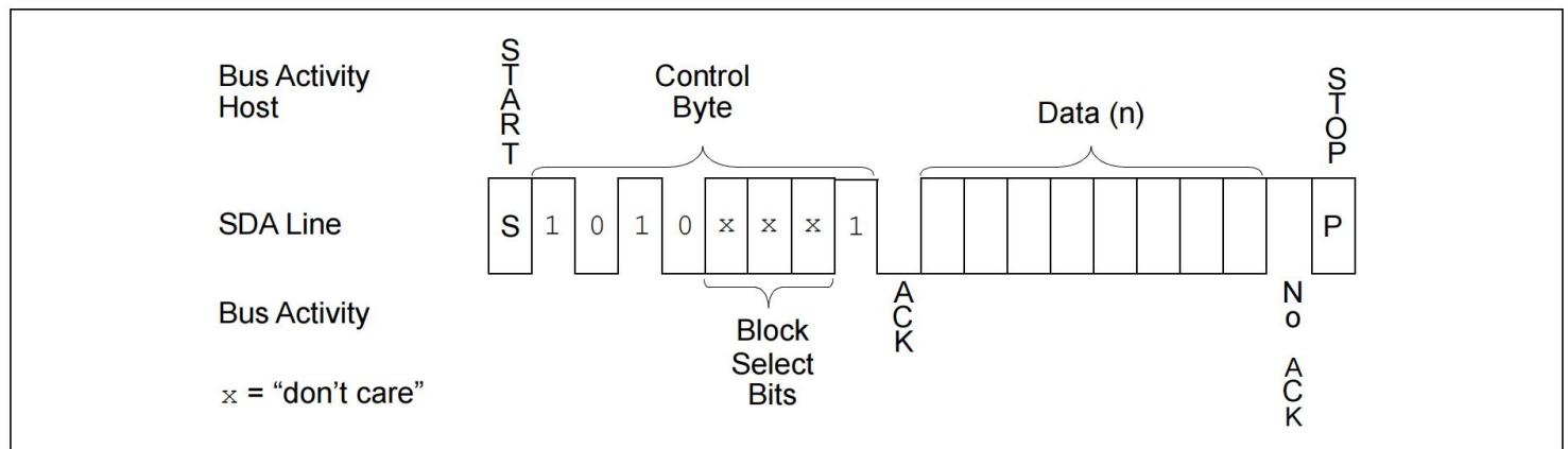
FIGURE 8-1: CURRENT ADDRESS READ
