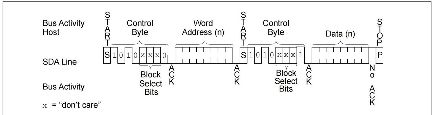
FIGURE 8-2: RANDOM READ
