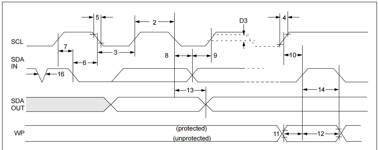
FIGURE 1-1: BUS TIMING DATA
