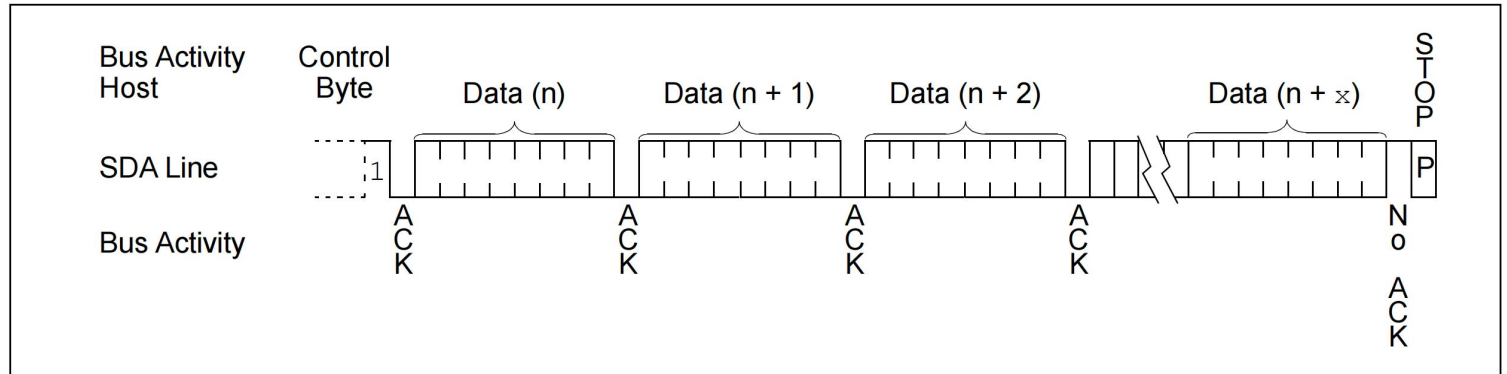
FIGURE 8-3: SEQUENTIAL READ
