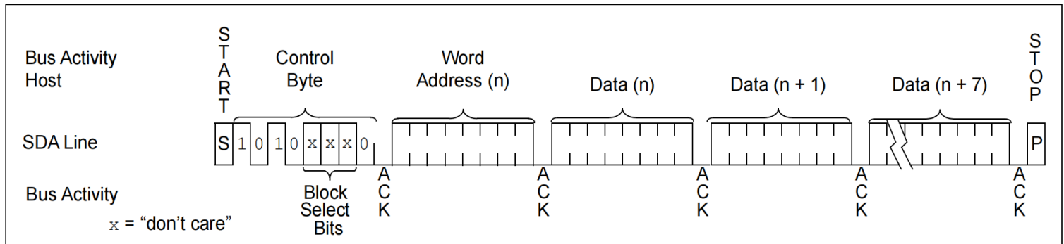
FIGURE 6-2: PAGE WRITE
