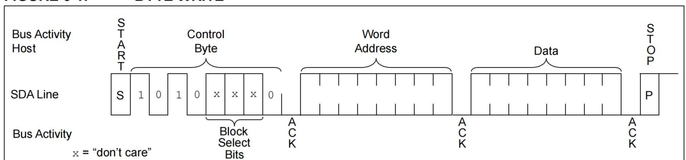
FIGURE 6-1: BYTE WRITE
