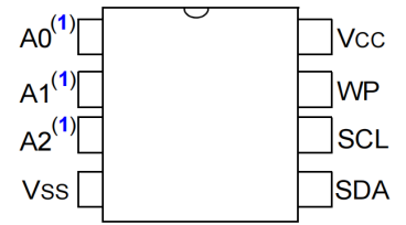
PDIP (Top view)
