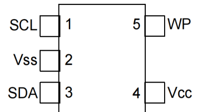
SOT-23 (Top view)
