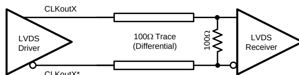
Figure 29. Differential LVDS Operation, DC Coupling, No Biasing by the Receiver
