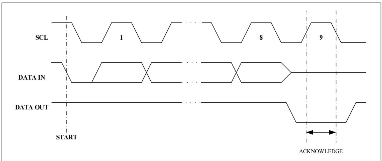
Figure 4. Output Acknowledge
