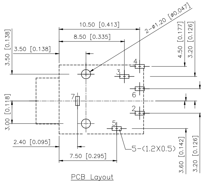
PCB Layout
