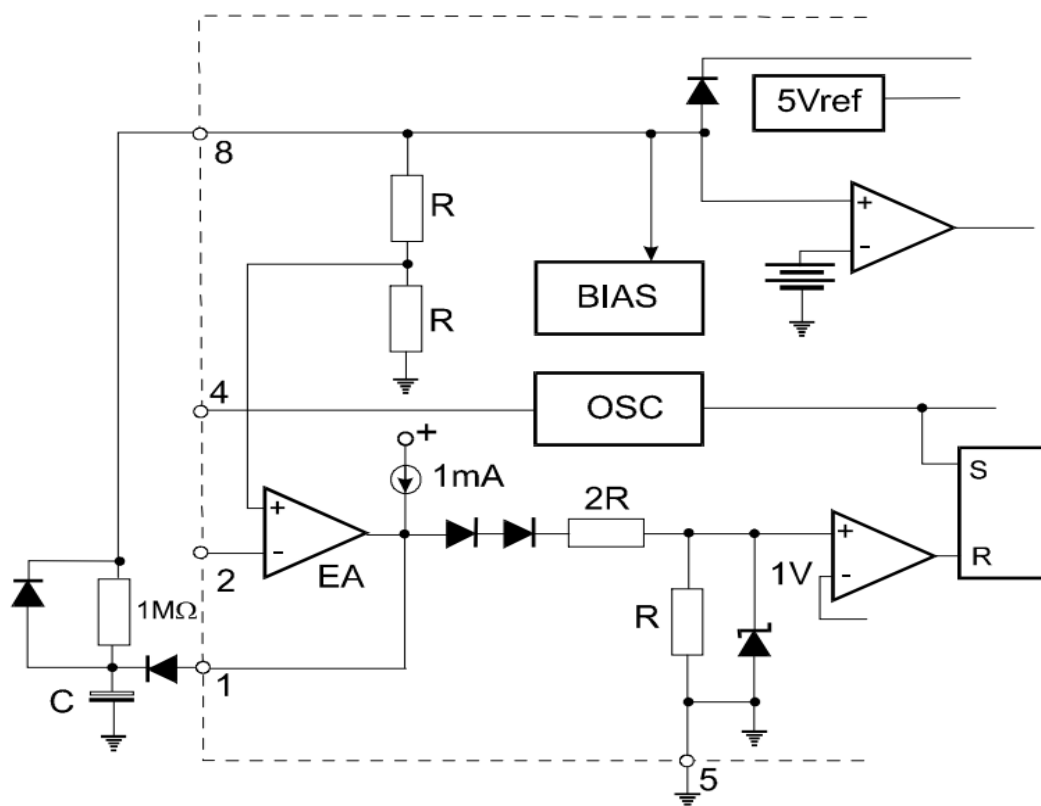
Figure 8. Soft-Start Circuit
