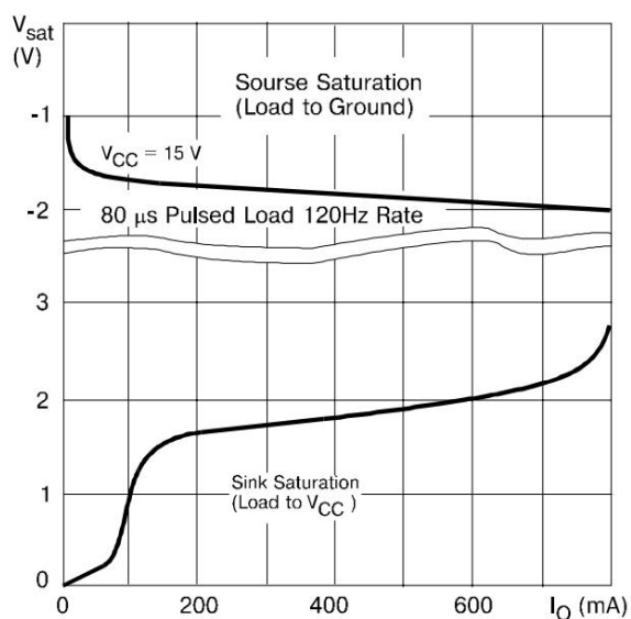
Figure 7. Output Saturation Voltage vs. Load Current T A = 25°C
