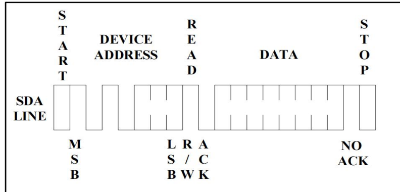
Figure 9. Random Read
